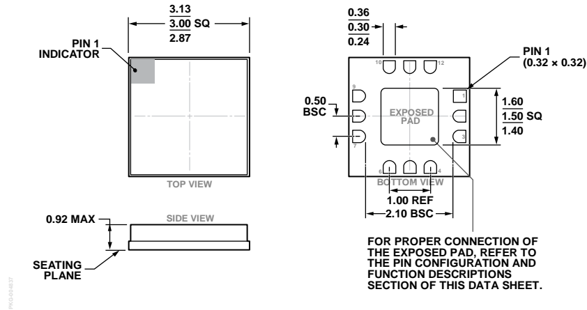
Figure 36. 12-Terminal Ceramic Leadless Chip Carrier [LCC] (E-12-1) Dimensions shown in millimeters
