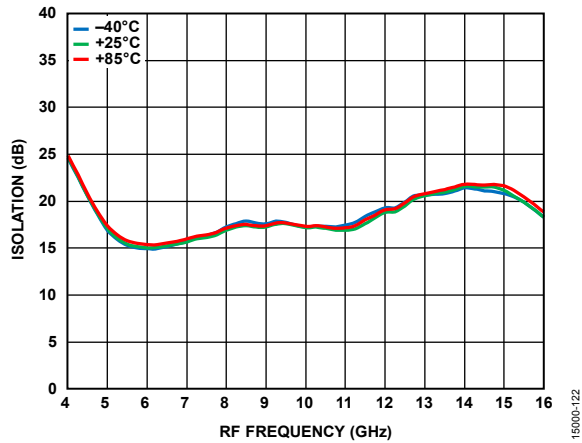
Figure 28. RF to IF Isolation vs. RF Frequency at Various Temperatures, IF = 100 MHz
