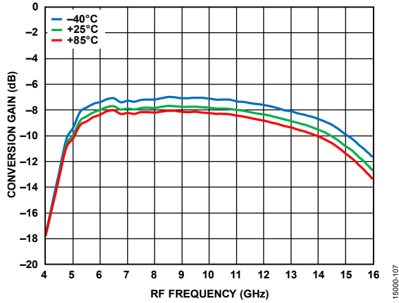
Figure 7. Conversion Gain vs. RF Frequency at Various Temperatures, IF = 100 MHz
