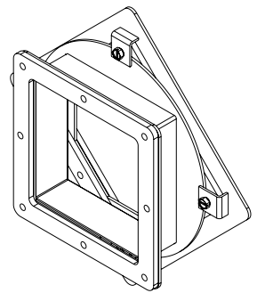
ISOMETRIC VIEW
