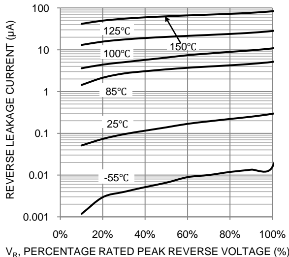
V_R , PERCENTAGE RATED PEAK REVERSE VOLTAGE (%) Fig.5 Typical Reverse Characteristics
