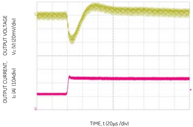
Figure 16. Transient Response to Dynamic Load Change from 50% to 100% at 12V in , C out = 2x47uF+2x330uF, CTune=5600pF & RTune=220Ω
