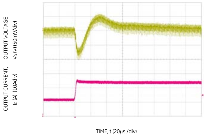
Figure 28. Transient Response to Dynamic Load Change from 50% to 100% at 12V in , C out = 2x47uF+1x330uF, CTune=2700pF & RTune=300Ω
