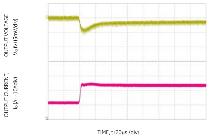
Figure 4. Transient Response to Dynamic Load Change from 50% to 100% at 12Vin, Cout=1x47uF+11x330uF, CTune=47nF, RTune=180Ω
