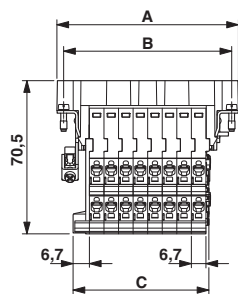
Dimensioned drawing
