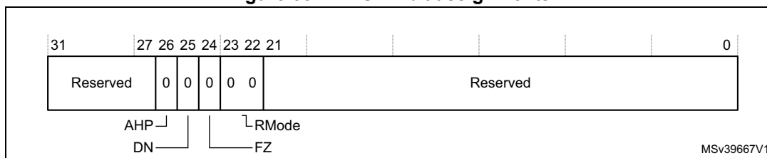
Figure 58. FPDSCR bit assignments
