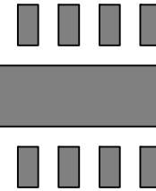
(c) Copper Area = 30mm 2 , \theta_{JA} = 54^\circ\text{C/W}
