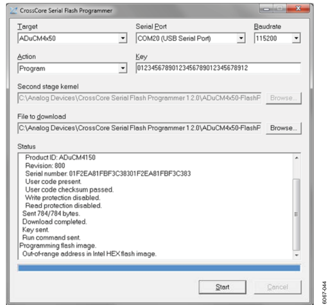
Figure 32. User Application Code Being Written by the SSL to User Flash Memory via the CCSFP
