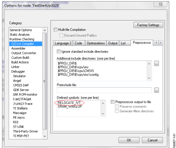
Figure 24. IAR C/C++ Compiler Options—RELOCATE_IVT Directive in the Defined Symbols Textbox
