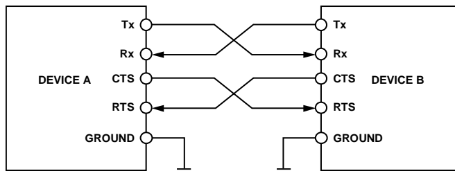
Figure 40. Hardware Flow Control
