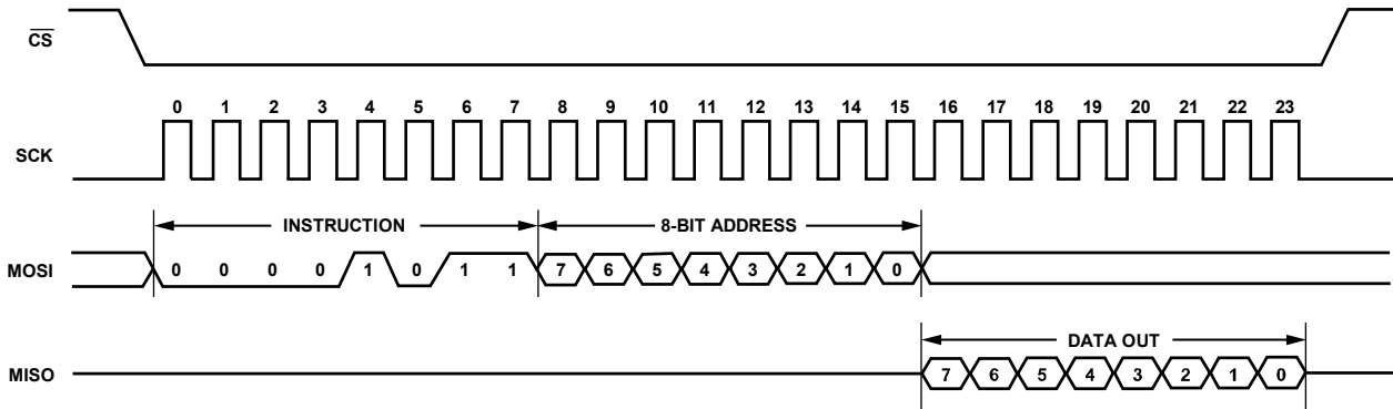
Figure 49. Read Command Mode
