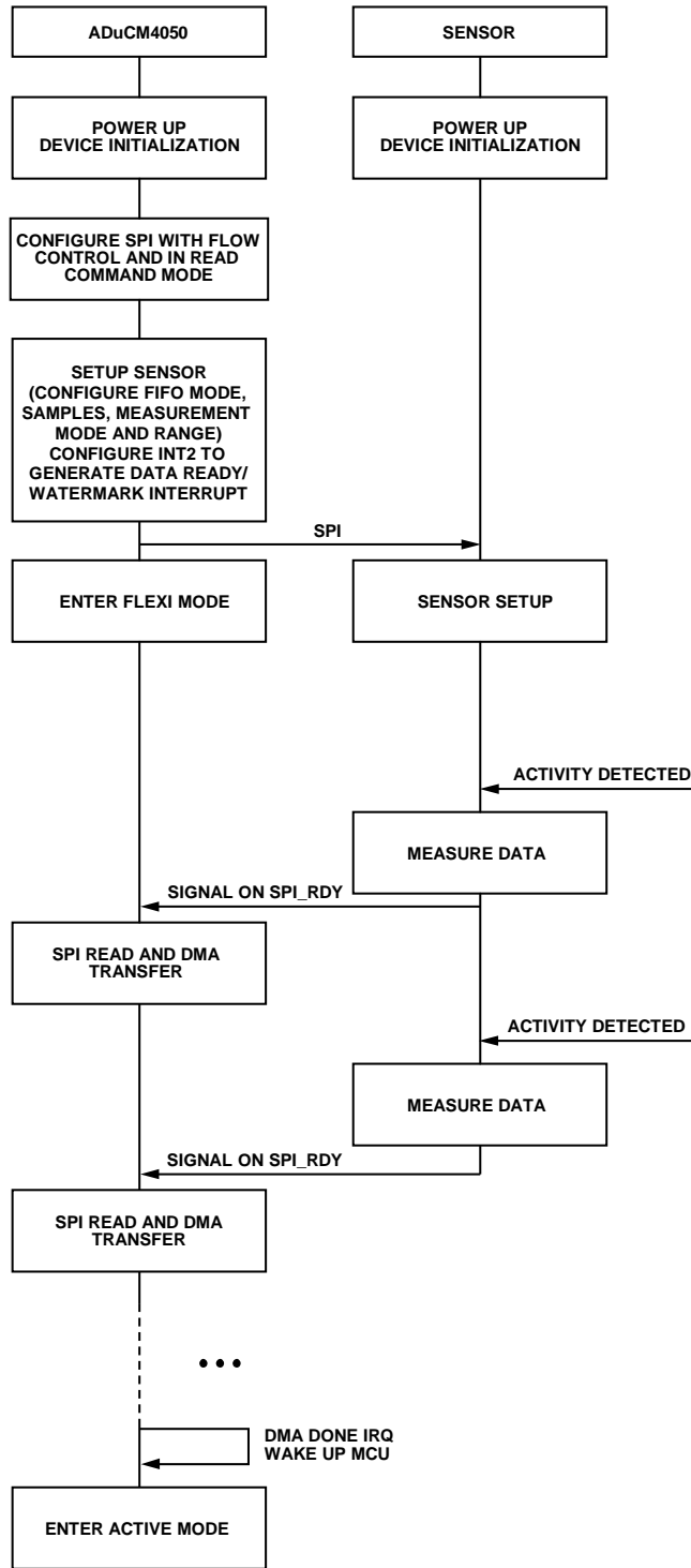
Figure 56. Application Flowchart
