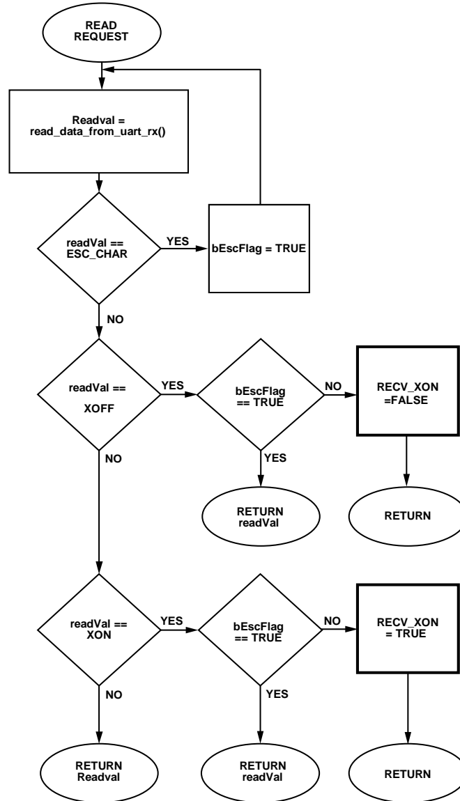
Figure 44. Flowchart of the Control Signals in the ISR Being Processed
