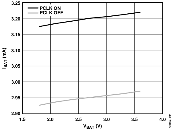
Figure 15. Impact of Peripheral Clock Gating on Active Mode Power Consumption
