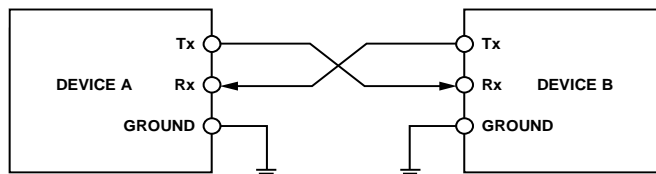
Figure 39. Software Flow Control Block Diagram
