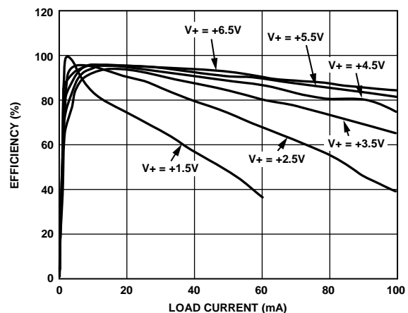
Figure 38. ADM660/ADM8660 Efficiency vs. Load Current
