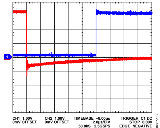
Figure 22. Normal Wake Up from Hibernate Mode Response
