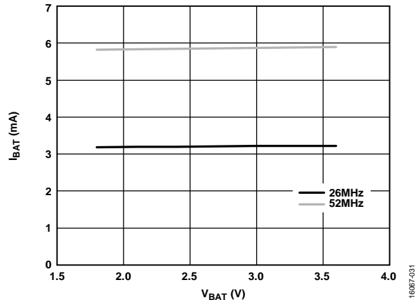
Figure 14. Impact of Core Clock Frequency on Active Mode Power Consumption with the PLL
