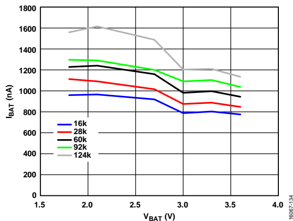
Figure 18. Current on the V BAT Supply Pin (I BAT ) for Various Retained SRAM Values
