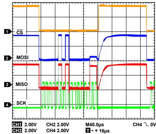
Figure 51. Sector Erase—Single CS Frame Capture
