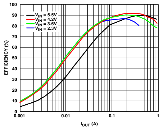
Figure 37. ADP2503/ADP2504 Efficiency vs. Output Current ( I_{OUT} )
