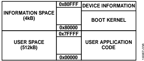
Figure 26. Flash Information Memory Space
