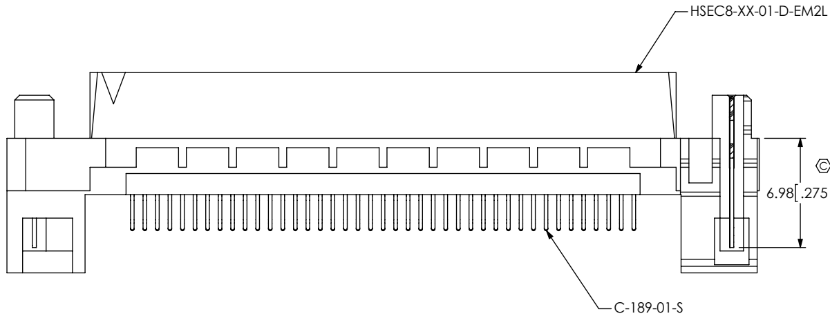
SECTION "E"-"E"
