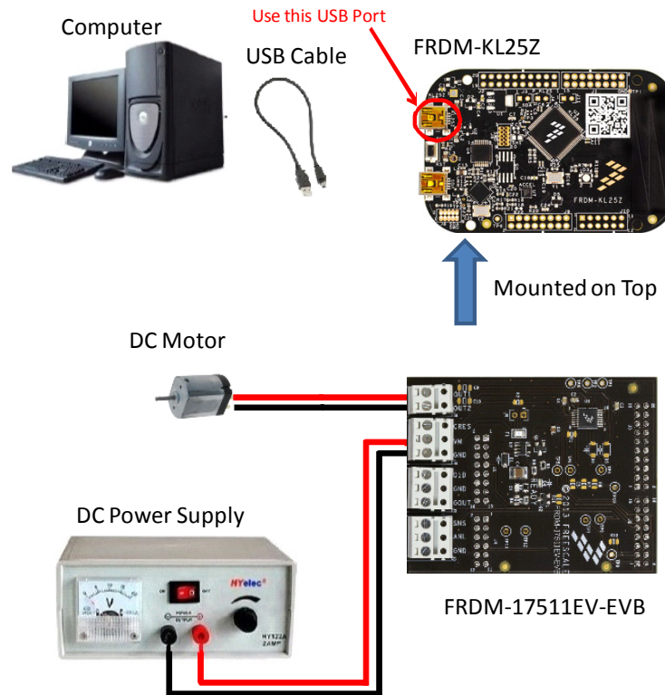
Figure 5. FRDM-17511EV-EVB plus FRDM-KL25Z Board Setup
