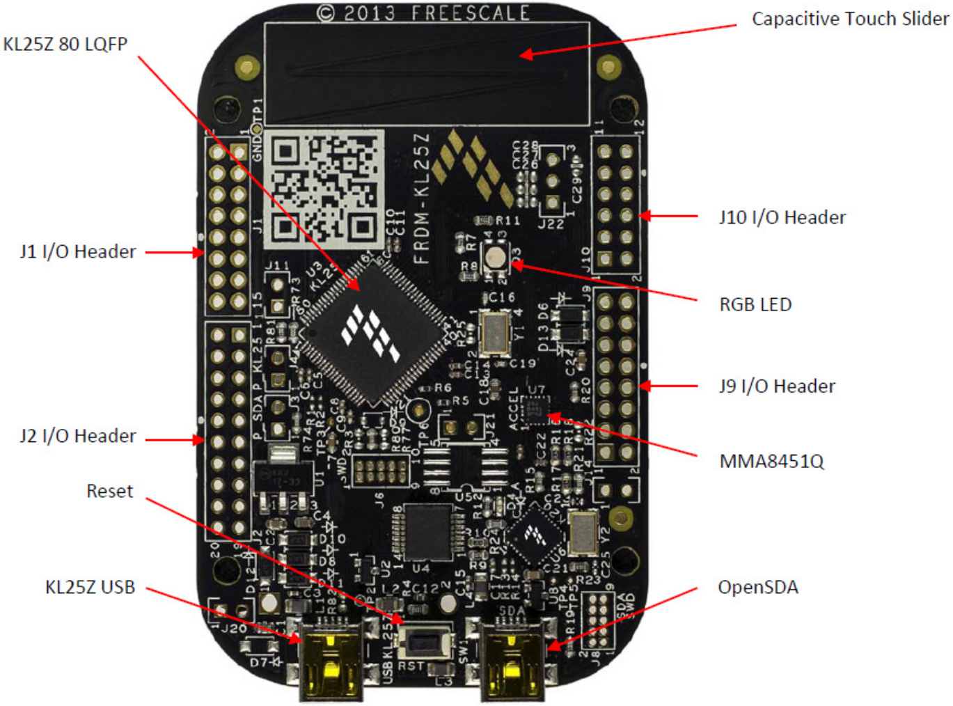
Figure 3. FRDM-KL25Z
