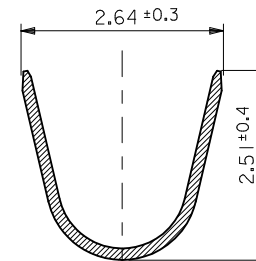
SECT. Y-Y
