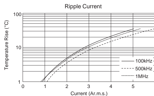
[Example of Temperature Rise (Heat Generation) in Chip Monolithic Ceramic Capacitors in Contrast to Ripple Current]
