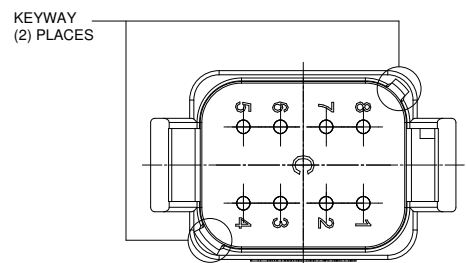
P/N AT04-08PC-BMXX KEY-C CONFIGURATION COLOR: GREEN
