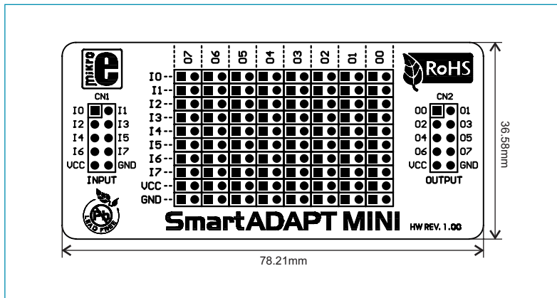
Figure 5: Dimensions of the Smart ADAPT MINI additional board
