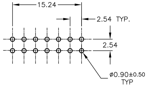
RECOMMENDED P.C.B. LAYOU
