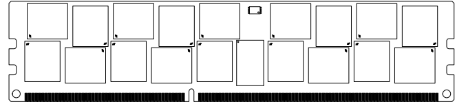
Figure 1: 240-Pin RDIMM (MO-269 R/C H0)
