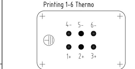
Contact arrangement
