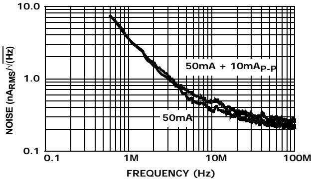
FIGURE 9. I_{BLUE} NOISE vs FREQUENCY
