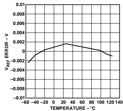
Figure 19. Typical Voltage Reference Error vs. Temperature
