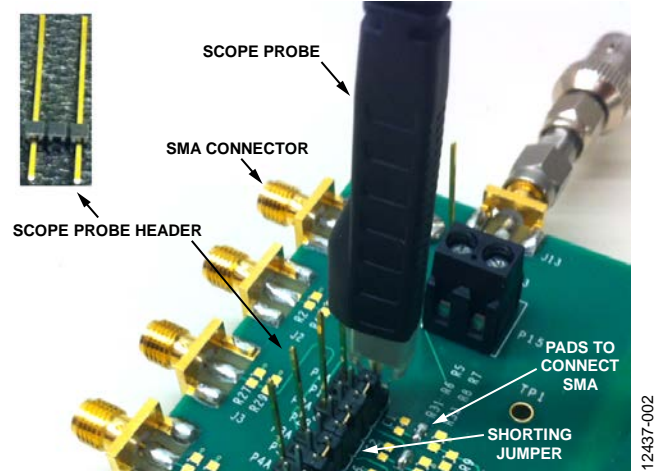
Figure 2. Optional Components
