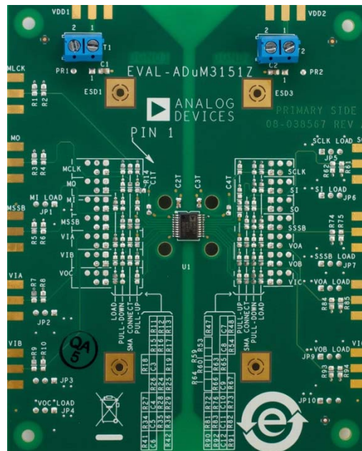
Figure 1. EVAL-ADuM3151Z Evaluation Board
