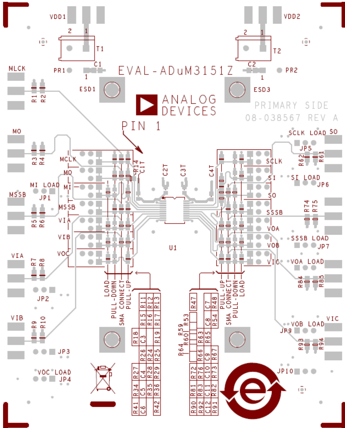
Figure 5. Top Side Layout
