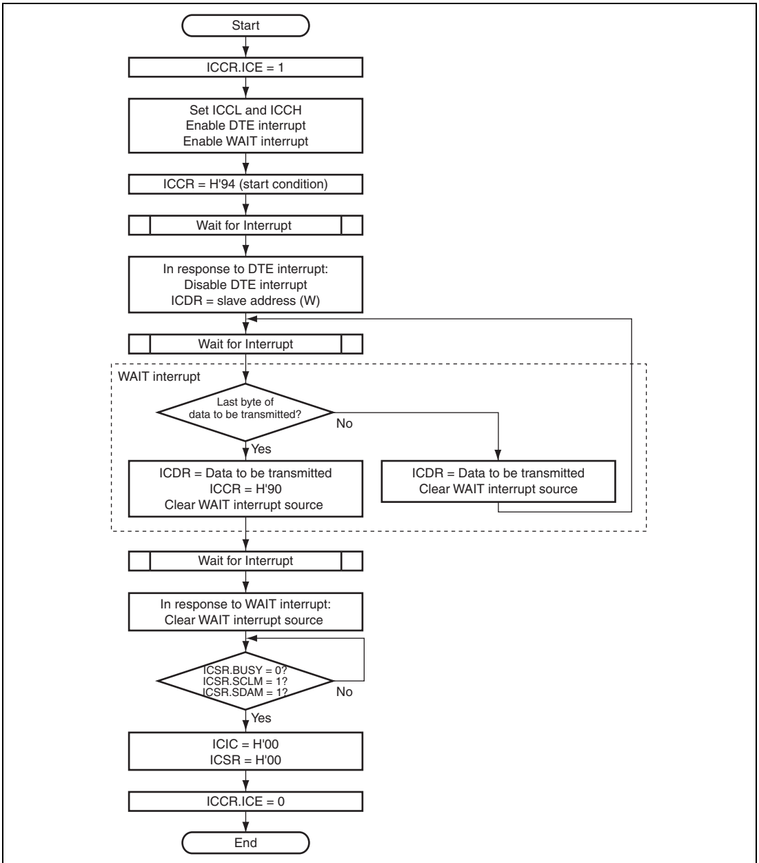
Figure 32.16 Example Flow of Software for Transmission with Use of Wait Interrupt
