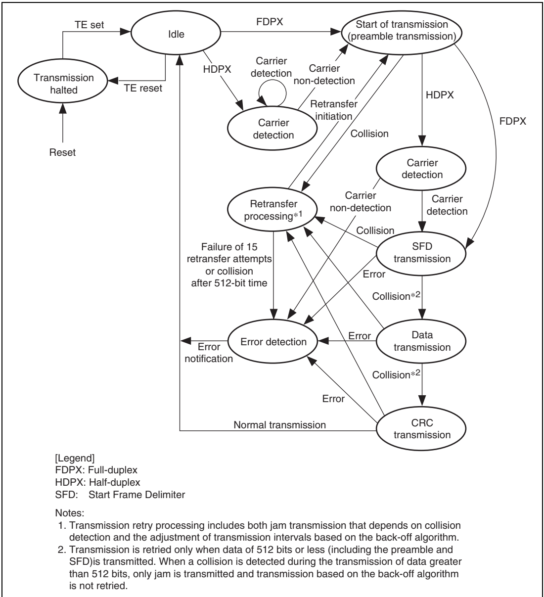
Figure 47.7 EtherC Transmitter State Transitions
