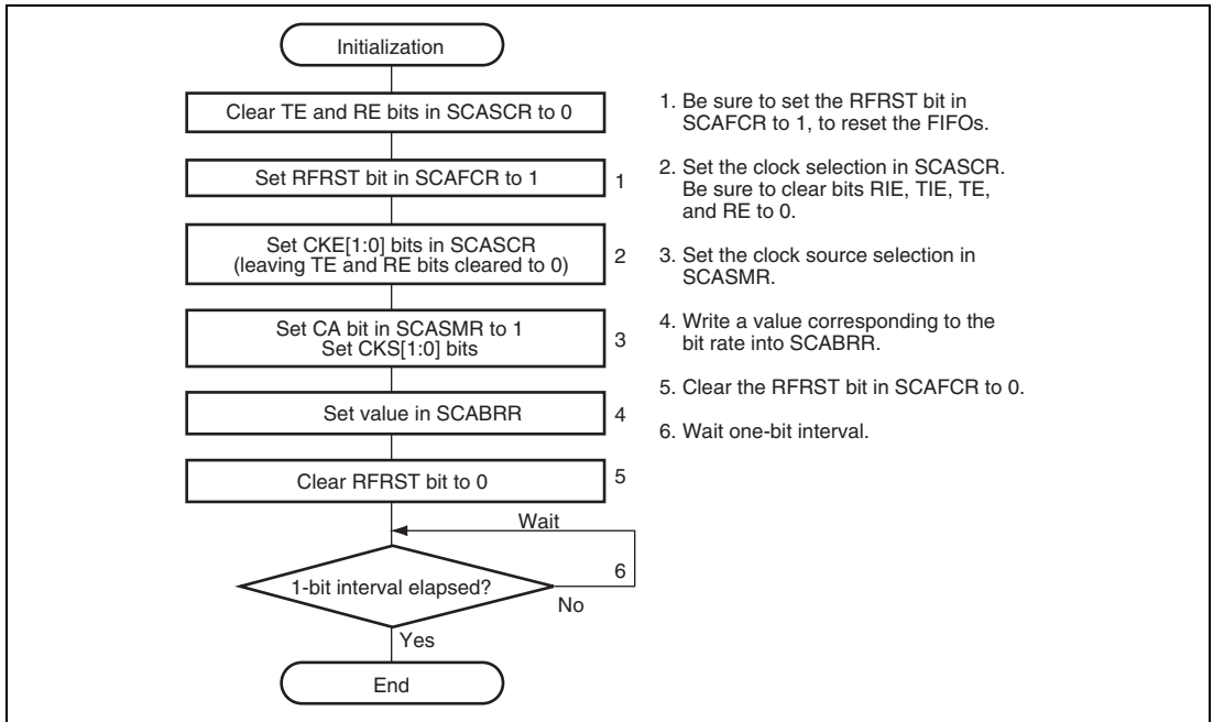
Figure 27.14 Sample SCIFA Initialization Flowchart (2) (Reception)
