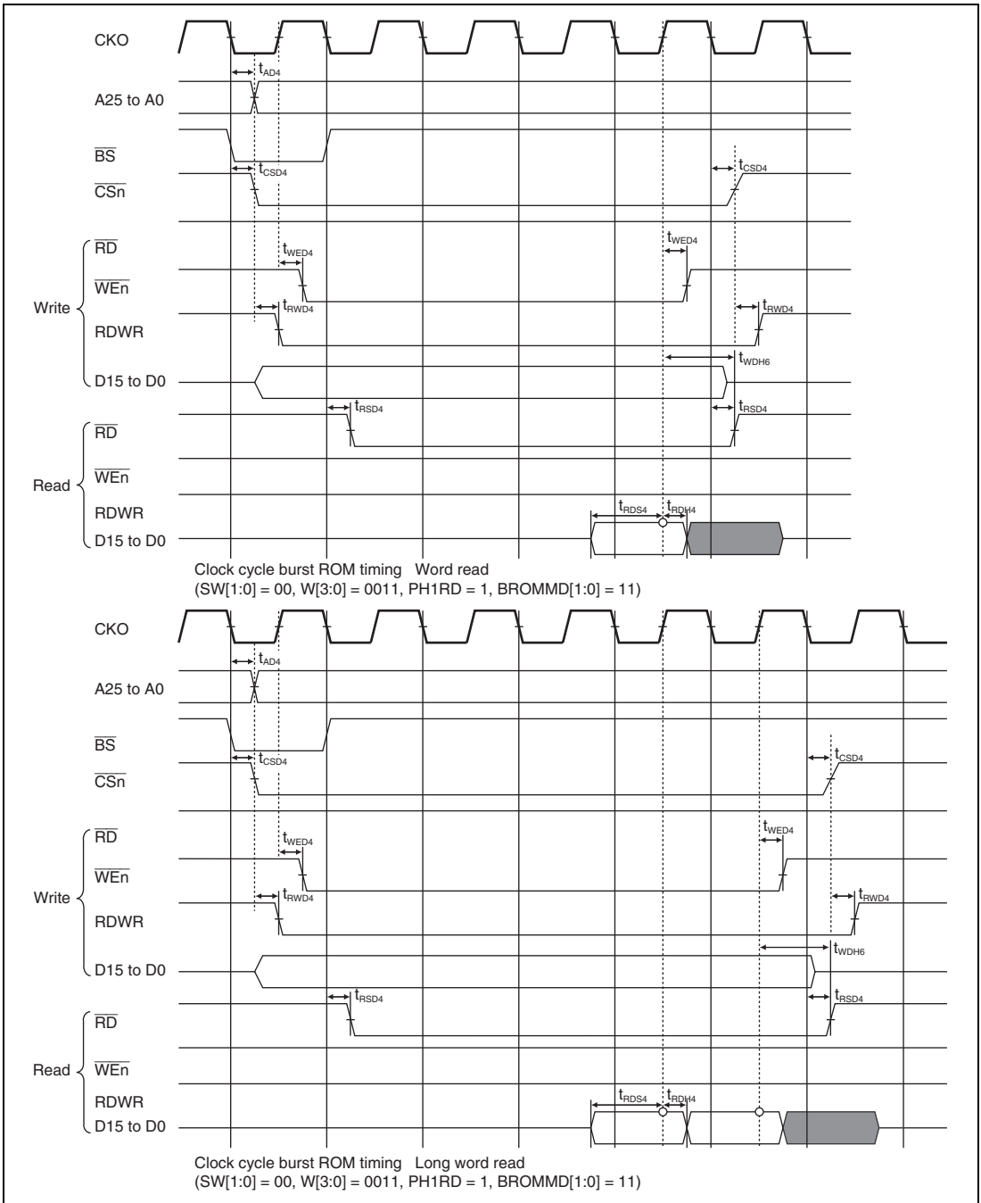
Figure 52.20 Clock-synchronous Burst ROM Timing
