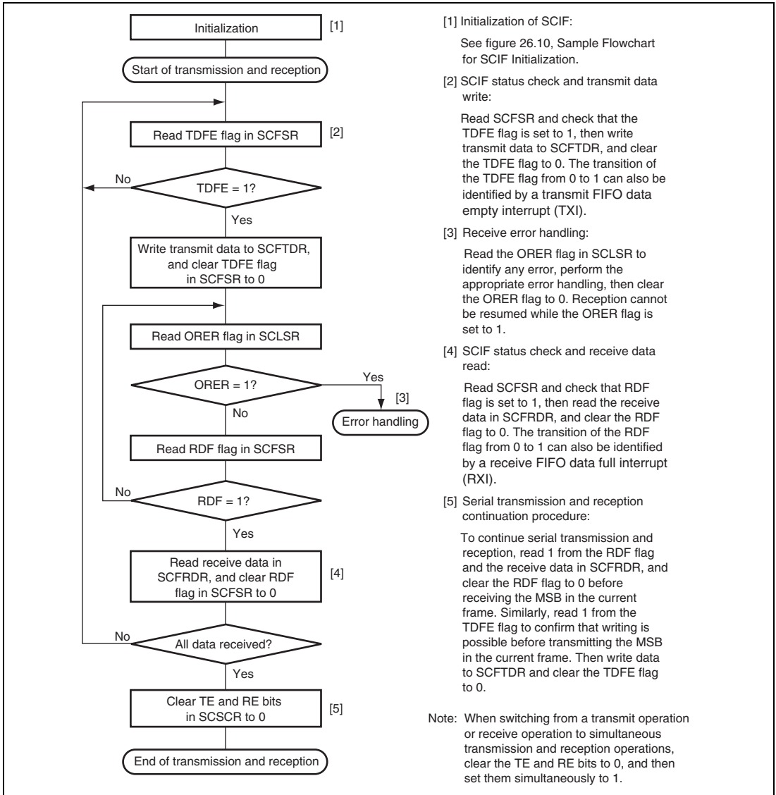
Figure 26.16 Sample Flowchart for Transmitting/Receiving Serial Data
