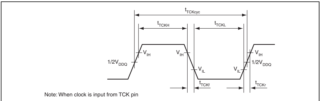
Figure 52.89 TCK Input Timing
