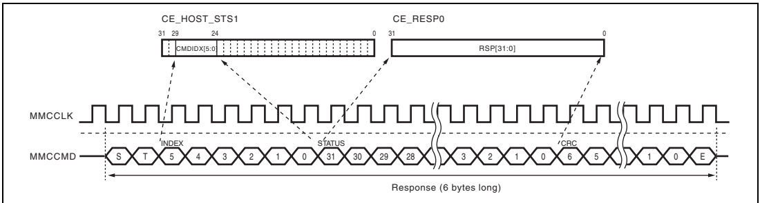
Figure 23.3 Format of 6-Byte Response
