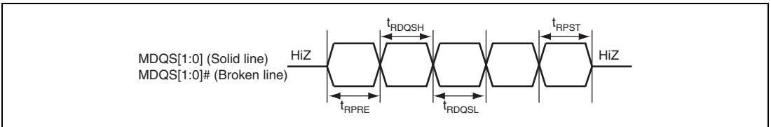
Figure 52.28 DQS Input Waveform Limitation (Read)
