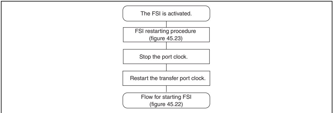
Figure 45.27 Procedures for Stopping and Restarting All Clocks (Software Reset)
