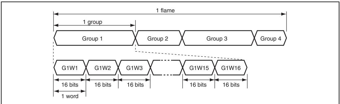
Figure 25.2 Multiple Channel Structure
