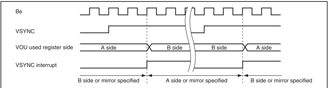
Figure 40.11 Timing of Interrupt and Specifying Timing
