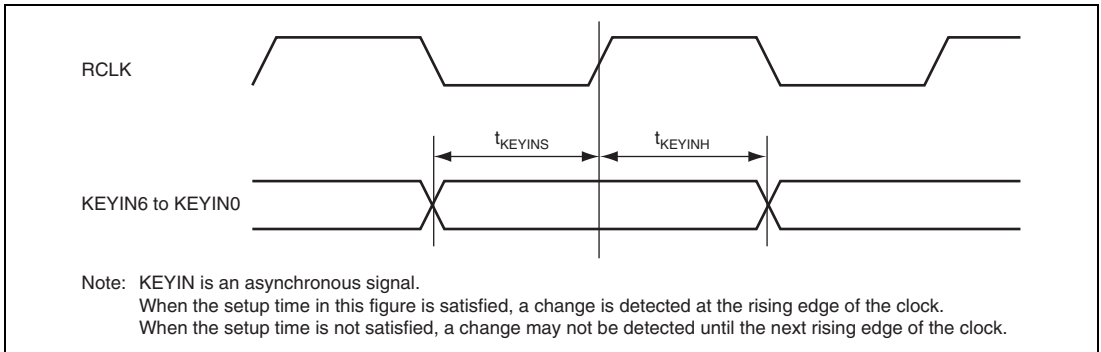
Figure 52.56 KEYIN Input Timing
