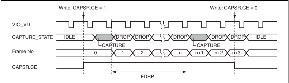
Figure 34.9 Setting of FDRP Bits and Frame Drop Timing
