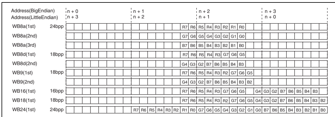
Figure 39.17 Write-Back Data Format
