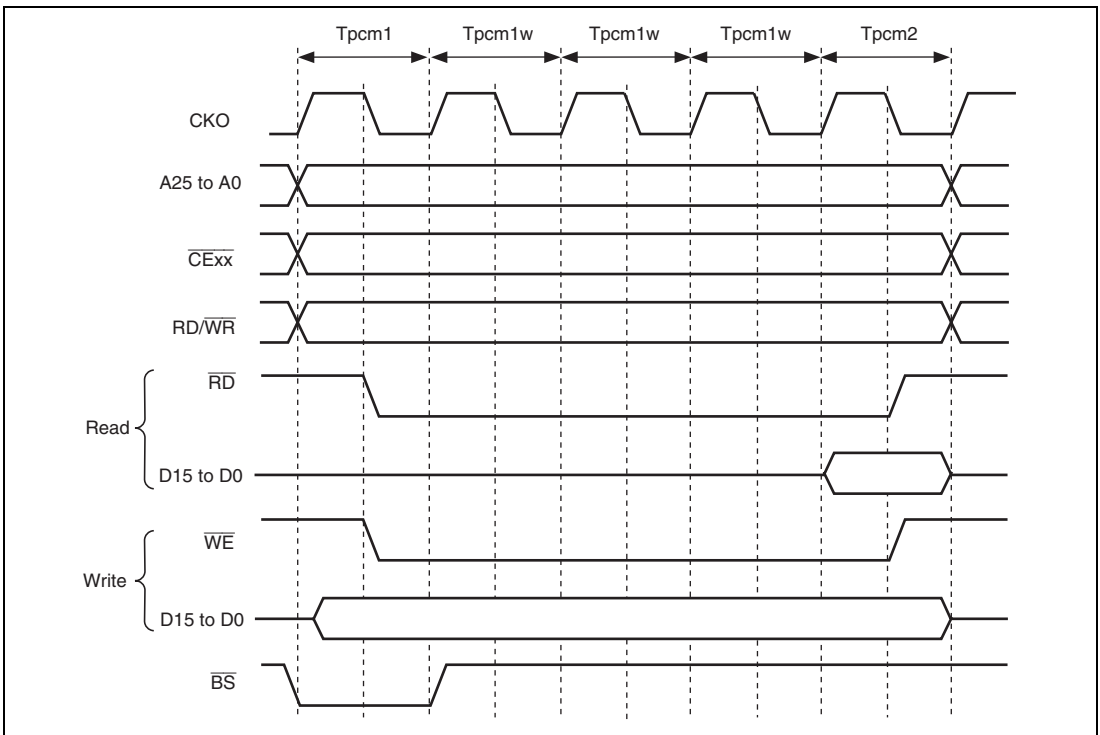
Figure 14.18 Basic Timing of PCMCIA Memory Card Interface
