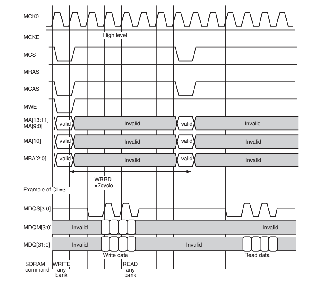
Figure 15.18 WRITE-READ Minimum Time
