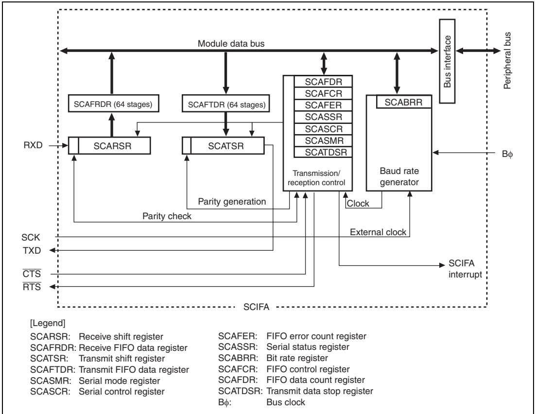
Figure 27.1 Block Diagram of SCIFA
