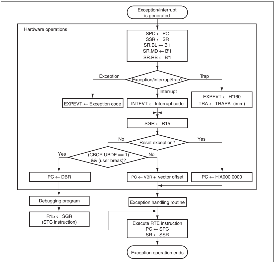
Figure 49.2 Flowchart of User Break Debugging Support Function
