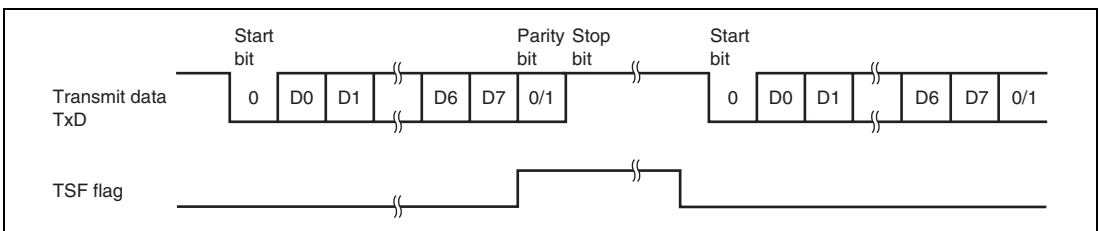
Figure 27.5 Example of Transmit Data Stop Function
