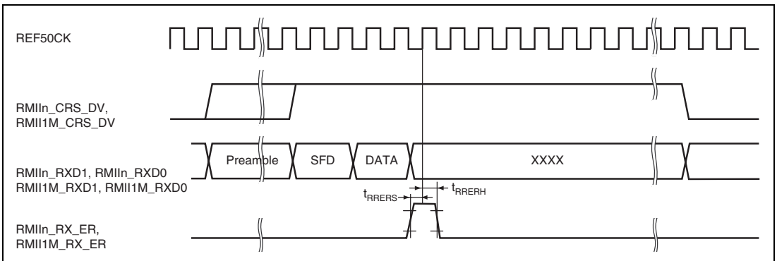
Figure 52.84 RMI Reception Timing (in Case of Error)
