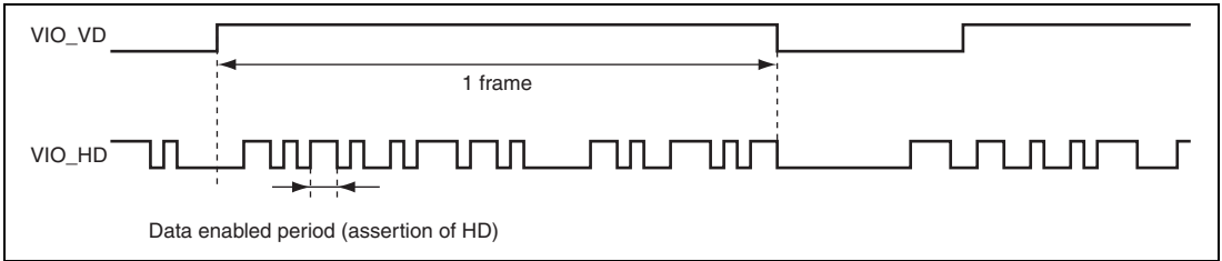
Figure 34.5 Frame Timing (Data Enable Fetch)
