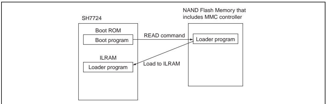
Figure 24.1 Overview of Flash Memory Boot
