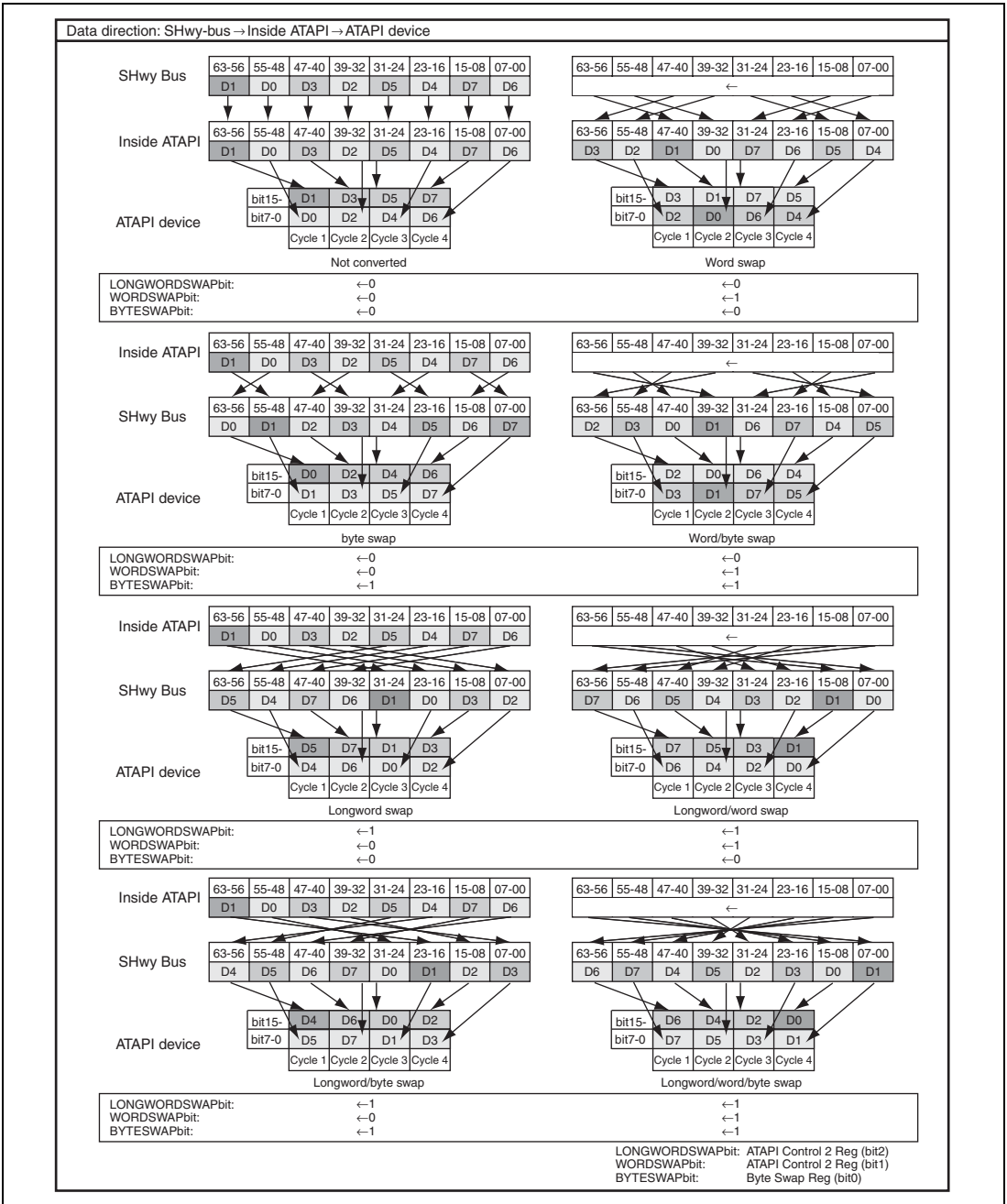
Figure 46.5 ATAPI Data Bus Alignment
