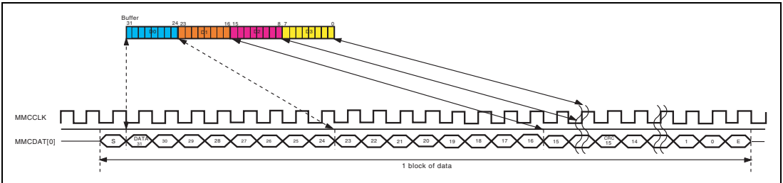
Figure 23.9 Data Format (1-Bit Mode)
