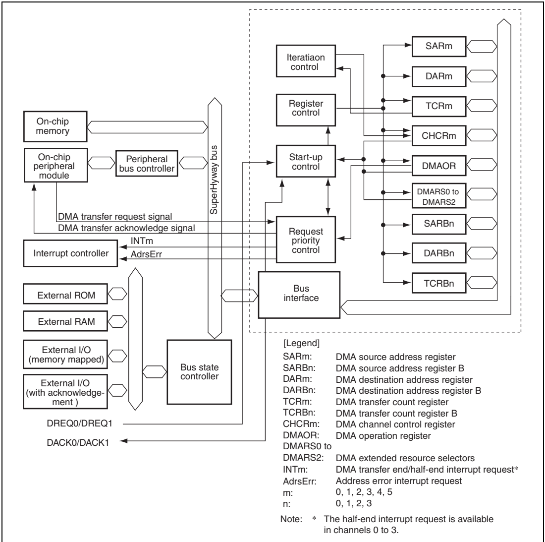
Figure 16.1 Block Diagram of DMAC
