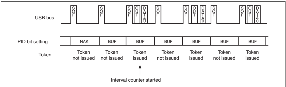
Figure 31.14 Token Issuance when IITV = 1
