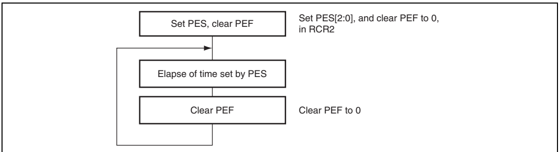
Figure 28.5 Using Periodic Interrupt Function
