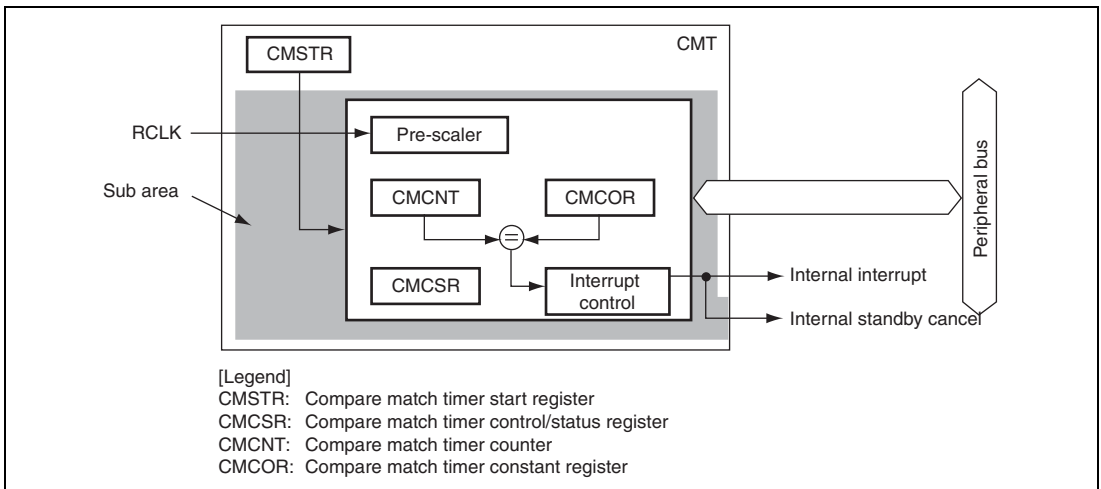
Figure 22.1 Block Diagram of CMT
