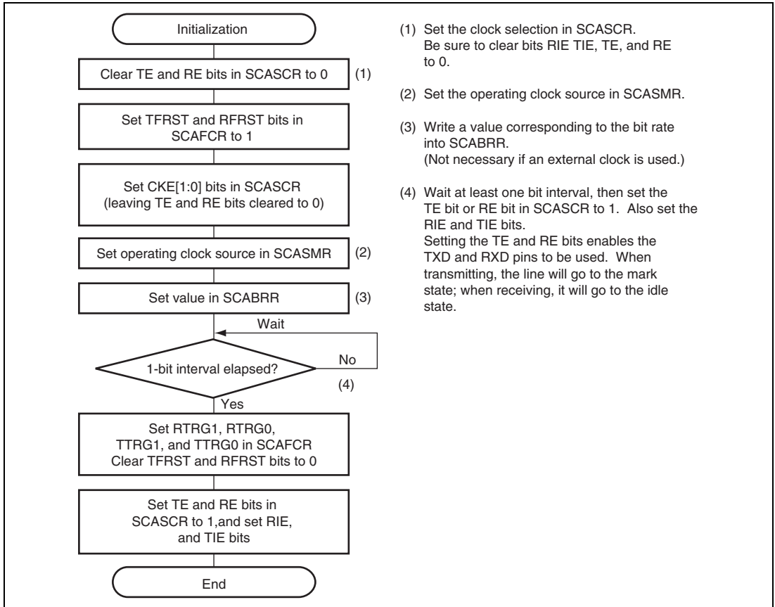
Figure 27.2 Sample SCIFA Initialization Flowchart
