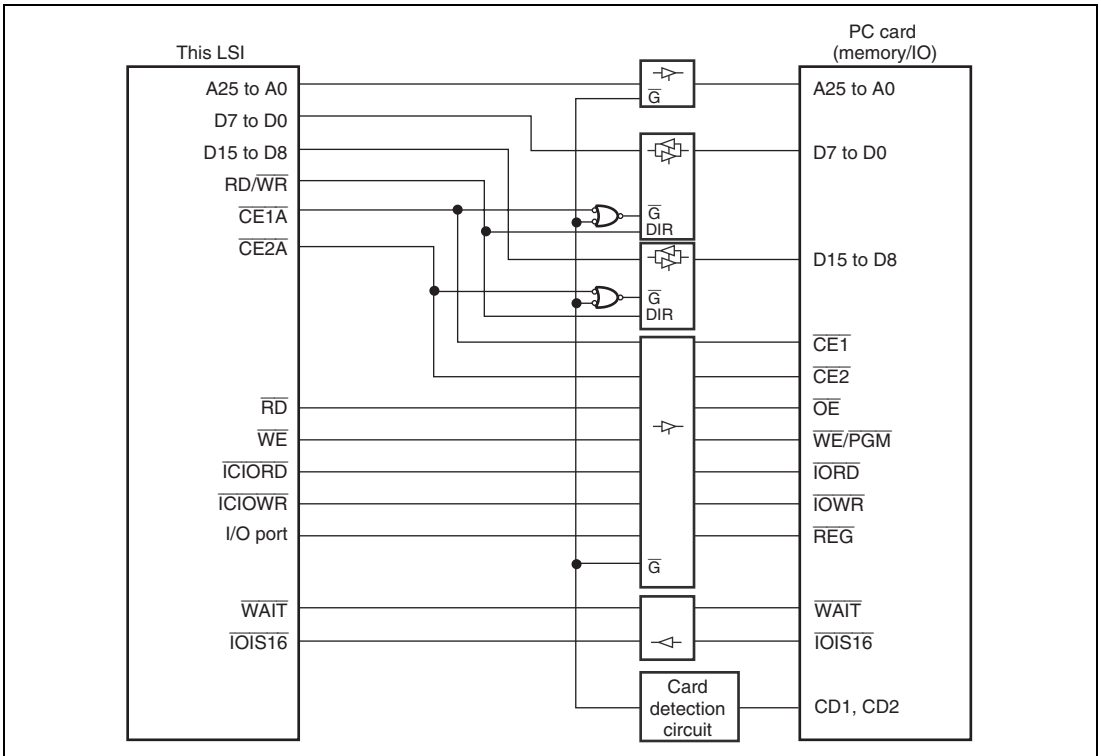
Figure 14.17 Connection Example with PCMCIA Interface
