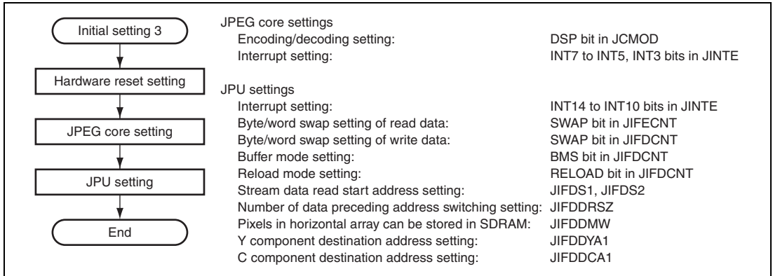
Figure 37.14 Flow of Initial Setting 3
