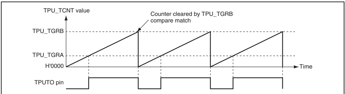
Figure 21.12 Example of PWM Mode Operation (1)
