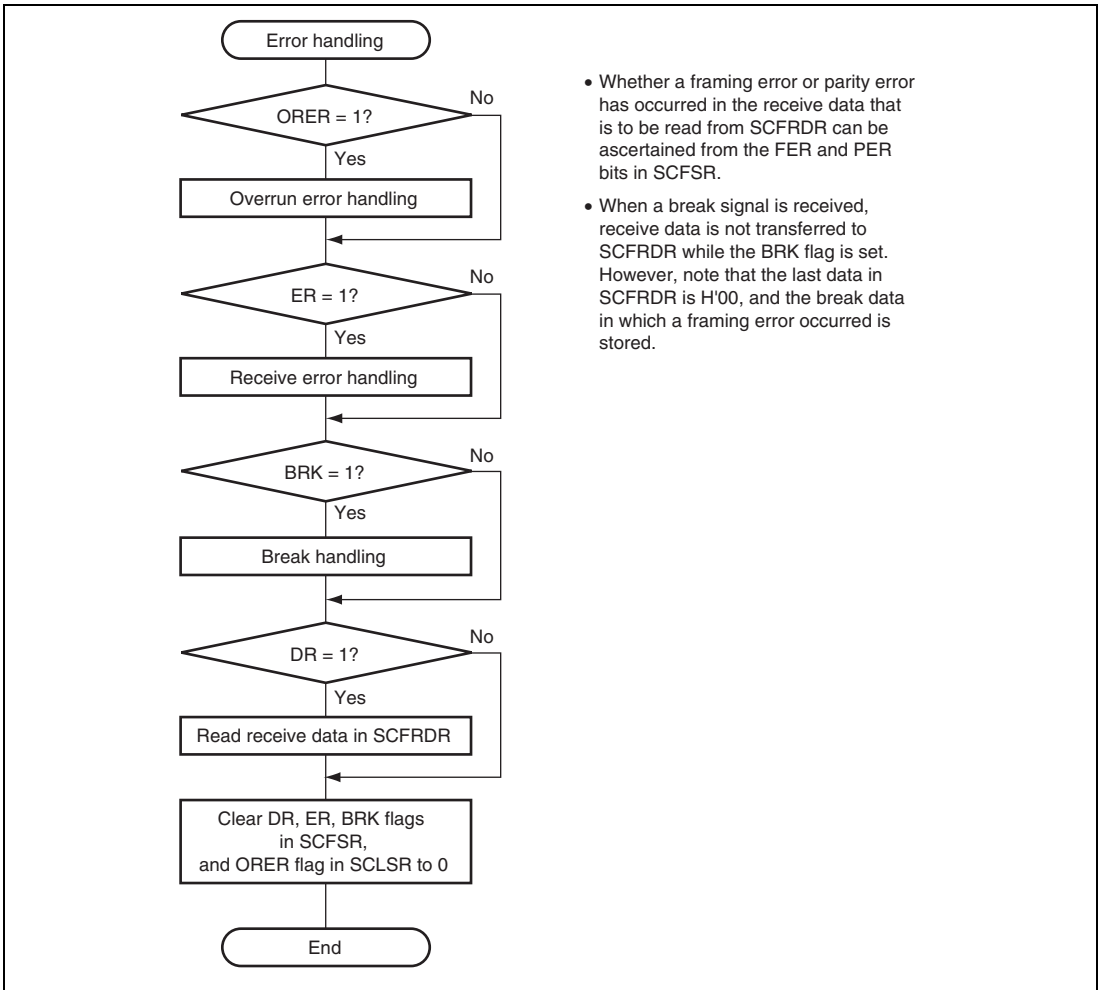
Figure 26.7 Sample Flowchart for Receiving Serial Data (cont)
