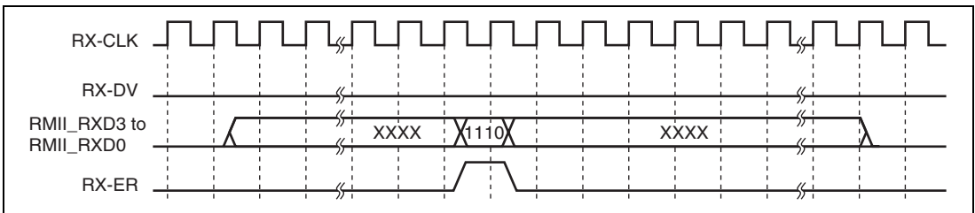
Figure 47.9 (6) MII Frame Receive Timing (Reception Error (2): Carrier Error Notification)
