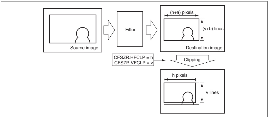
Figure 34.32 Clipping of Image Output from Filter
