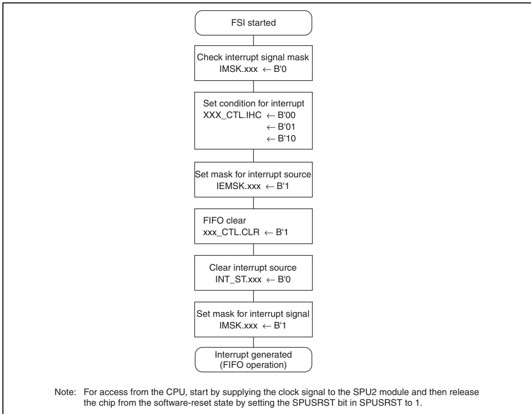
Figure 45.24 Flow for Configuring Initial Interrupt Setting
