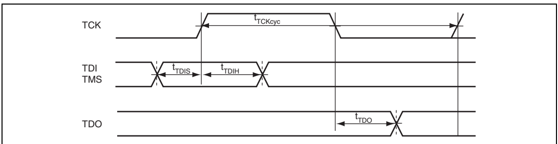
Figure 52.90 H-UDI Data Transfer Timing
