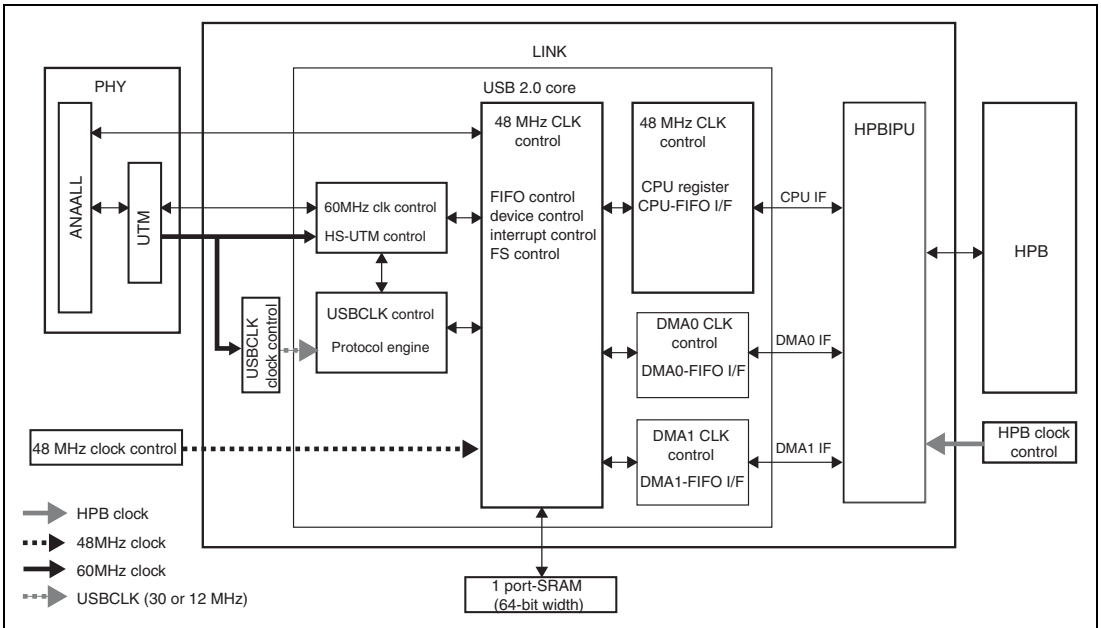
Figure 31.1 USB block diagram
