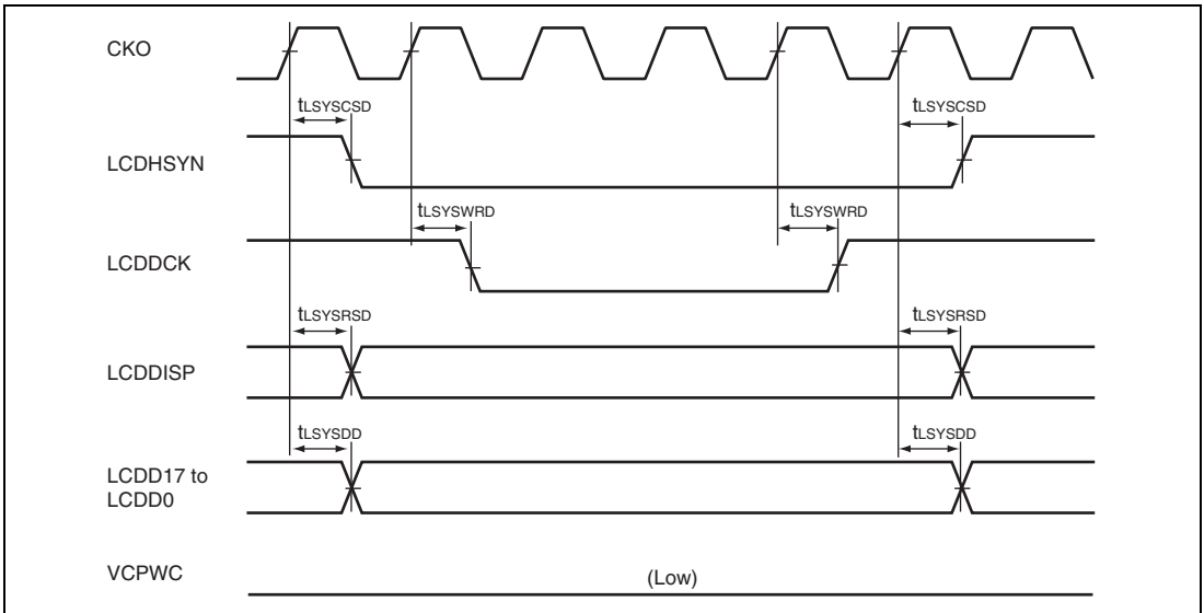
Figure 52.49 LCDC AC Characteristics SYS Interface, Command Write Bus Cycle (MLDMT2R.WCEC = 5, MLDMT2R.WCLW = 3)
