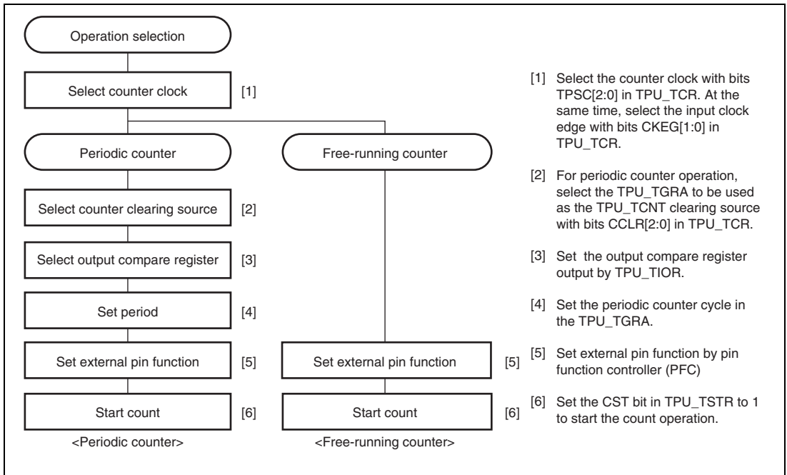
Figure 21.2 Example of Counter Operation Setting Procedure
