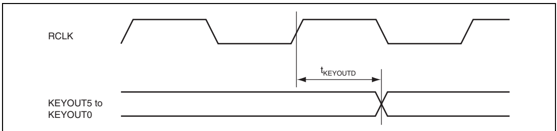
Figure 52.57 KEYOUT Output Timing
