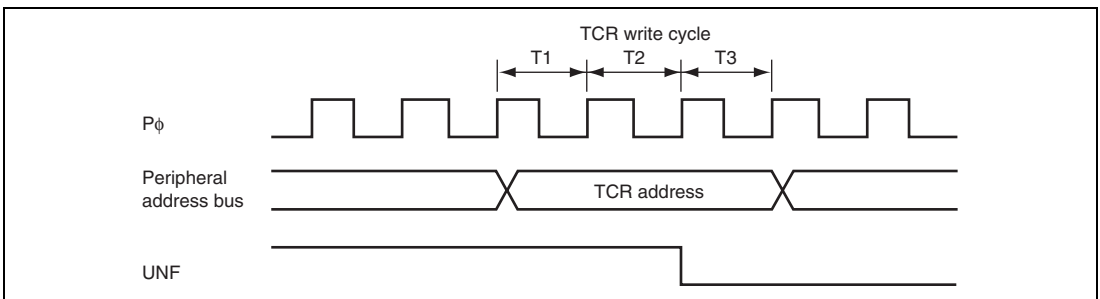
Figure 20.6 Status Flag Clear Timing
