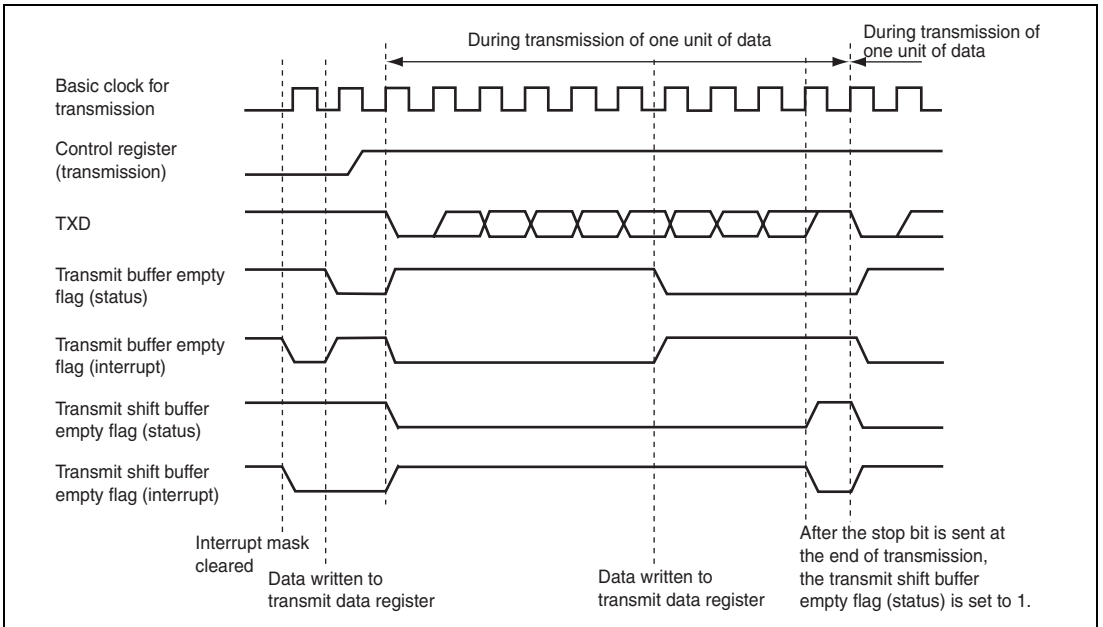
Figure 29.3 Data Transmission Timing
