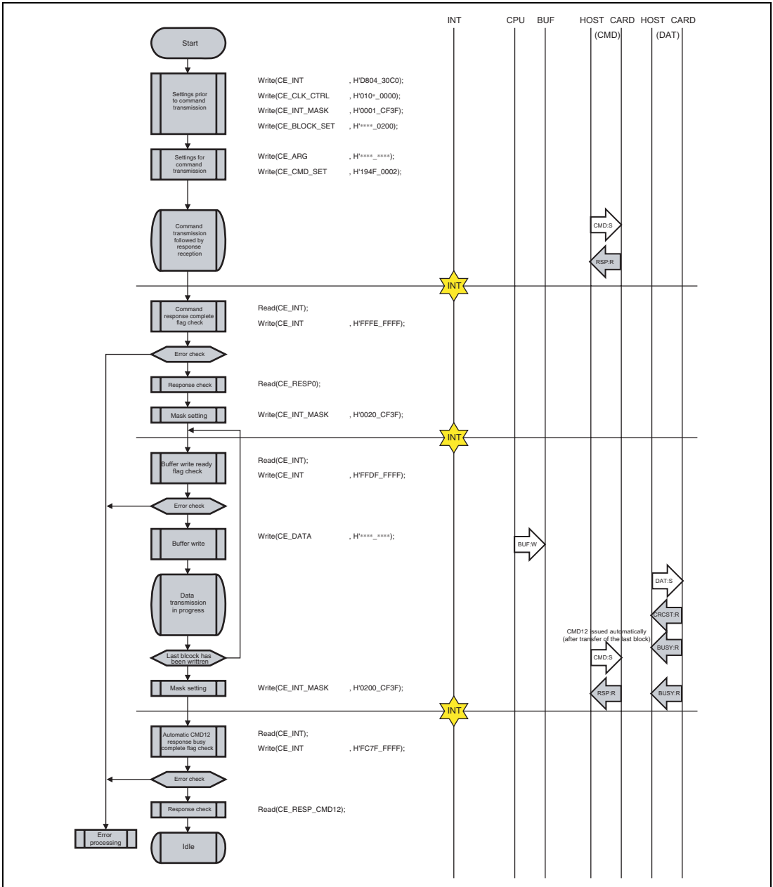
Figure 23.19 Multi-Block Write (with Automatic CMD12 Issuance) (CMD25)
