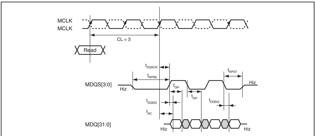
Figure 52.35 Mobile-DDR-SDRAM Input Timing (Read)
