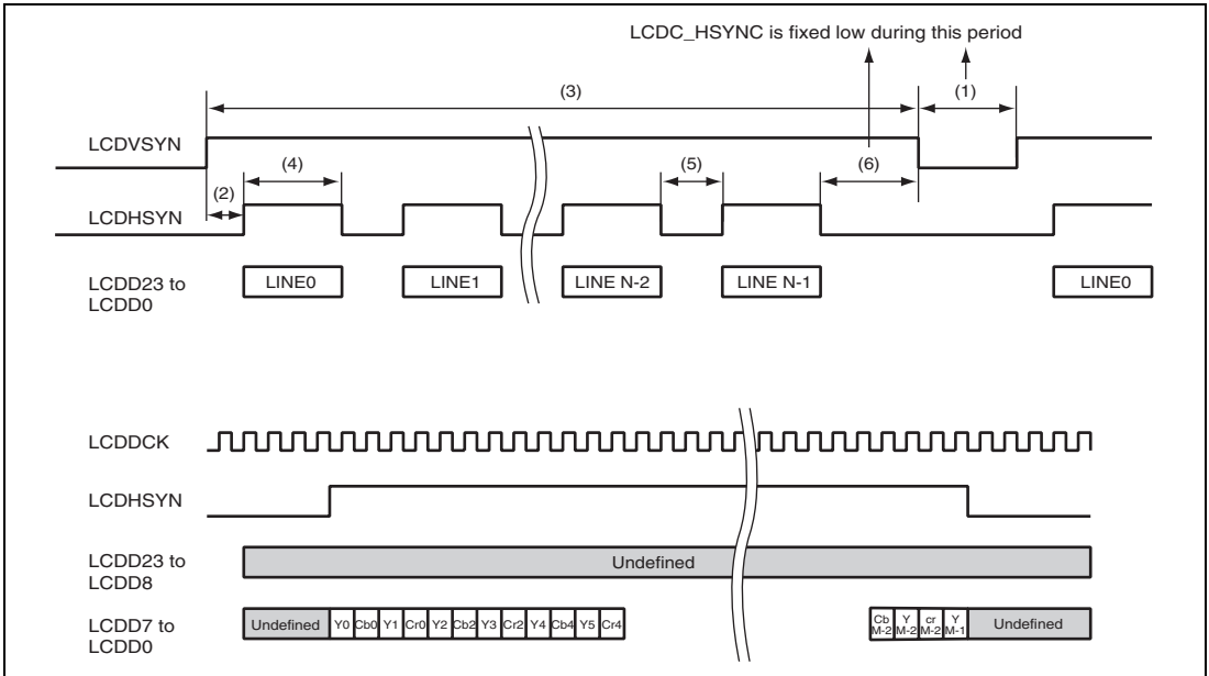
Figure 39.9 Example of Output Signals in YCbCr Operating Mode
