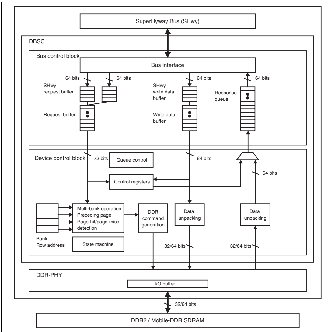
Figure 15.1 Block Diagram of the DBSC
