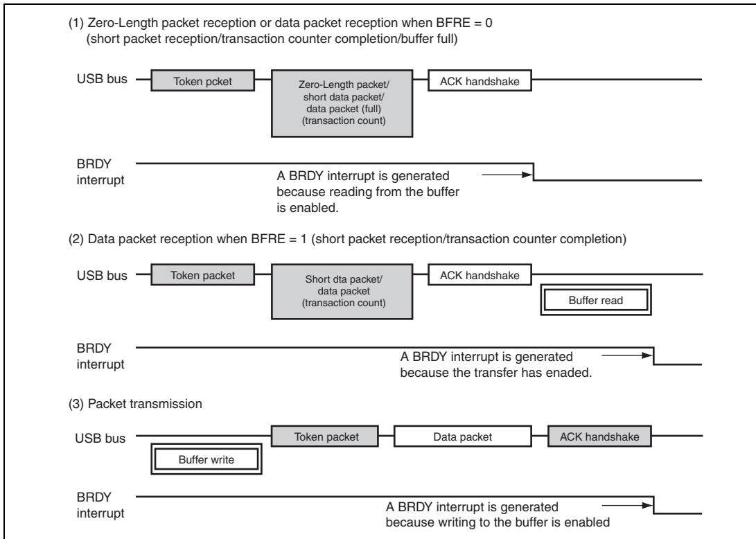
Figure 31.4 Timing at which a BRDY Interrupt is Generated
