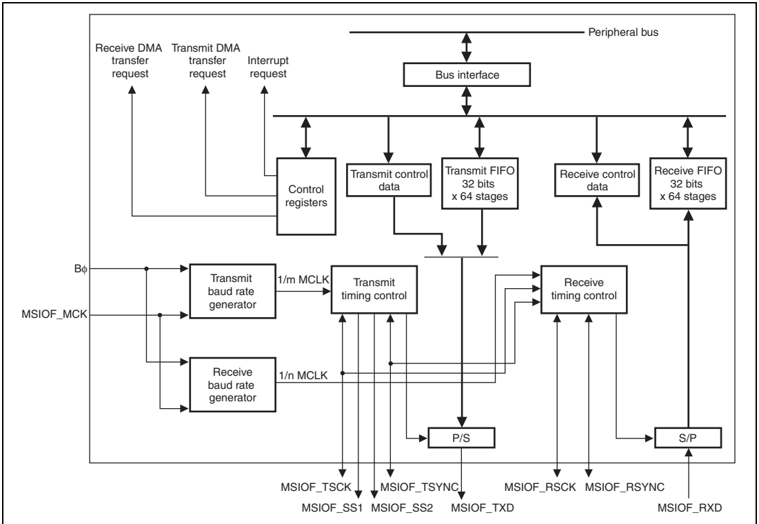
Figure 25.1 Block Diagram of MSIOF
