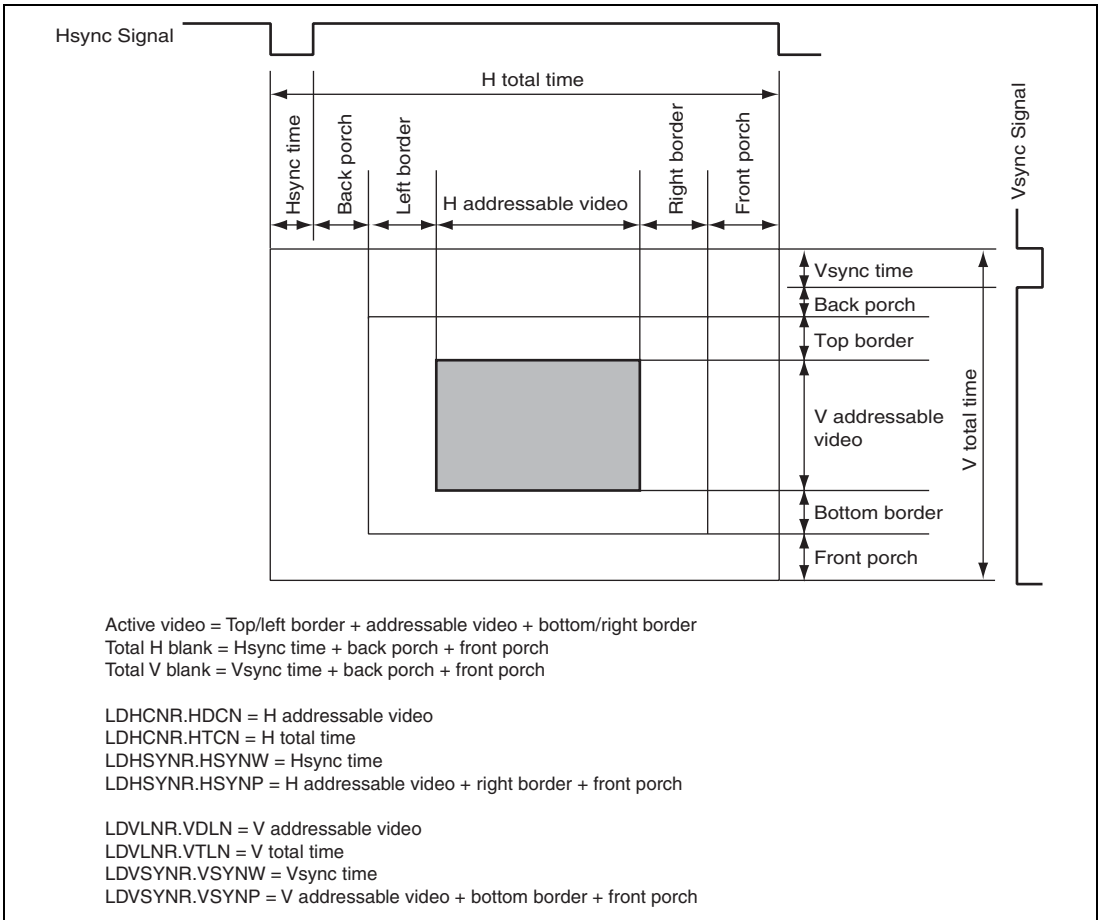
Figure 39.5 Valid Display and Blanking Periods
