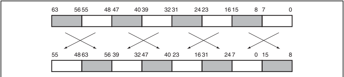
Figure 42.5 Data Before and After Byte Swapping
