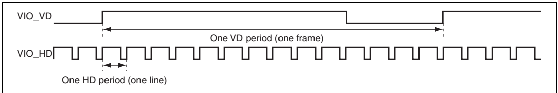
Figure 34.3 Frame Timing
