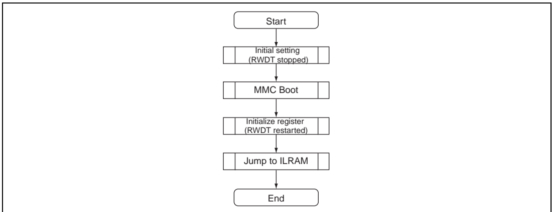
Figure 24.2 Overview of the Boot Program
