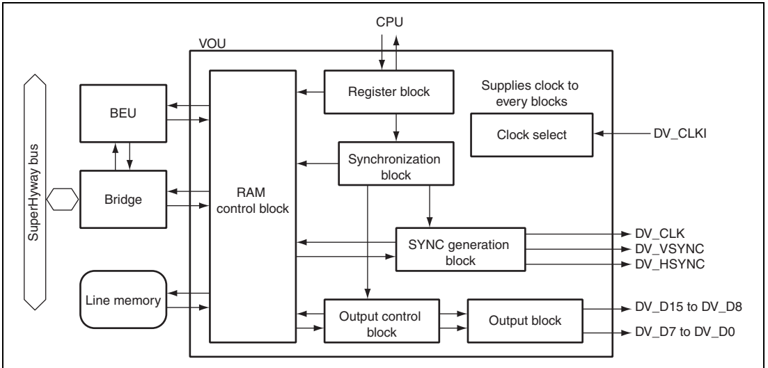
Figure 40.1 VOU Block Diagram
