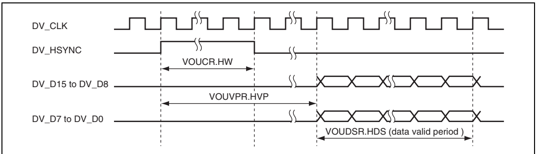
Figure 40.8 Timing of HSYNC and Data Valid Period
