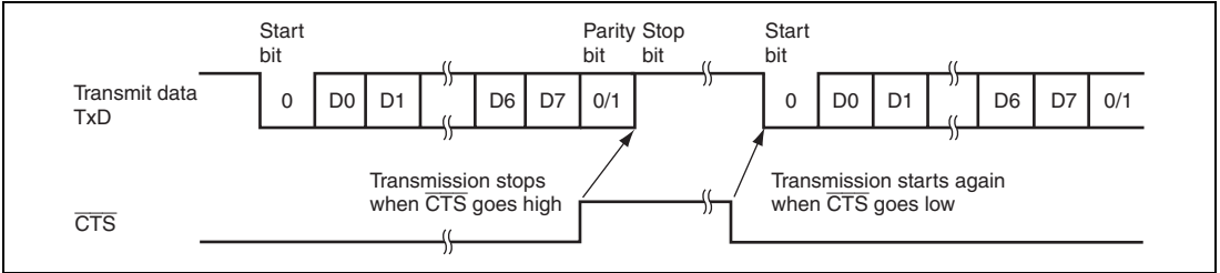
Figure 27.10 Example of \overline{\text{CTS}} Control Operation
