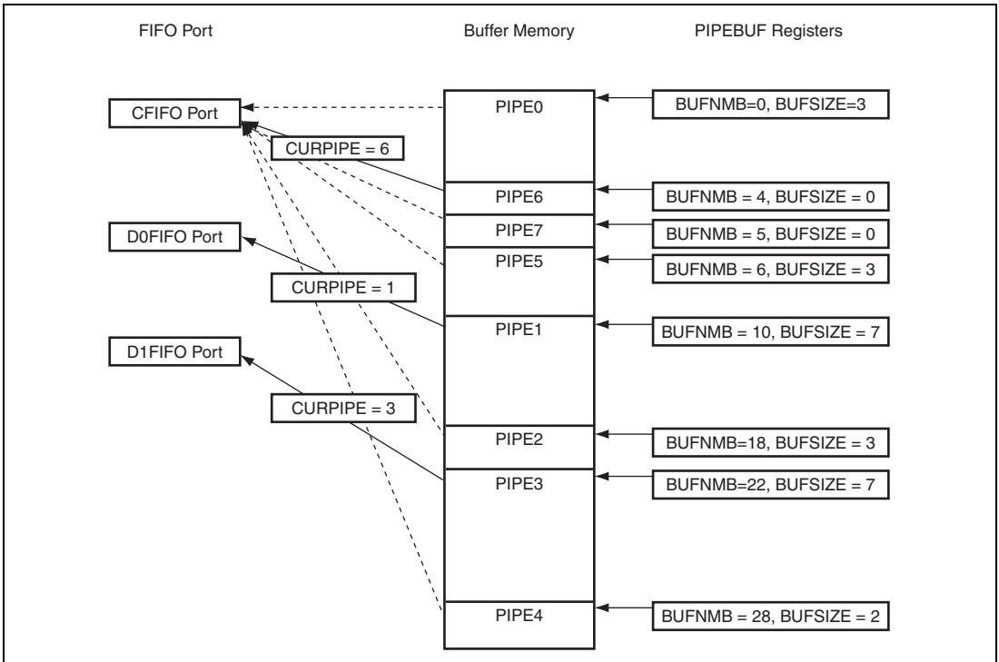
Figure 31.10 Example of a Buffer Memory Map
