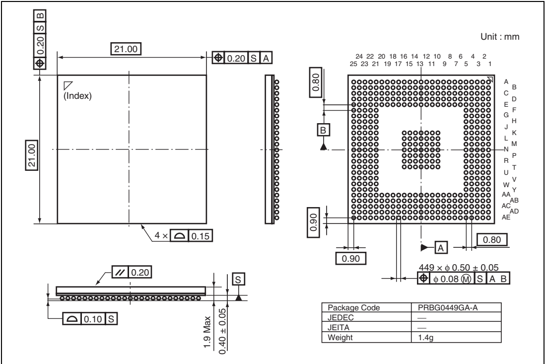
Figure E.1 Package Dimension
