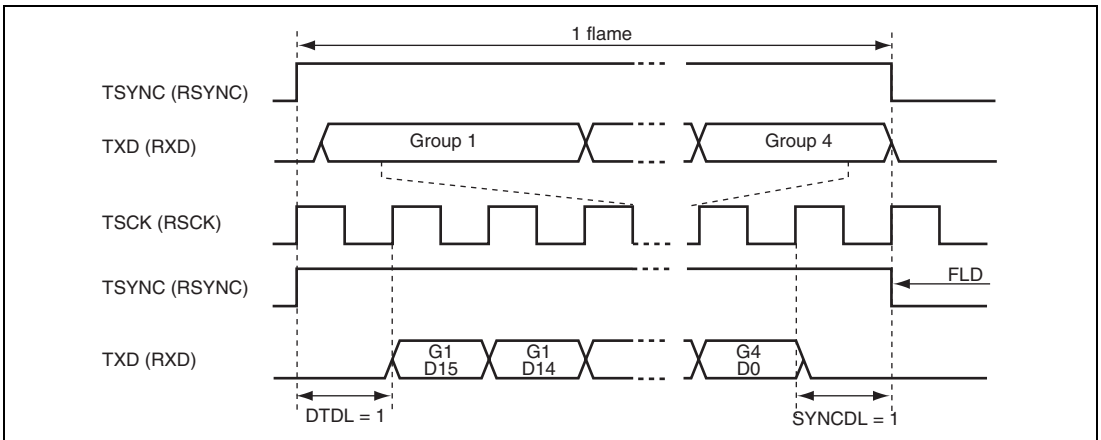
Figure 25.5 Synchronization Timing in Level Synchronization Mode
