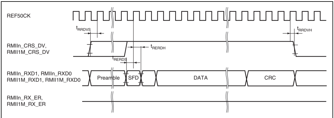
Figure 52.83 RMI Reception Timing (Normal Operation)
