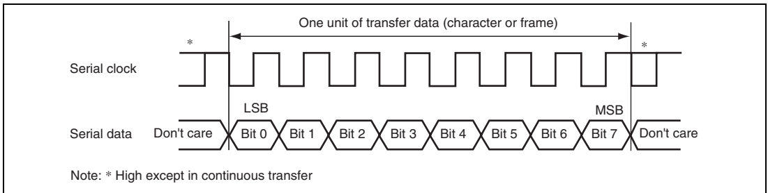
Figure 26.9 Data Format in Clock Synchronous Communication
