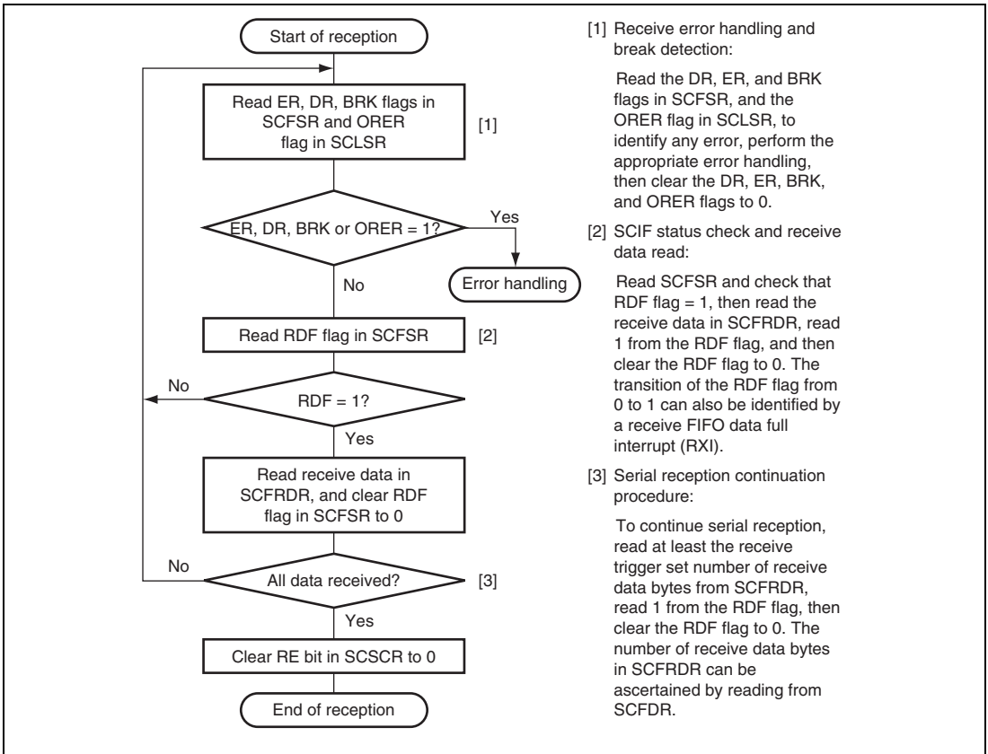
Figure 26.6 Sample Flowchart for Receiving Serial Data
