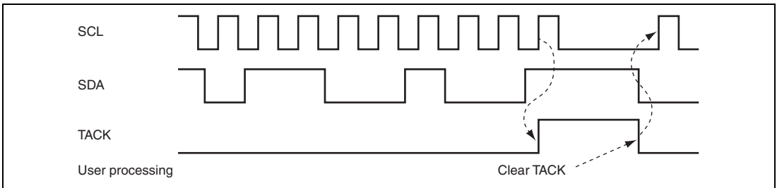
Figure 32.14 Example of Non-Acknowledge Operation Timing
