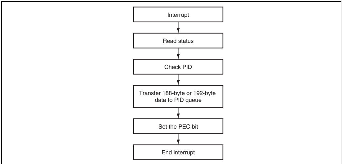
Figure 43.8 TSIF Interrupt Process Flow
