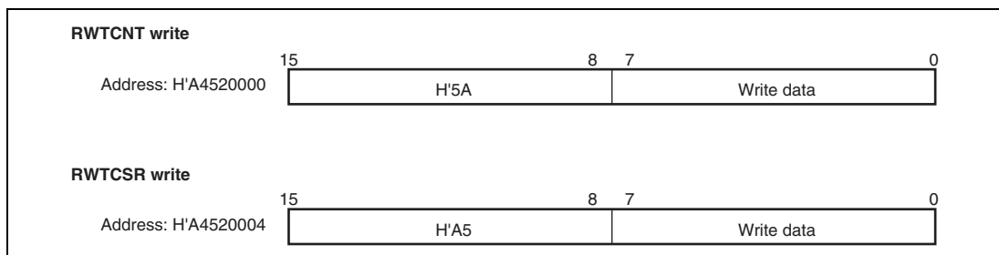
Figure 19.2 Writing to RWTCNT and RWTCR
