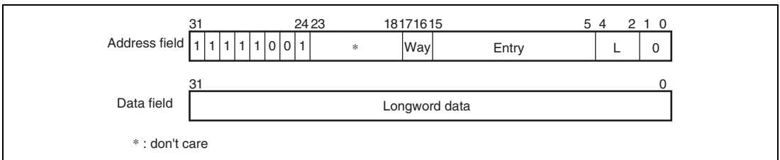
Figure 9.3 Memory-Mapped Secondary Cache Data Array
