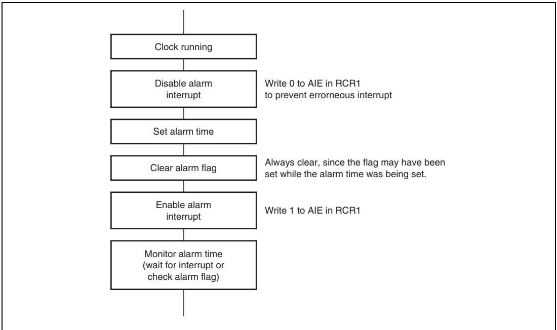
Figure 28.4 Using Alarm Function
