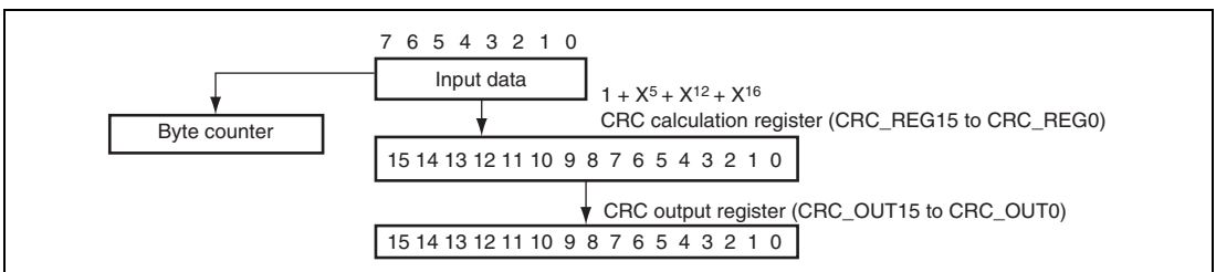
Figure 29.8 CRC Engine Operation
