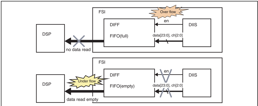
Figure 45.13 Input FIFO Overflow/Underflow
