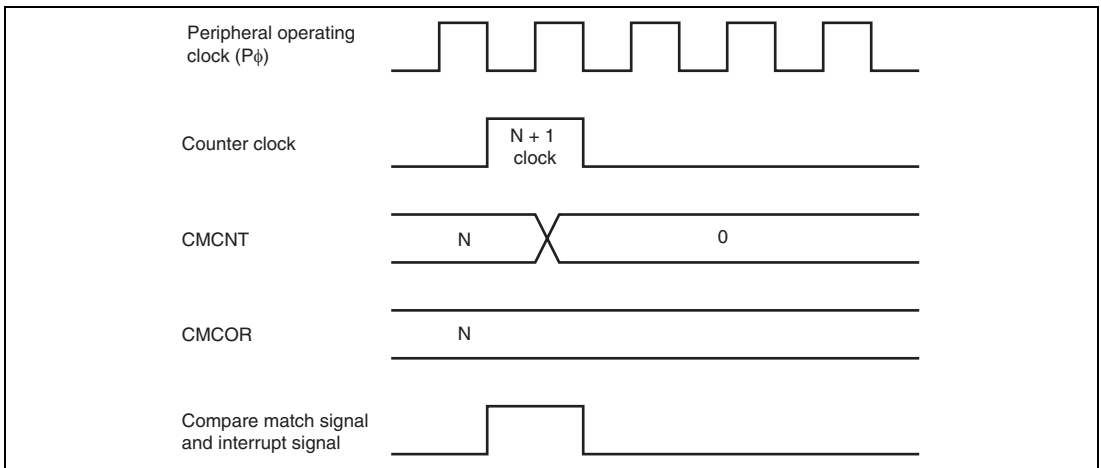
Figure 22.4 CMF Set Timing
