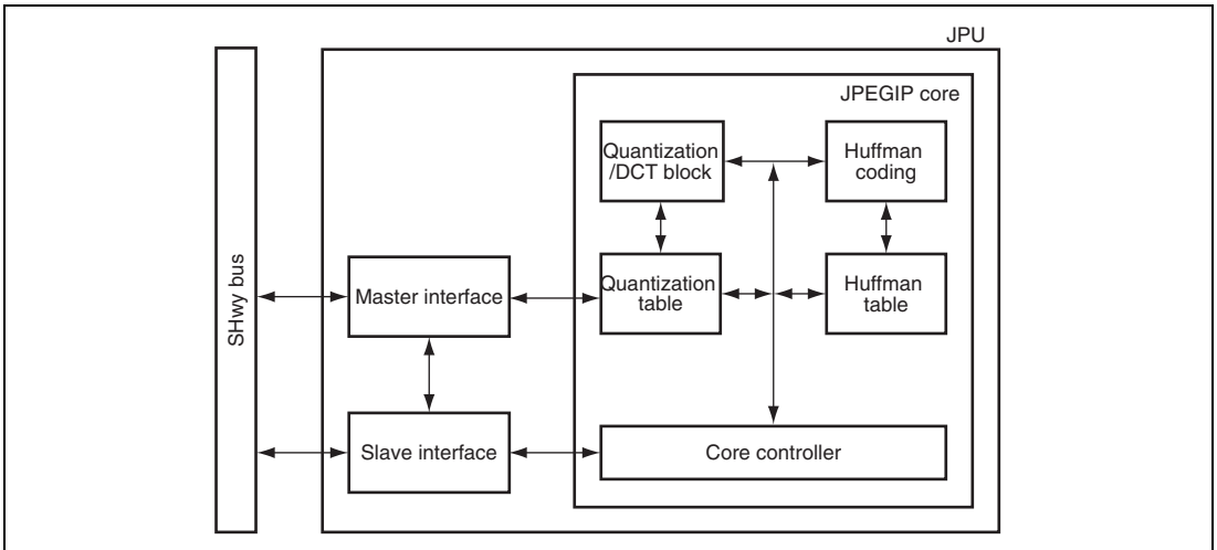
Figure 37.1 Connection between JPU and Peripheral Modules
