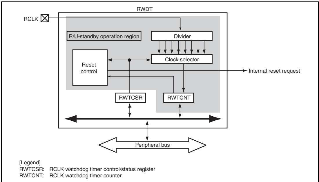
Figure 19.1 Block Diagram of RWDT
