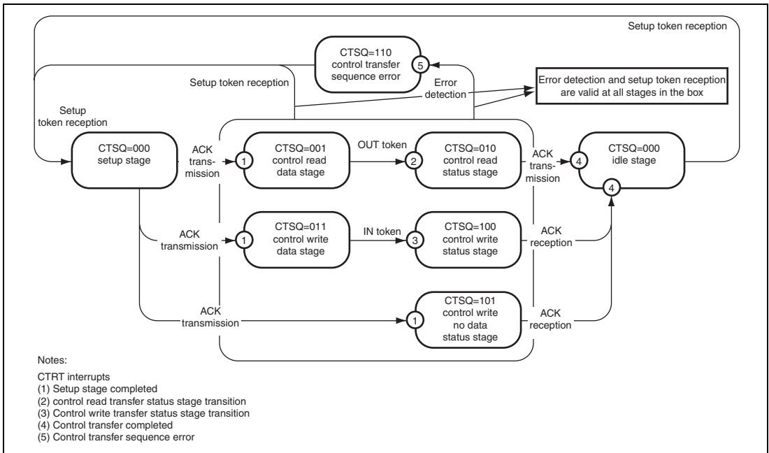
Figure 31.8 Control Transfer Stage Transitions
