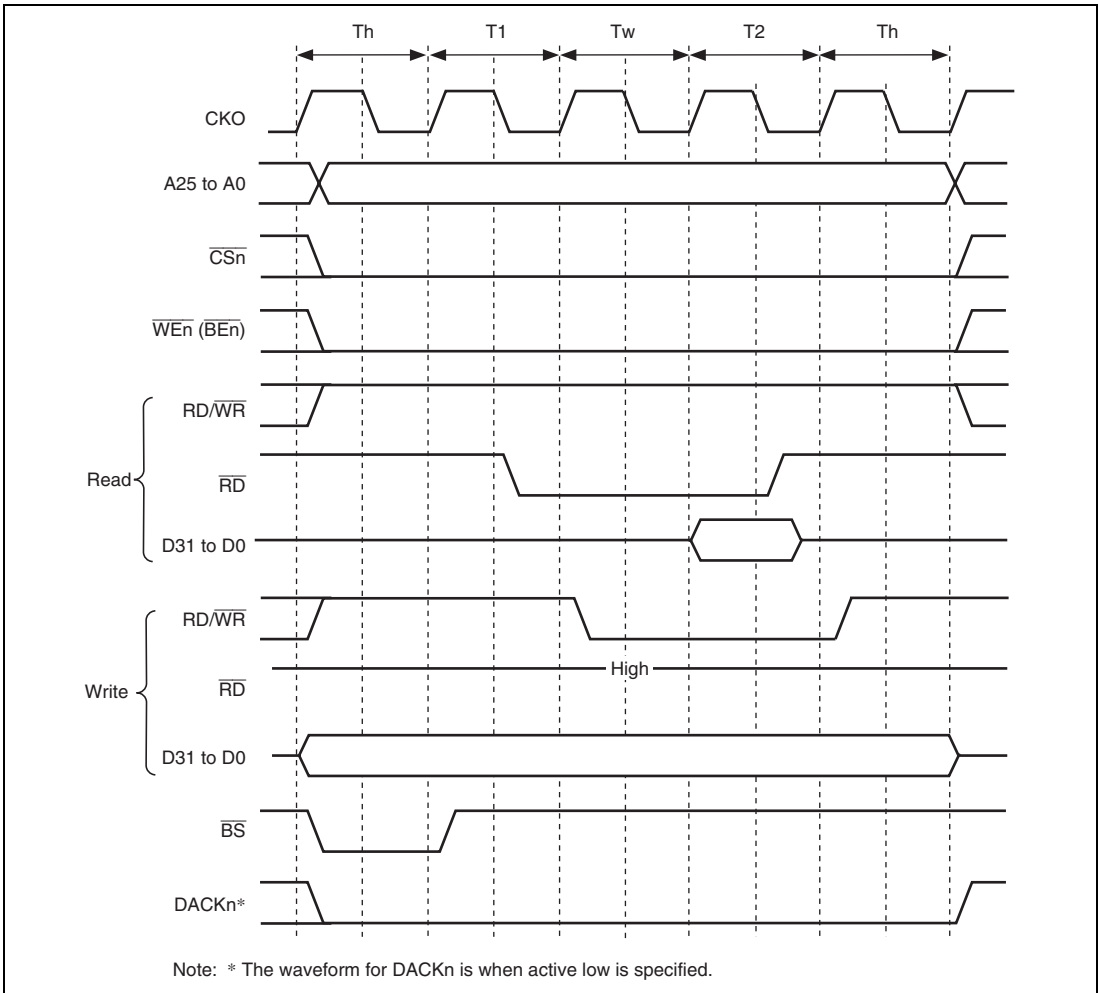
Figure 14.14 Wait Timing for SRAM with Byte Selection (BAS = 1) (for Software Waiting only)
