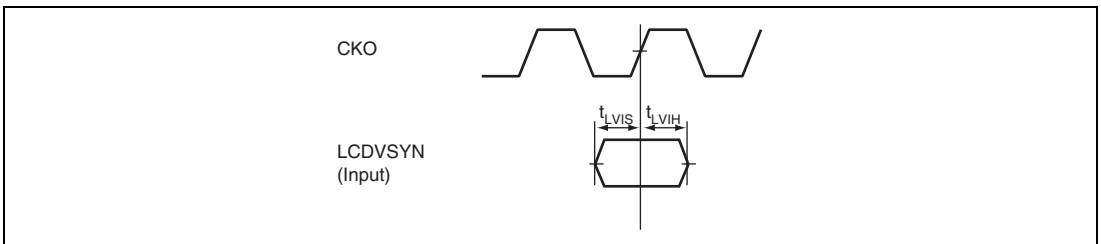
Figure 52.52 LCDC AC Characteristics (VSYNC Input Mode)
