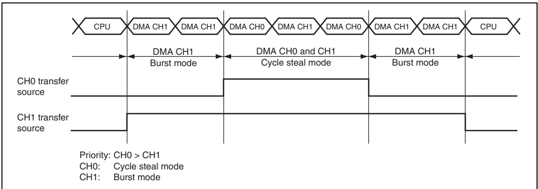
Figure 16.9 Bus State when Multiple Channels are Operating
