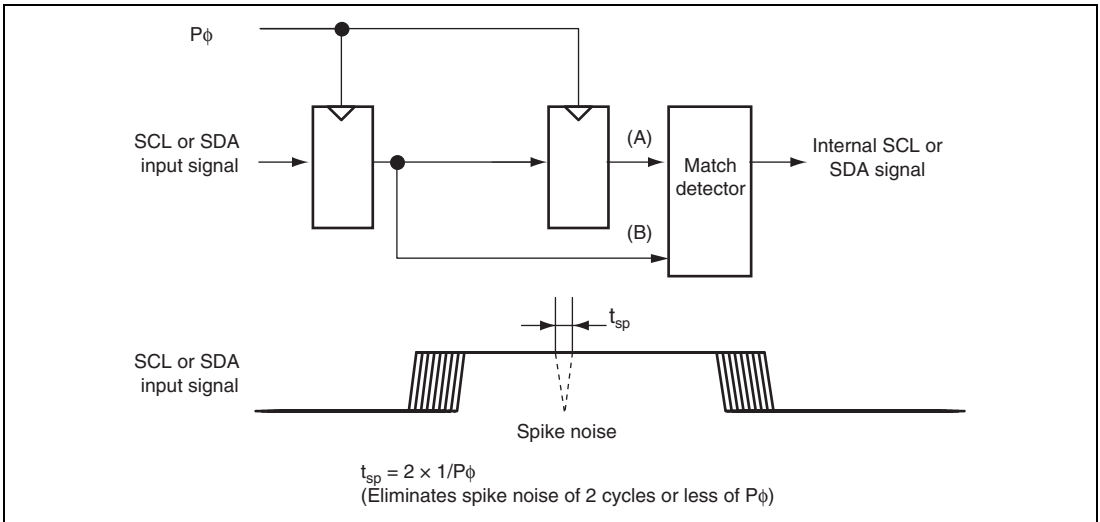
Figure 32.12 Block Diagram of Noise Canceler
