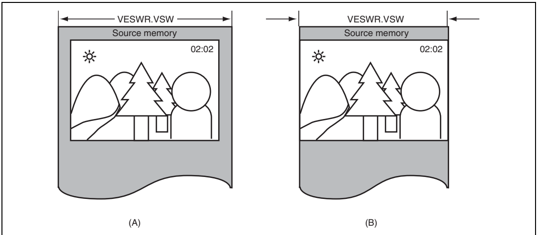
Figure 35.6 Relationship between Image Clipping Size and VESWR
