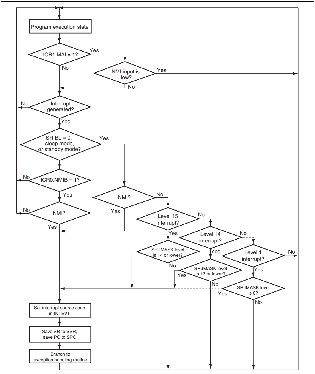
Figure 13.2 Interrupt Operation Flowchart (when CPUOPM.INTMU = 0)
