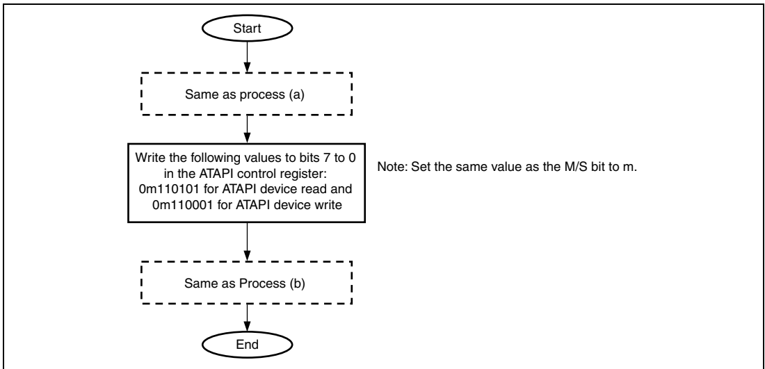
Figure 46.15 Transfer to and from Memory via SHwy Bus by Polling
