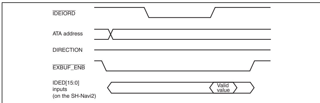
Figure 46.6 PIO Read Data Transfer
