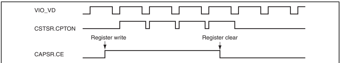
Figure 34.8 Continuous-Frame Capture
