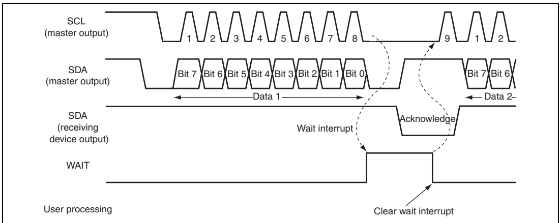
Figure 32.15 Example of Wait Operation Timing
