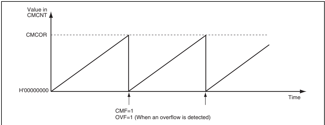
Figure 22.3 Counter Operation (Free-Running Operation)
