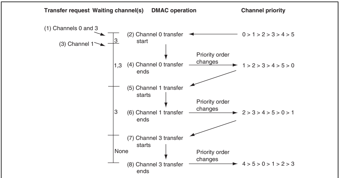
Figure 16.3 Changes in Channel Priority in Round-Robin Mode
