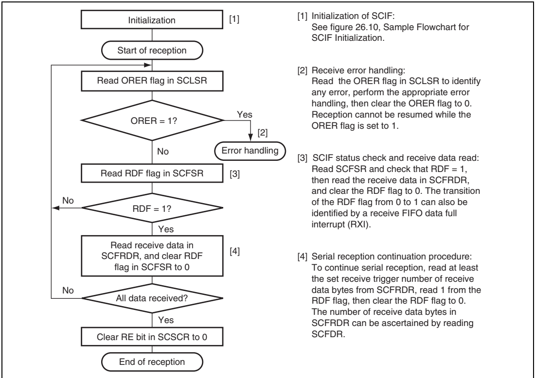
Figure 26.13 Sample Flowchart for Receiving Serial Data (1)
