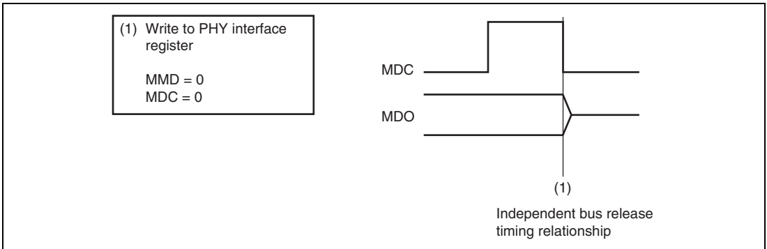
Figure 47.11 (4) Independent Bus Release Flowchart (IDLE in Write in Figure 47.10)
