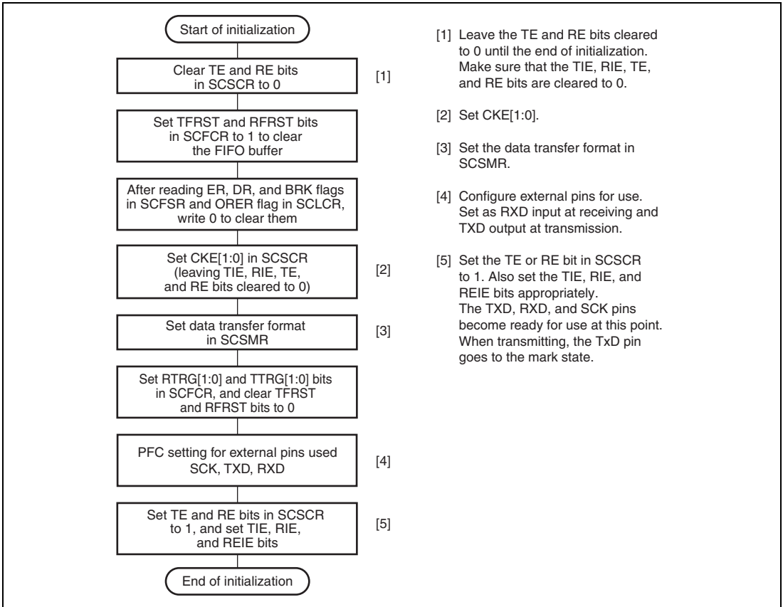
Figure 26.10 Sample Flowchart for SCIF Initialization
