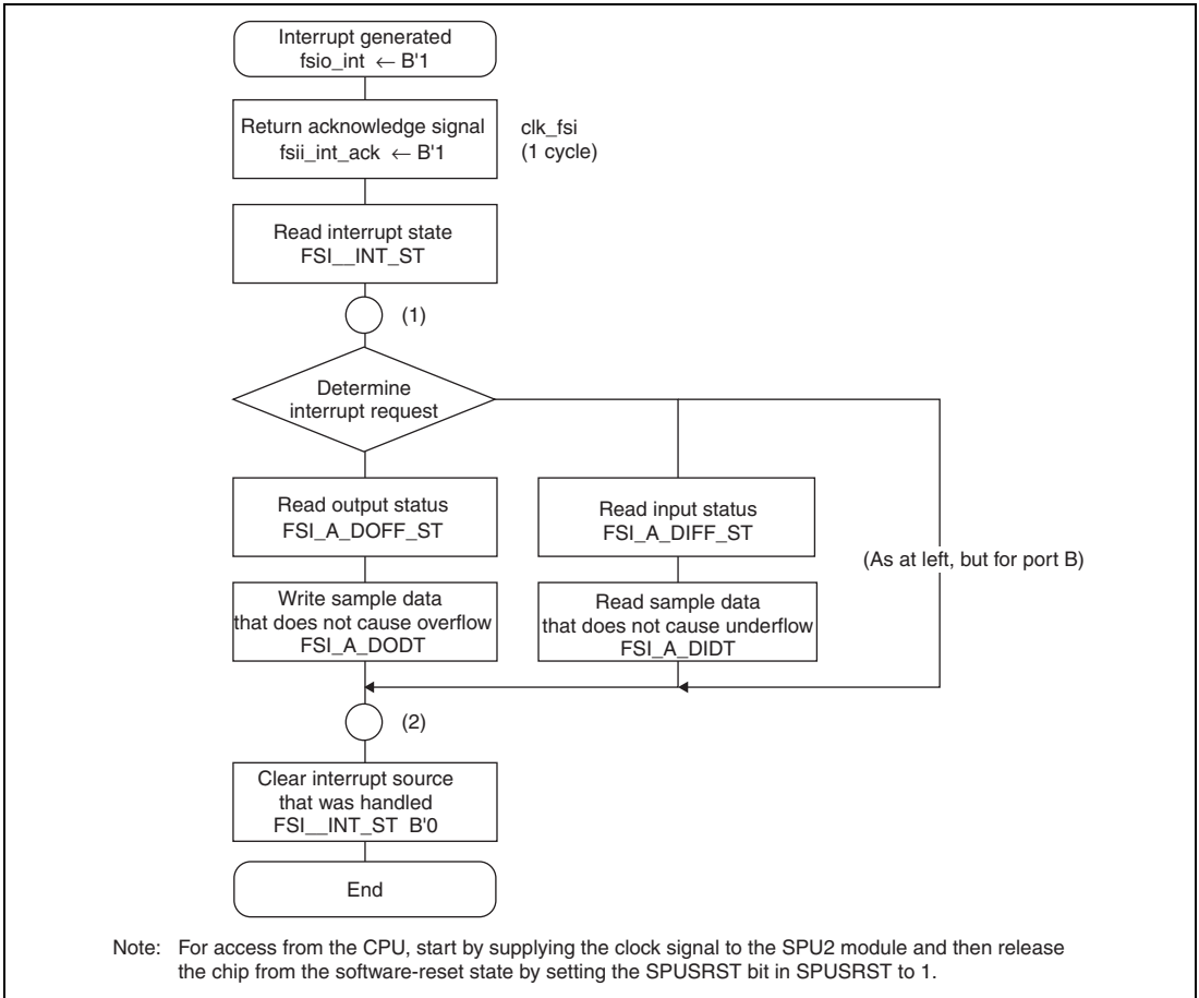
Figure 45.25 Example of SPU2/DSP Operation Flow when FSI Interrupts Occur
