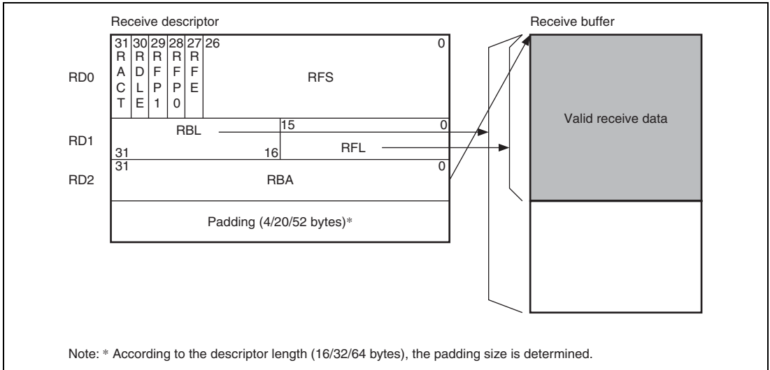
Figure 47.3 Relationship between Receive Descriptor and Receive Buffer
