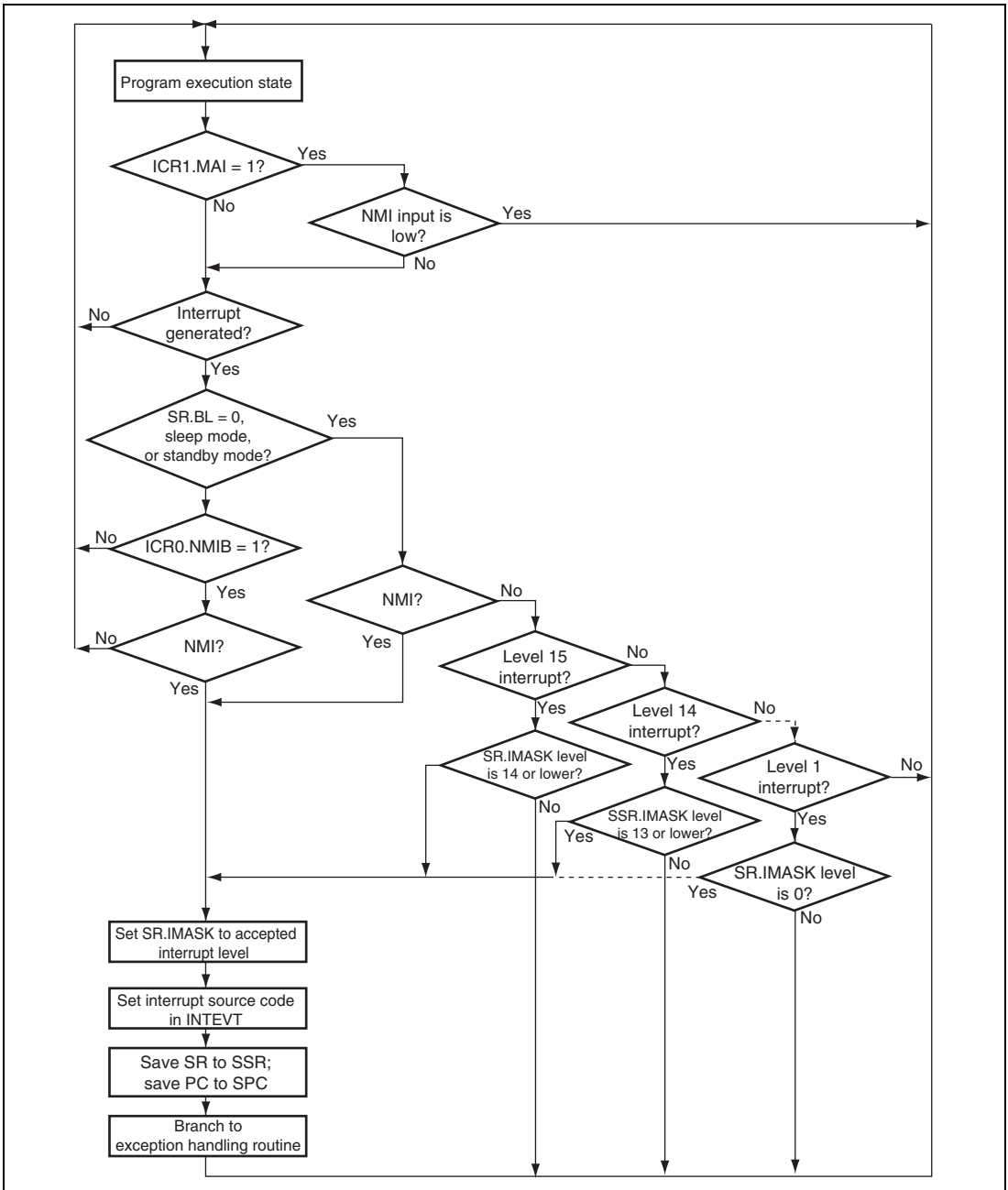
Figure 13.3 Interrupt Operation Flowchart (when CPUOPM.INTMU = 1)
