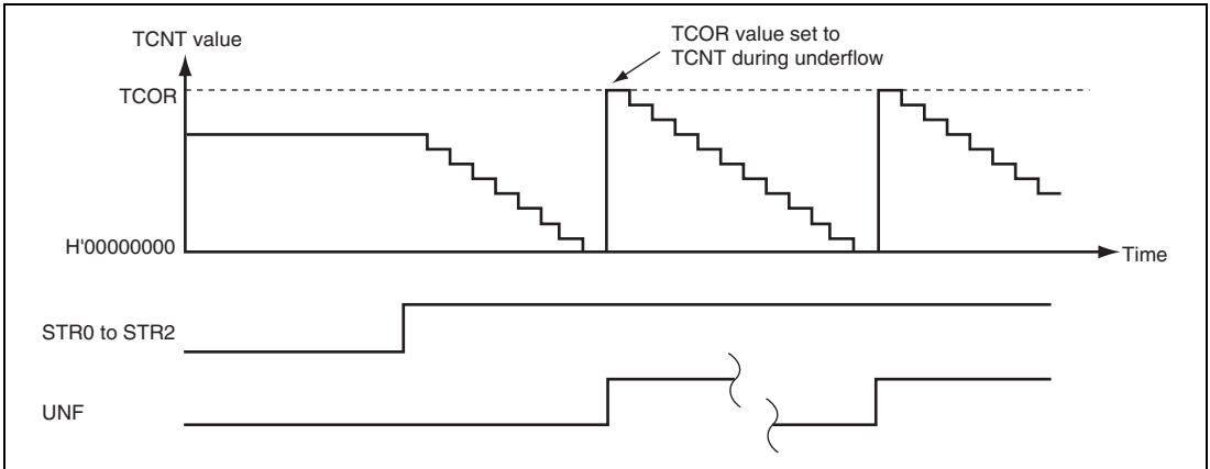
Figure 20.3 Auto-Reload Count Operation
