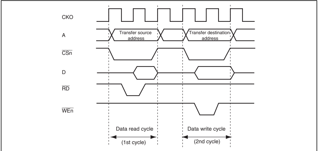
Figure 16.5 Example of DMA Transfer Timing in Dual Mode (Source: Ordinary Memory, Destination: Ordinary Memory)
