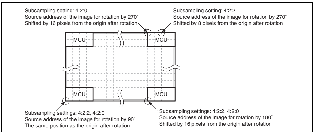
Figure 37.12 Position of Source Addresses for Rotation
