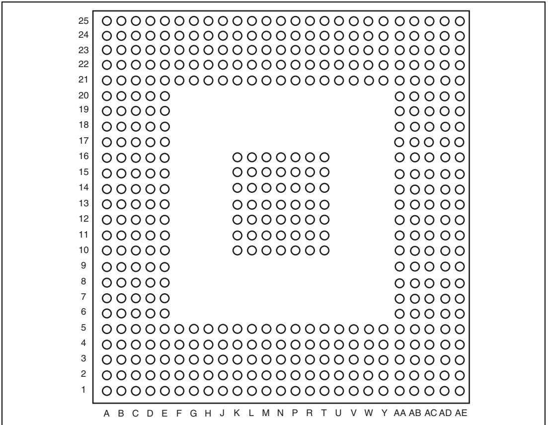
Figure 1.2 BGA449 Pin Arrangement (Top View)
