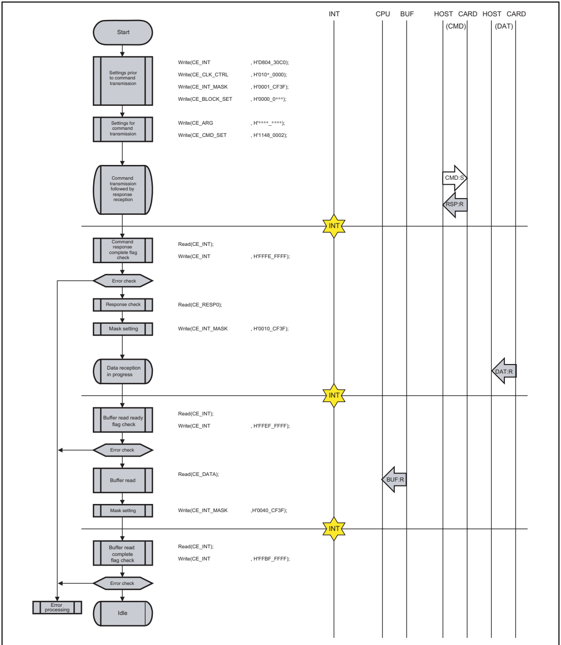
Figure 23.16 Single-Block Read (CMD17)
