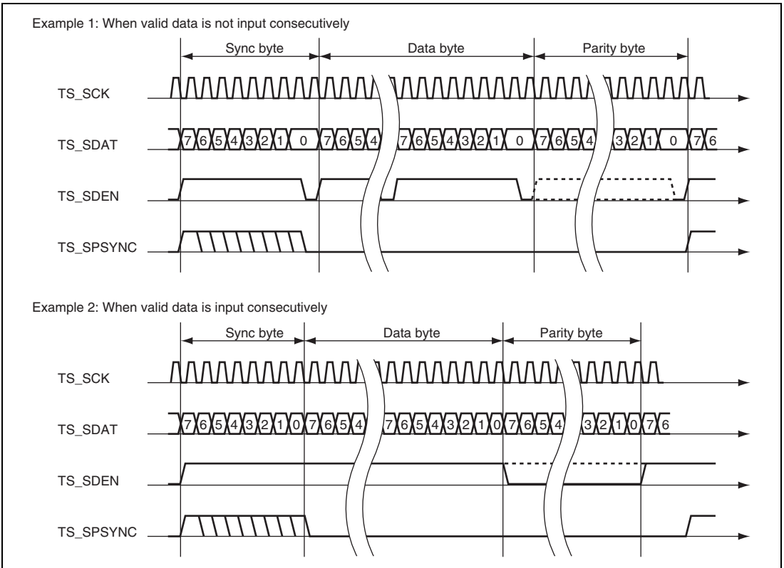
Figure 43.3 Timing of TS Data Serial Input
