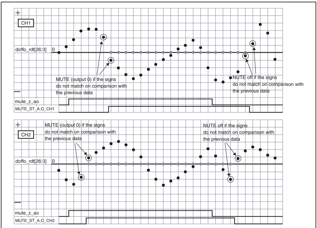
Figure 45.11 Zero Cross MUTE Specification (Output Operation)
