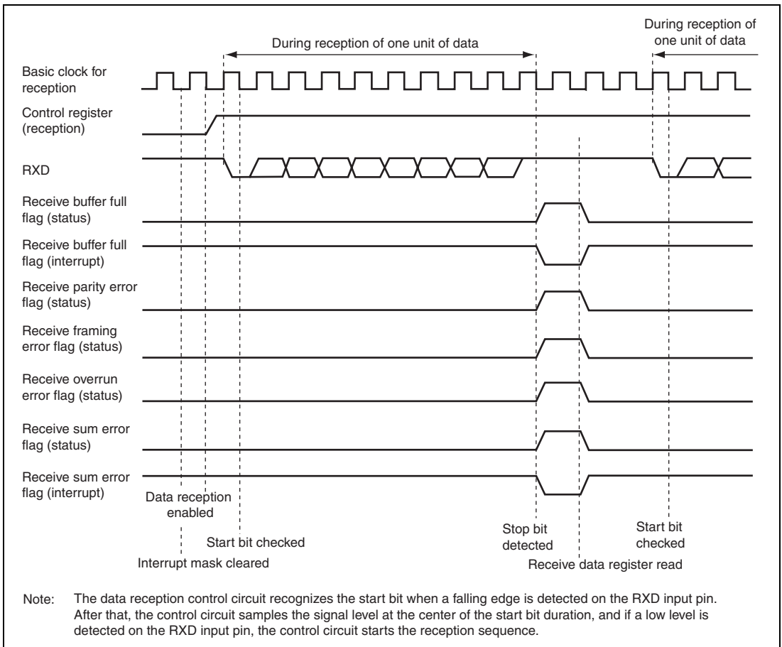
Figure 29.4 Data Reception Timing
