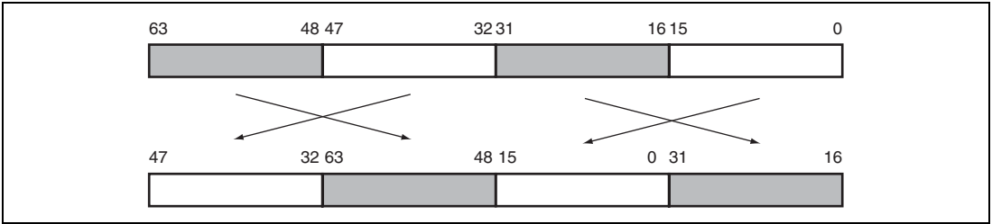
Figure 42.4 Data Before and After Word Swapping
