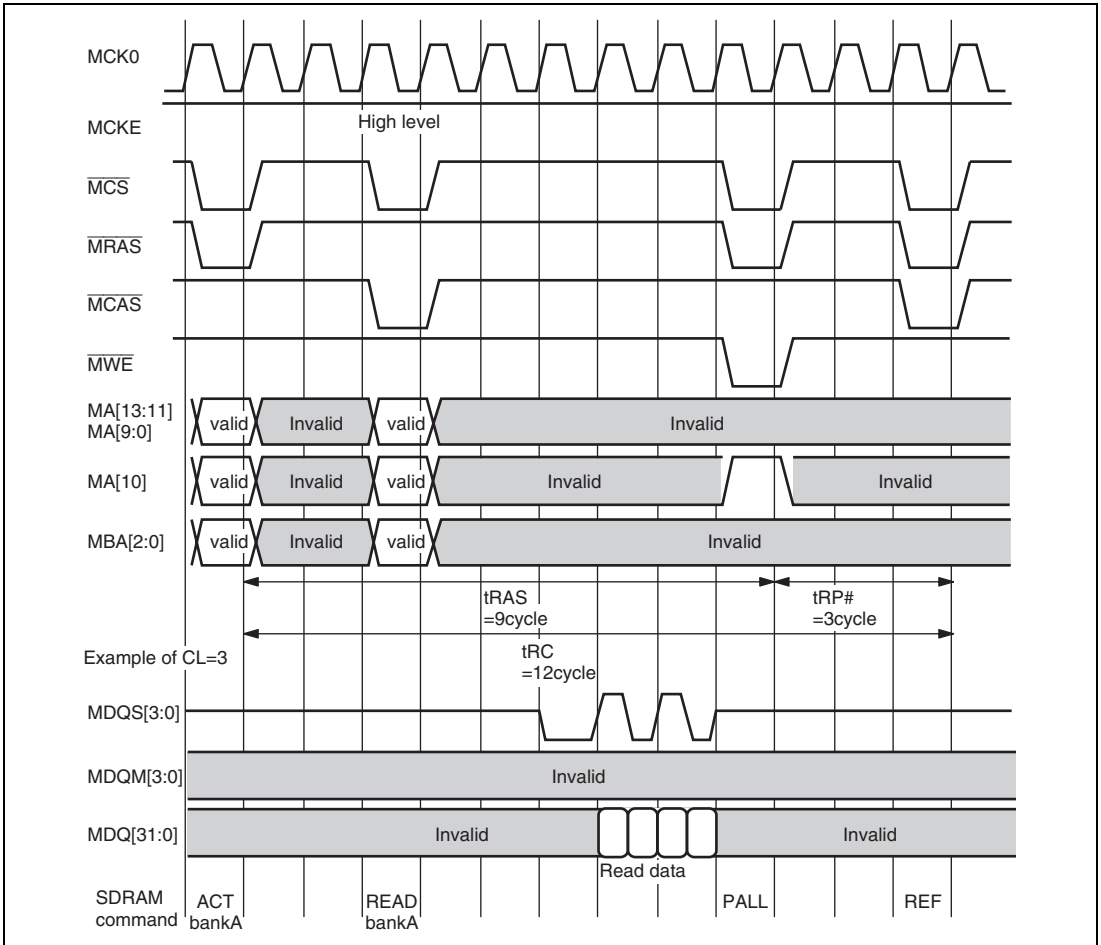
Figure 15.16 tRC
