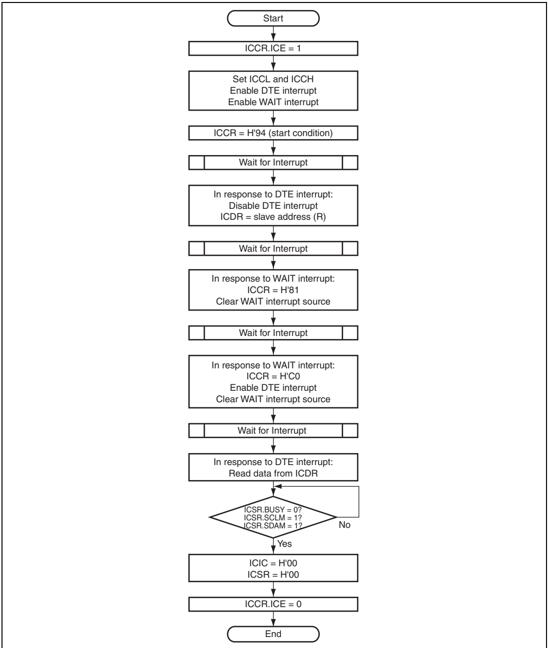
Figure 32.17 Example Flow of Software for 1-Byte Read with Use of Wait Interrupt
