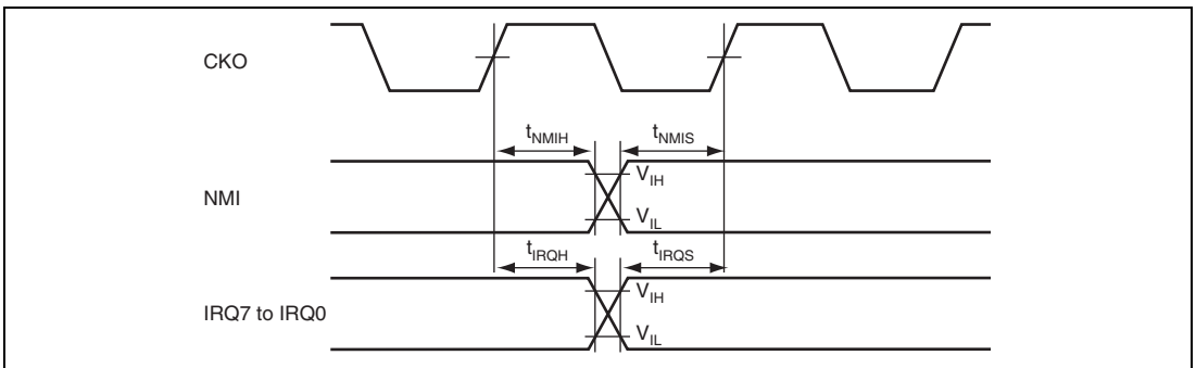
Figure 52.9 Interrupt Signal Input Timing
