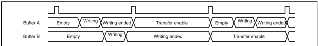
Figure 31.18 Example of Buffer Flush Function Operation
