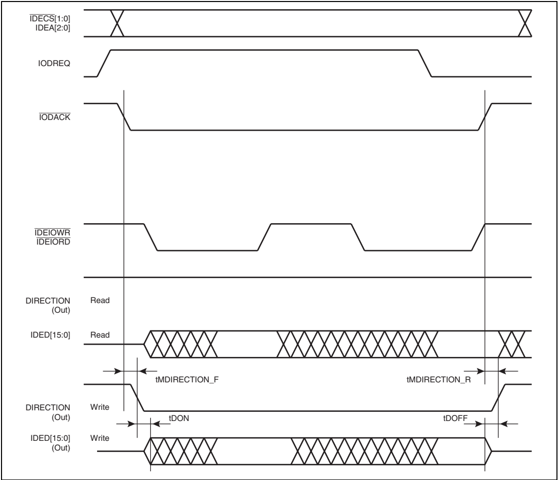
Figure 52.75 Multiword DMA Transfer (DIRECTION)
