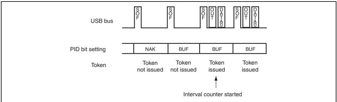
Figure 31.13 Token Issuance when IITV = 0
