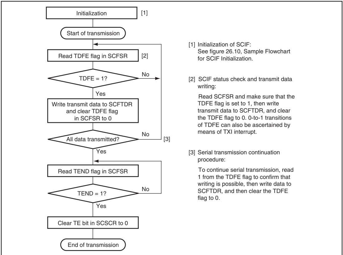
Figure 26.11 Sample Flowchart for Transmitting Serial Data
