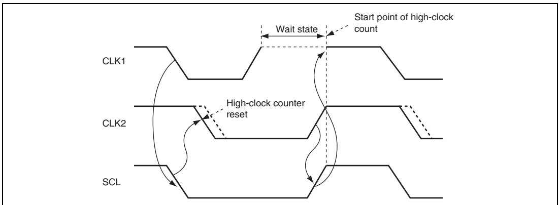
Figure 32.11 Synchronizing SCL Line
