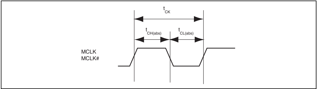
Figure 52.25 Output Clock
