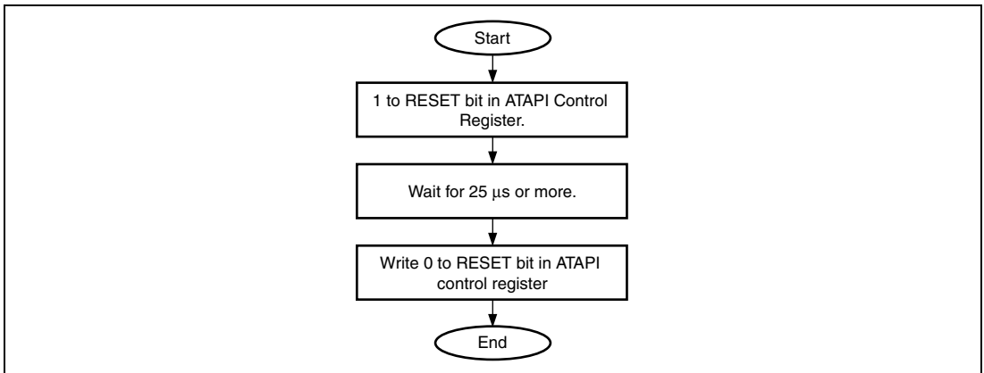
Figure 46.17 Procedure in Hardware Reset for ATAPI Device
