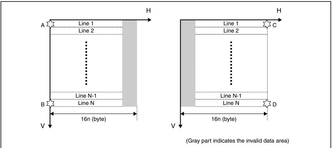
Figure 42.9 Point to be Specified in CHnDAR
