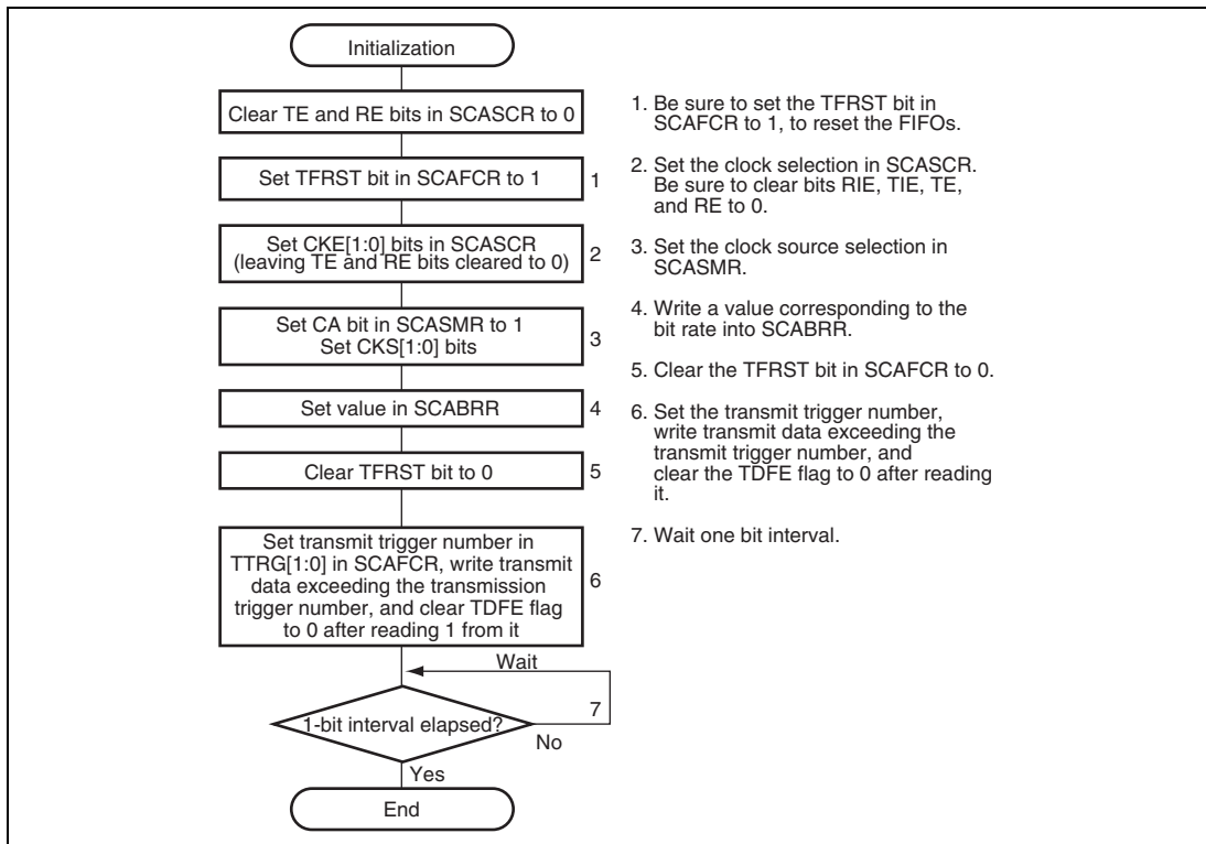
Figure 27.13 Sample SCIFA Initialization Flowchart (1) (Transmission)
