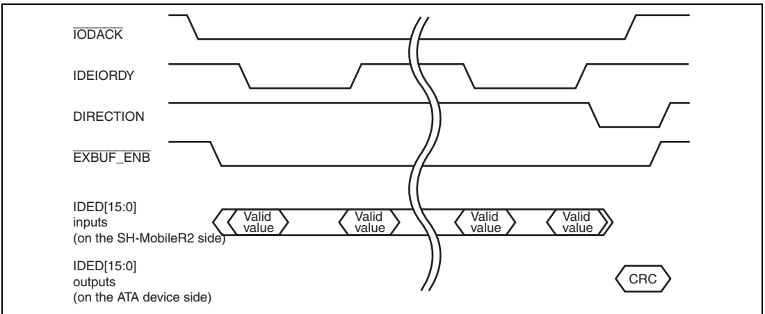
Figure 46.10 Ultra DMA Data-in Burst
