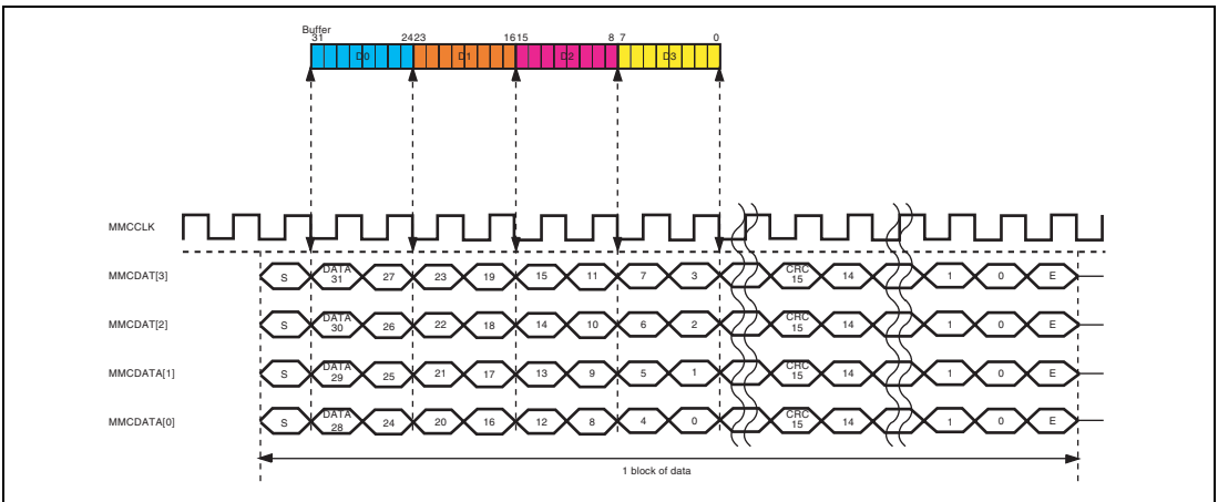
Figure 23.10 Data Format (4-Bit Mode)
