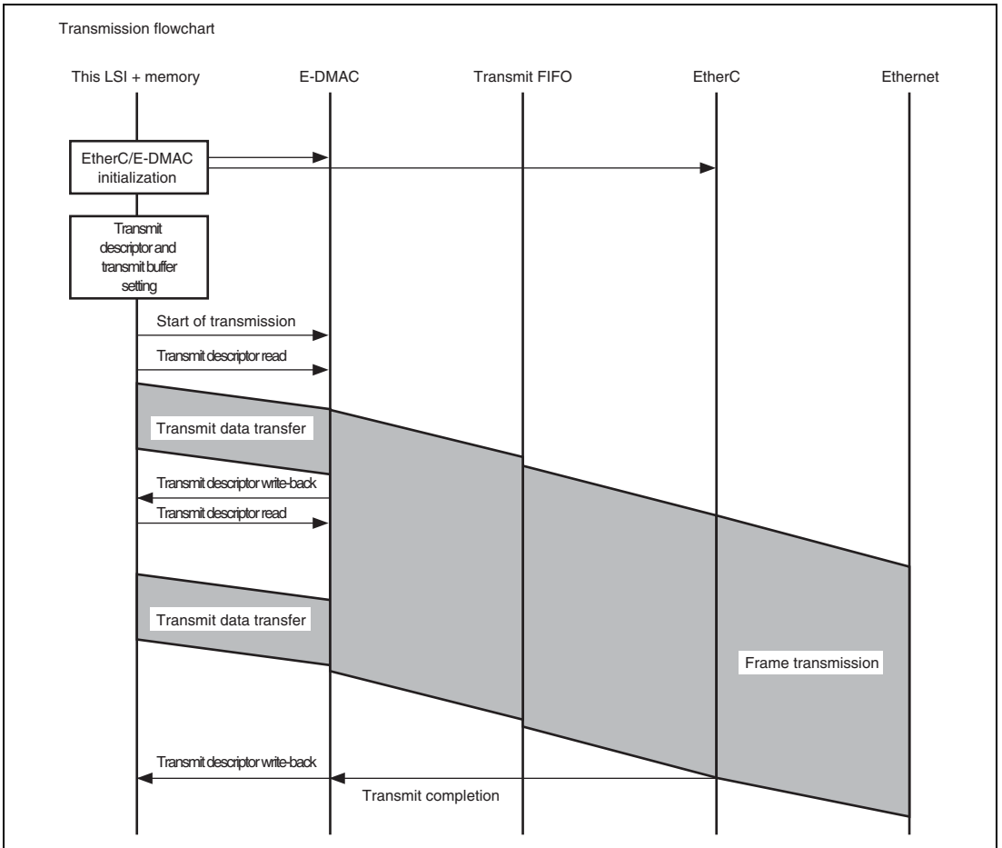
Figure 47.4 Sample Transmission Flowchart (Single-Frame/Two-Descriptor)
