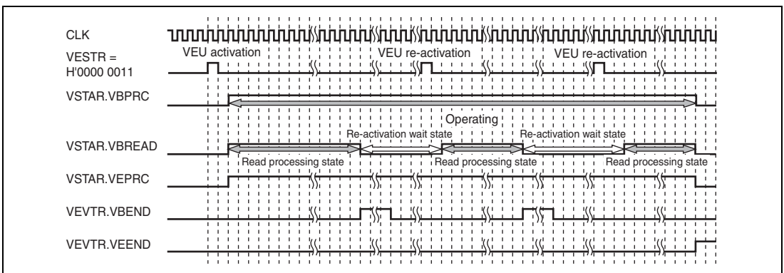
Figure 35.28 VSTAR State Transitions in Bundle Read Mode
