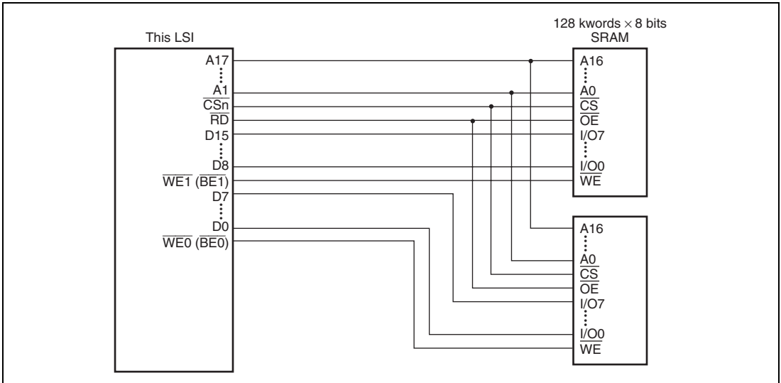
Figure 14.6 Example of 16-Bit Data-Width SRAM Connection
