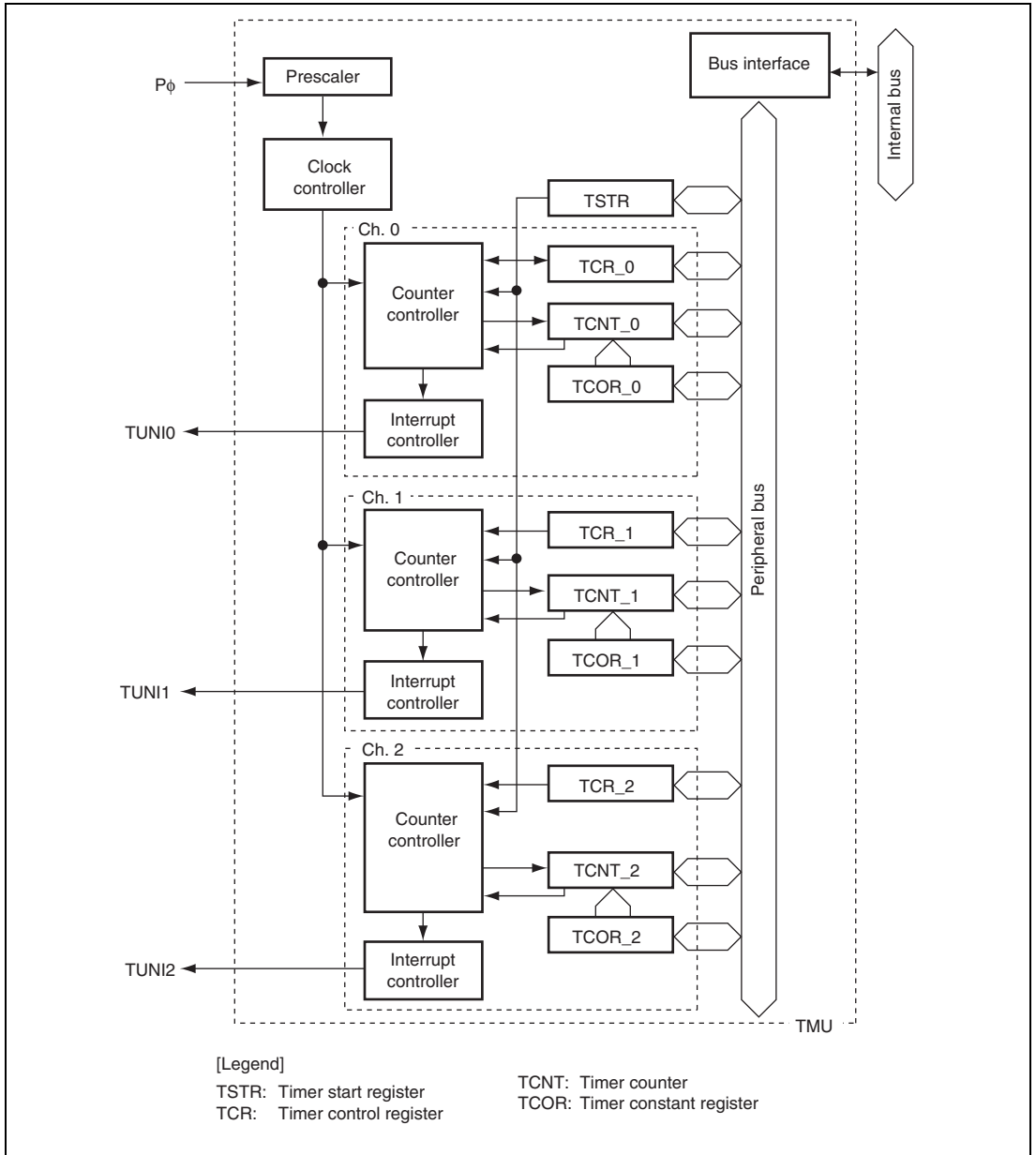
Figure 20.1 Block Diagram of TMU
