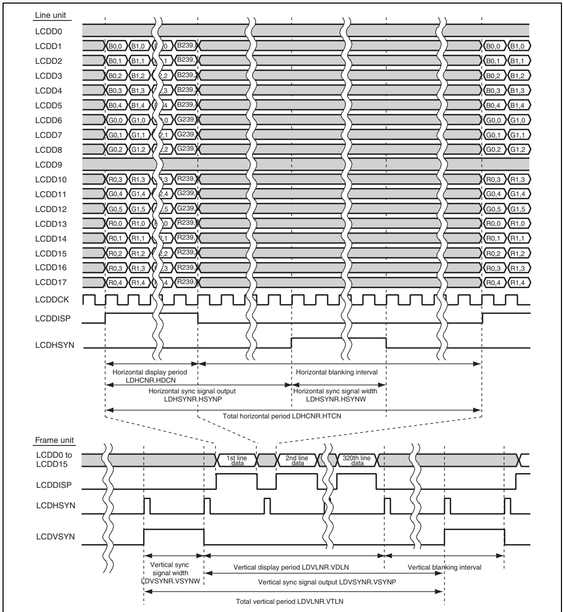
Figure 39.13 Example of Clock and LCD Data Signals (1)
