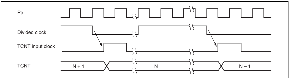
Figure 20.4 Count Timing when Internal Clock is Operating
