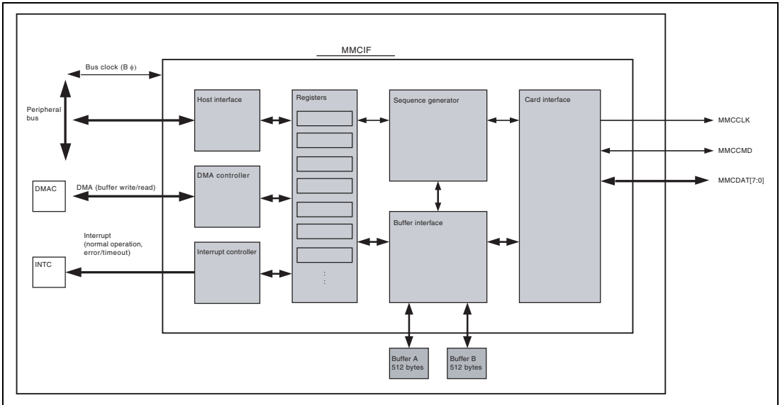
Figure 23.1 Block Diagram of MMCIF
