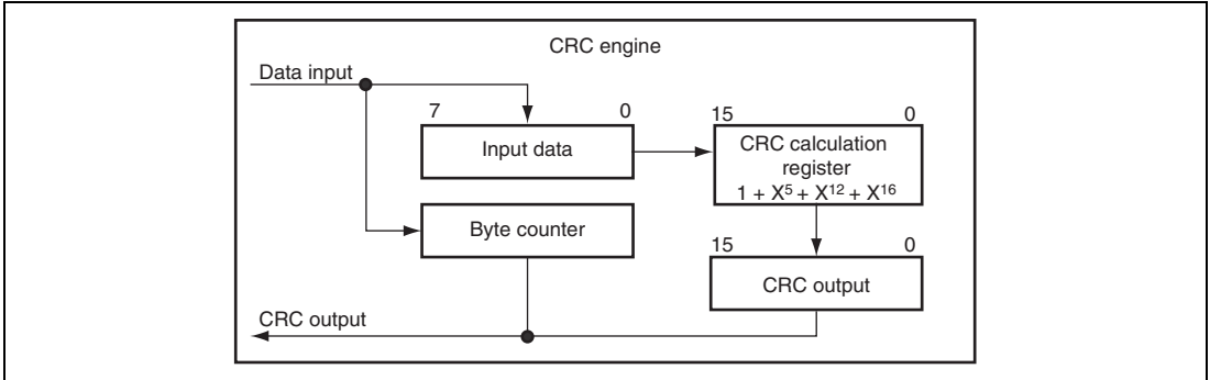
Figure 29.7 CRC Engine Configuration
