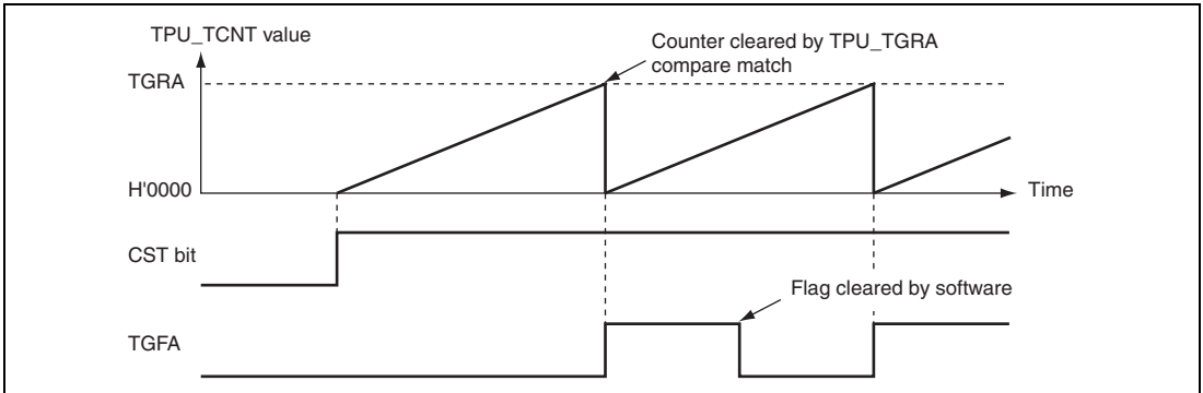
Figure 21.4 Periodic Counter Operation
