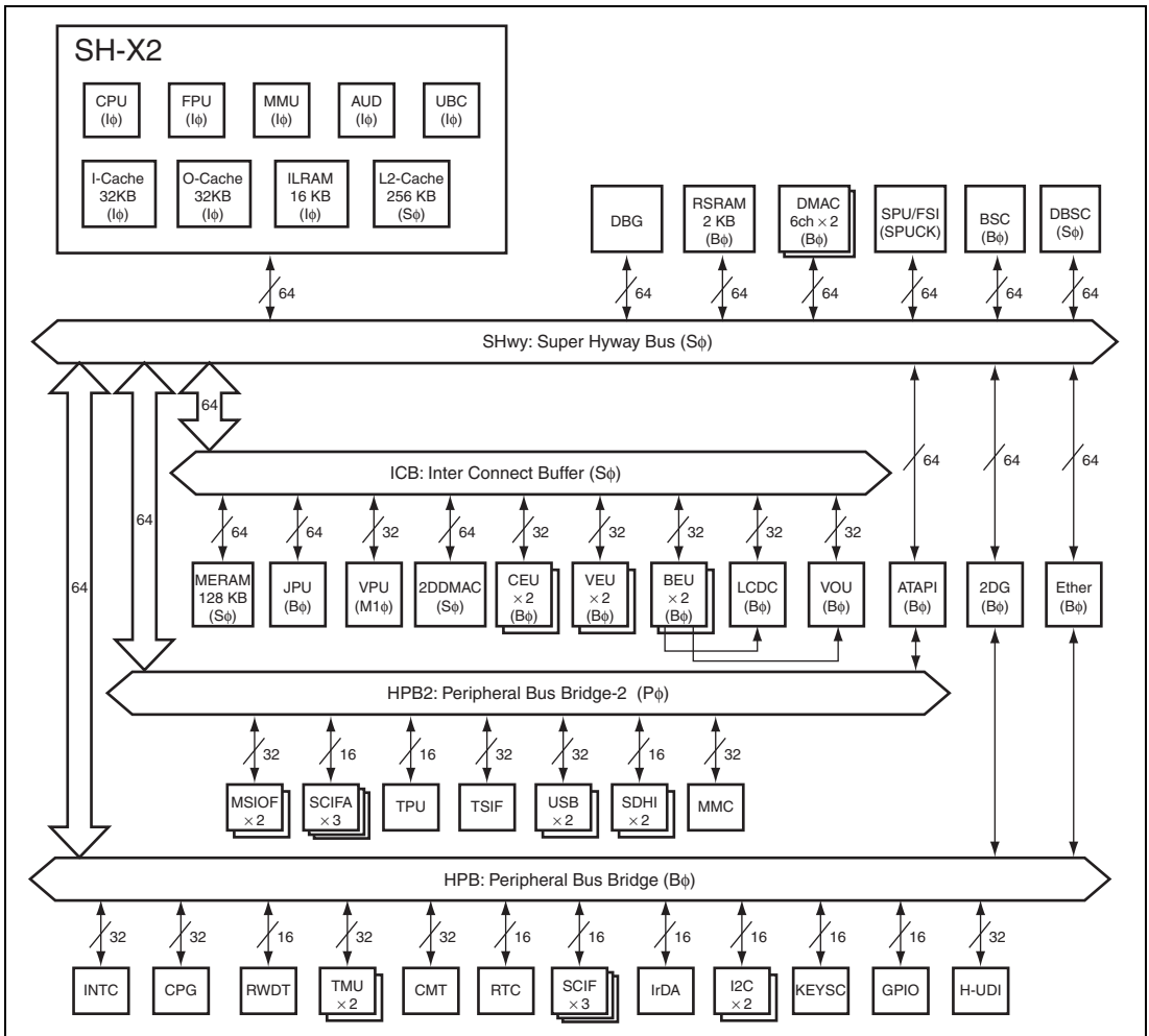
Figure 1.1 SH7724 Block Diagram
