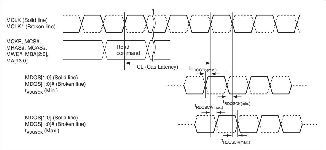
Figure 52.27 DQS Input on Data Read
