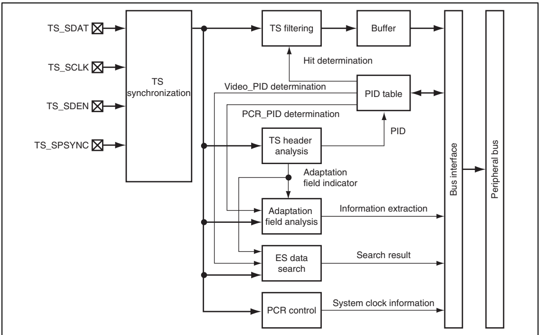
Figure 43.1 TSIF Block Diagram
