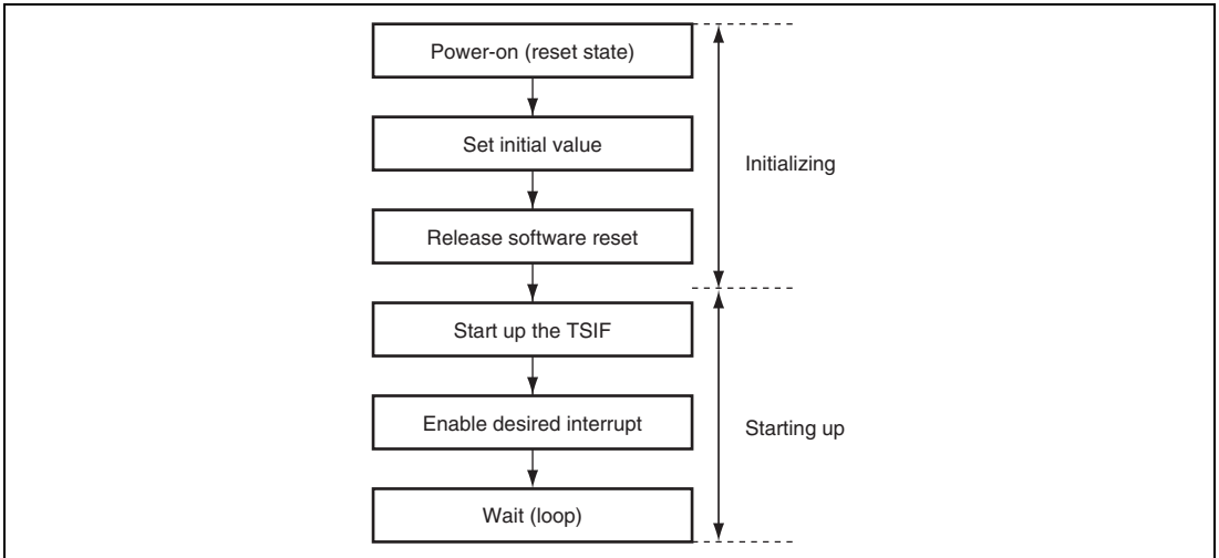
Figure 43.7 TSIF Process Flow
