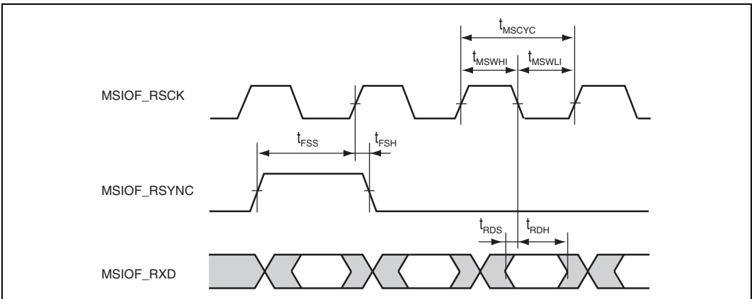
Figure 52.43 MSIOF Transmission/Reception Timing (Slave Mode)
