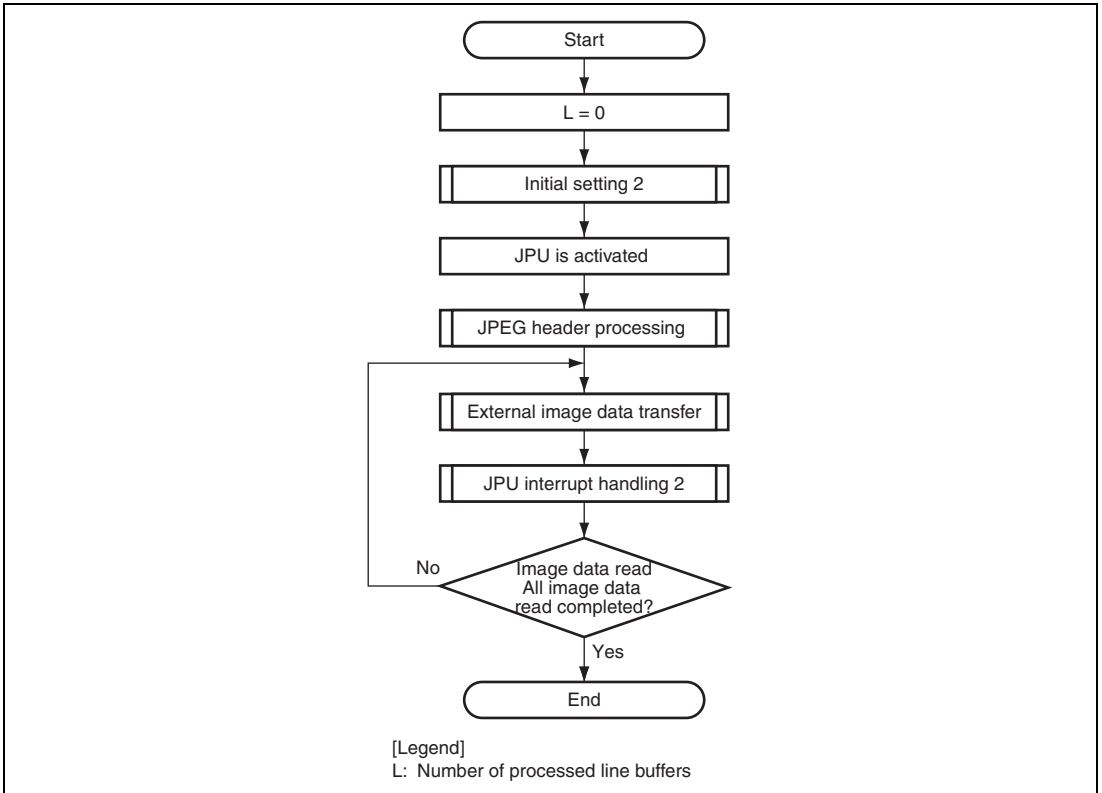
Figure 37.5 Flow of Encoding in Line Buffer Mode
