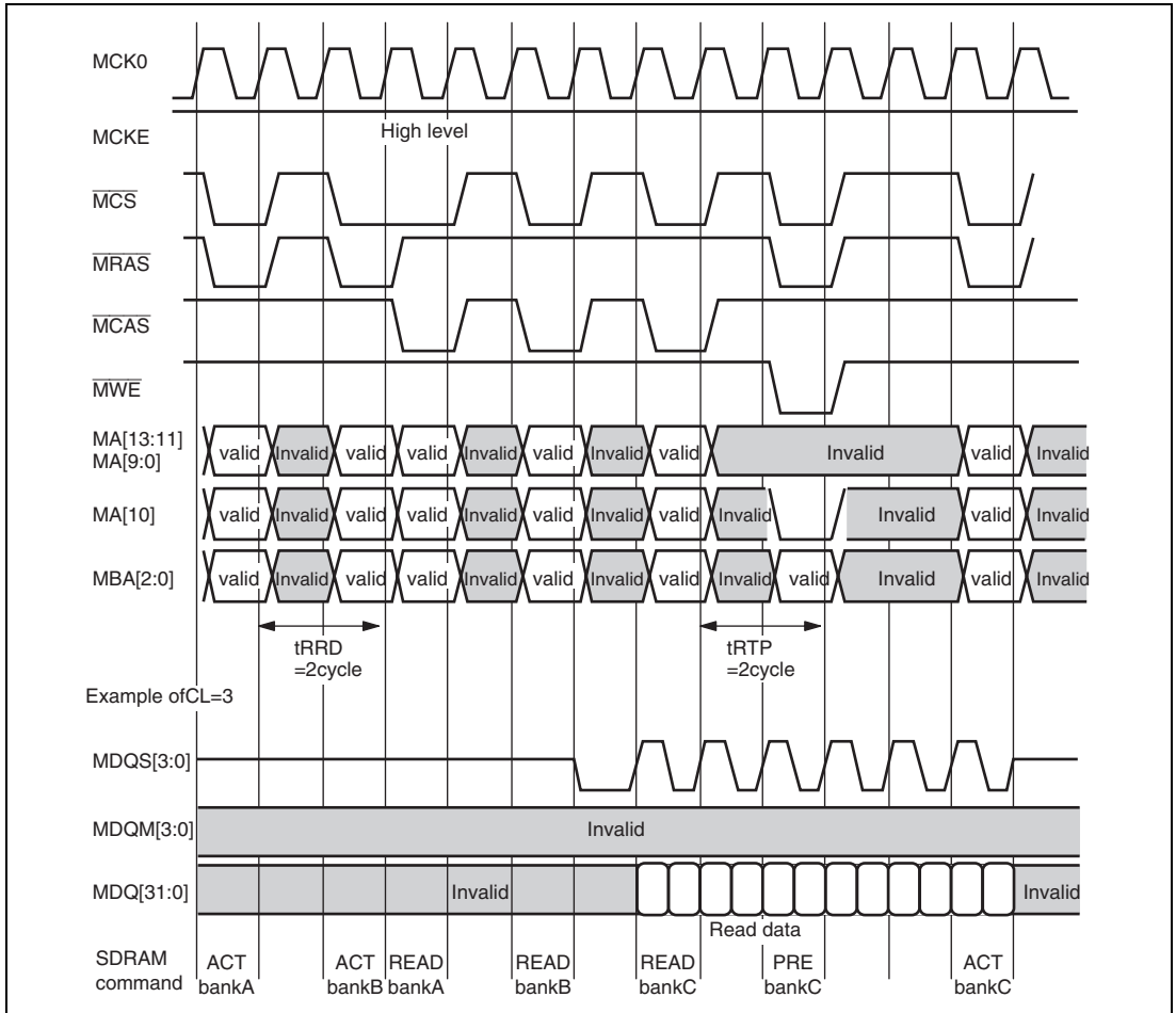
Figure 15.14 t_{RRD} and t_{RTP}
