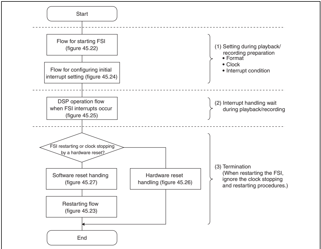
Figure 45.21 Entire FSI Operation and Each Operation Flow
