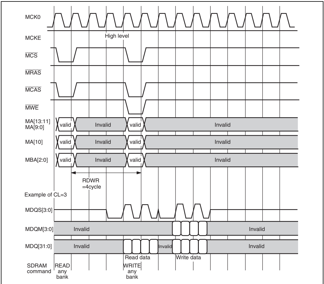
Figure 15.17 READ-WRITE Minimum Time
