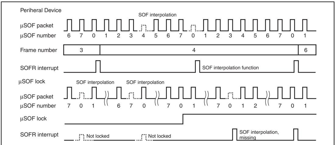
Figure 31.9 Example of SOFR Interrupt Output Timing
