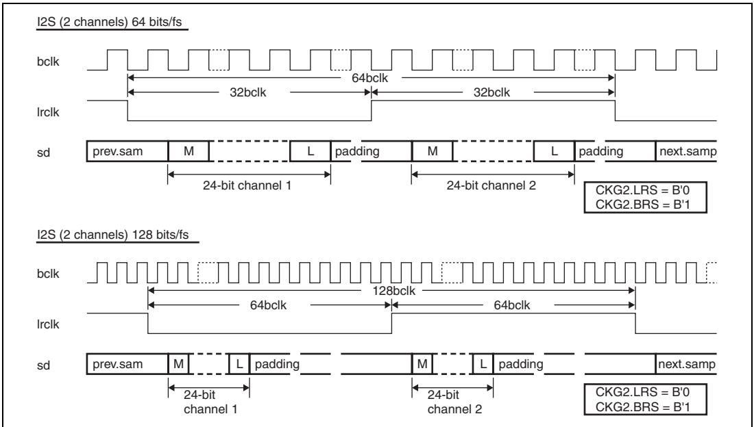
Figure 45.18 I2S Formats
