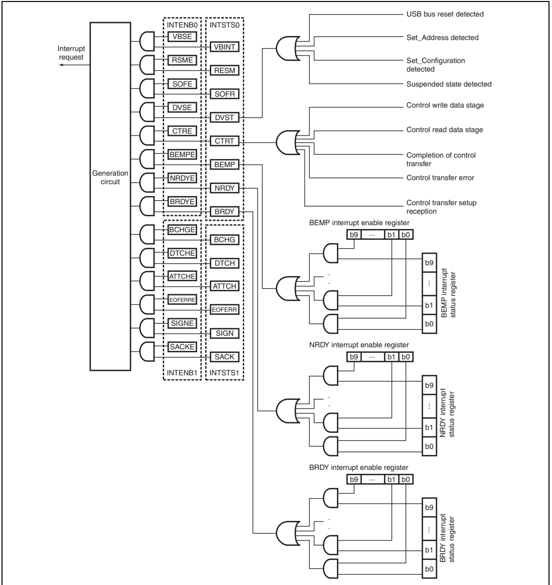
Figure 31.3 Items Relating to Interrupts
