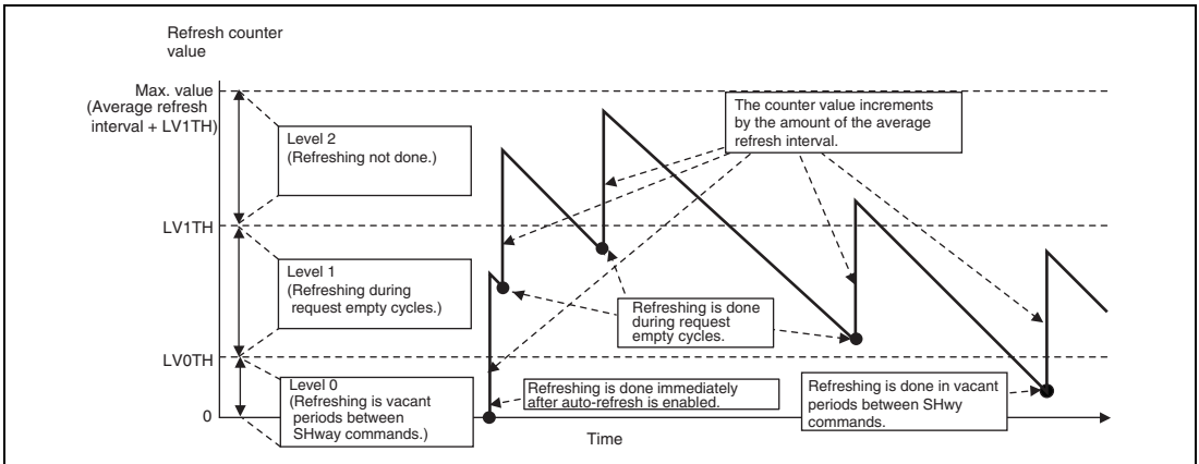
Figure 15.6 Relation between Auto-Refresh Operation and Threshold Values
