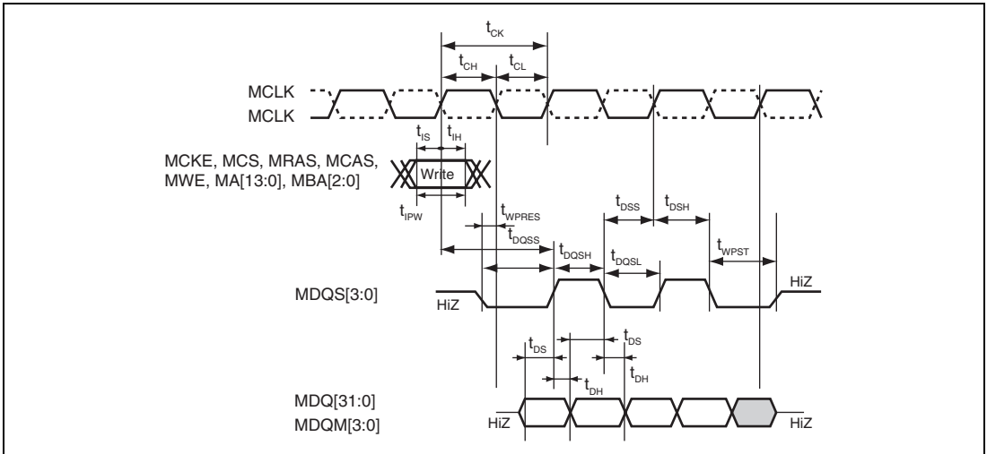
Figure 52.34 Mobile-DDR-SDRAM Output Timing (Write)
