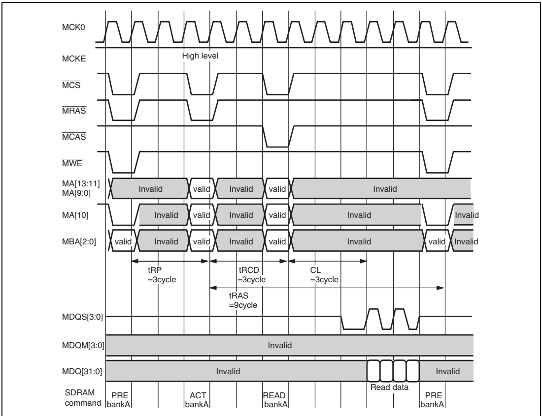
Figure 15.13 tRP, tRCD, CL, and tRAS
