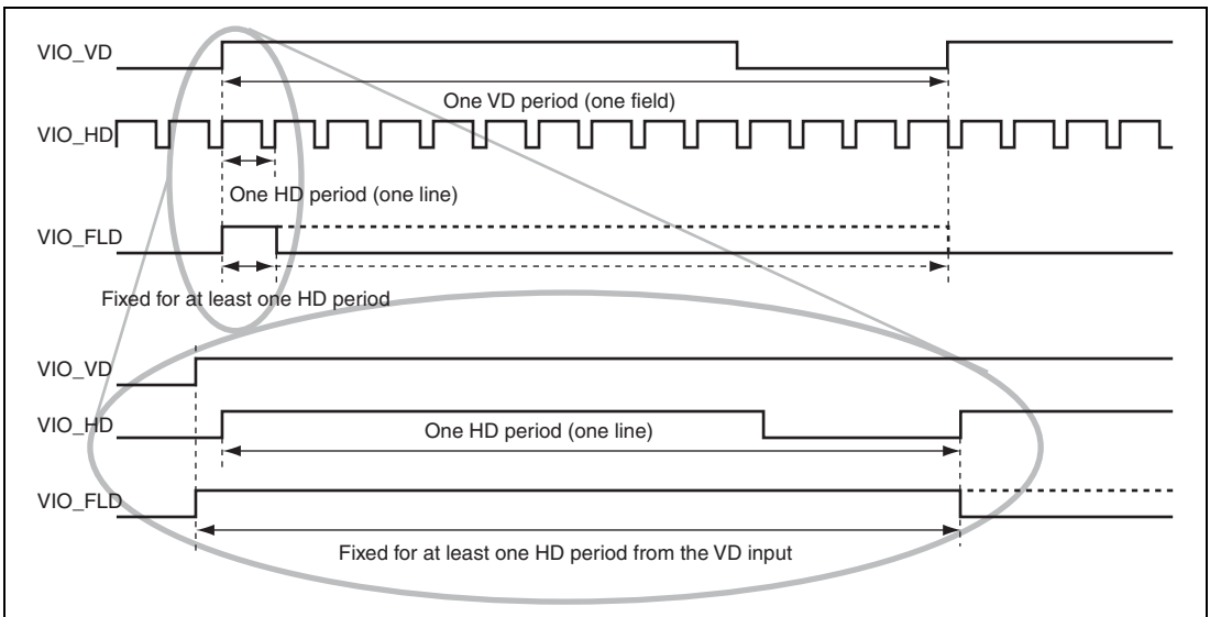
Figure 34.4 One Field Timing
