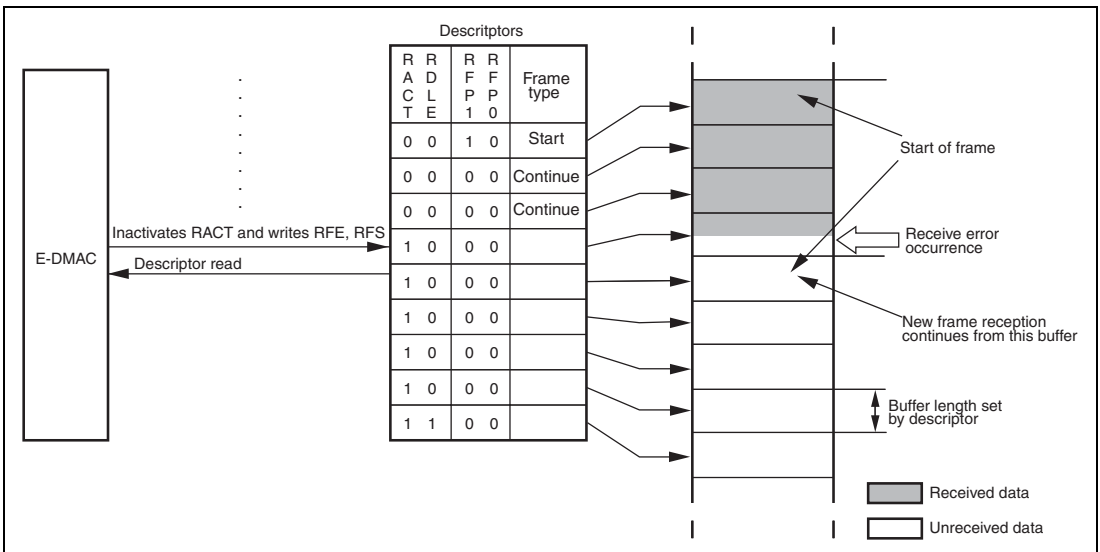
Figure 47.6 E-DMAC Operation after Receive Error
