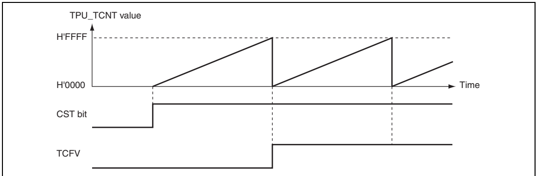
Figure 21.3 Free-Running Counter Operation
