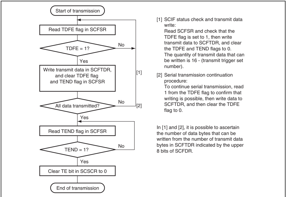
Figure 26.4 Sample Flowchart for Transmitting Serial Data
