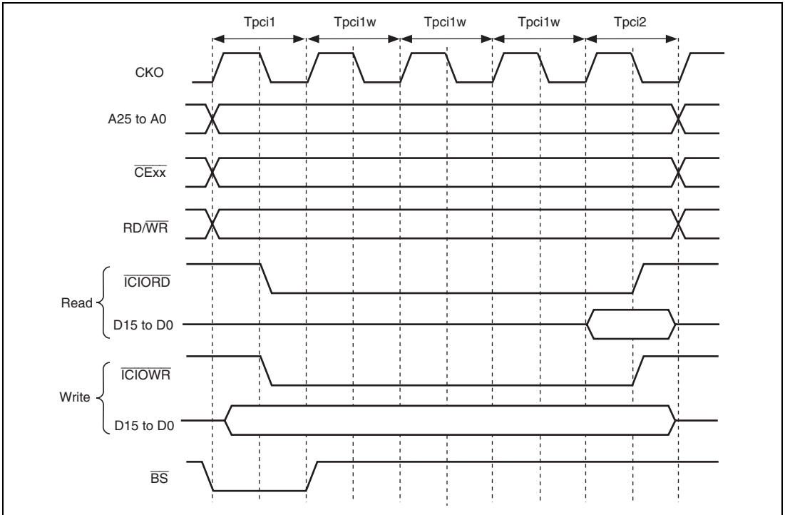
Figure 14.21 Basic Timing of PCMCIA I/O Card Interface
