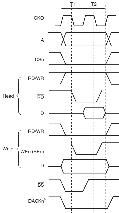
Figure 14.2 Normal Space Basic Access Timing (Access Wait 0)
