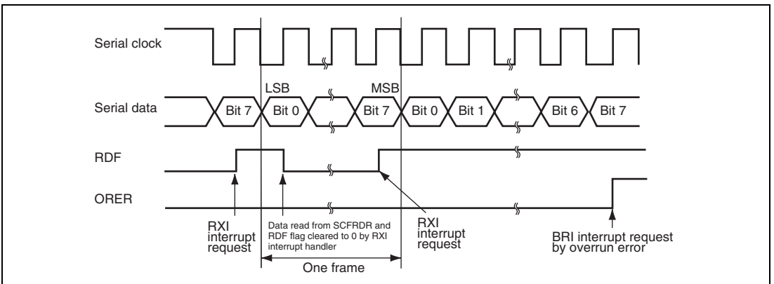
Figure 26.15 Example of SCIF Receive Operation
