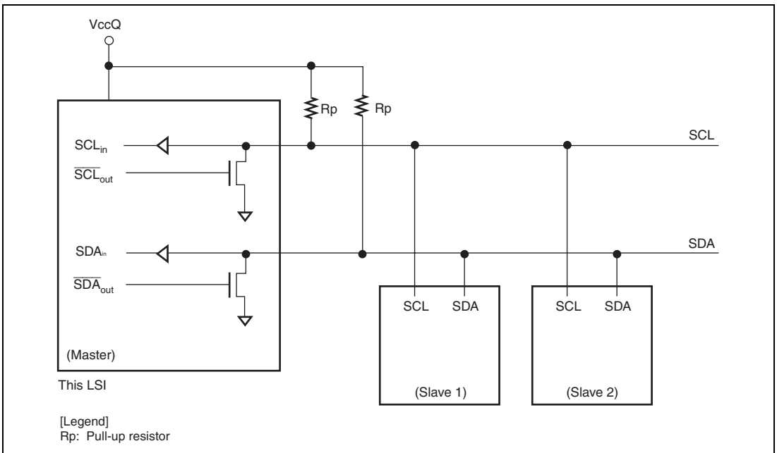
Figure 32.2 I 2 C Bus Interface Connections
