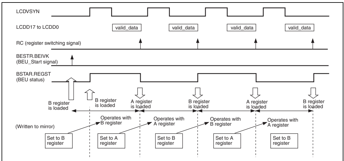
Figure 36.20 Register Switching in LCDC-Linked Operation
