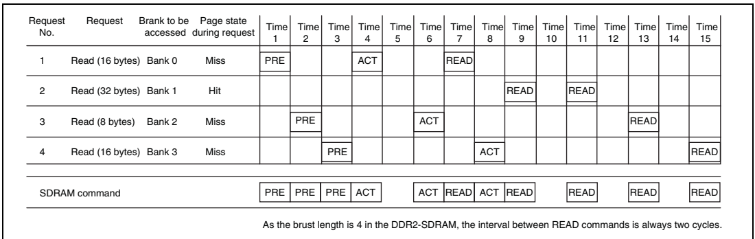
Figure 15.5 Example of Preceding Precharge/Activate Processing
