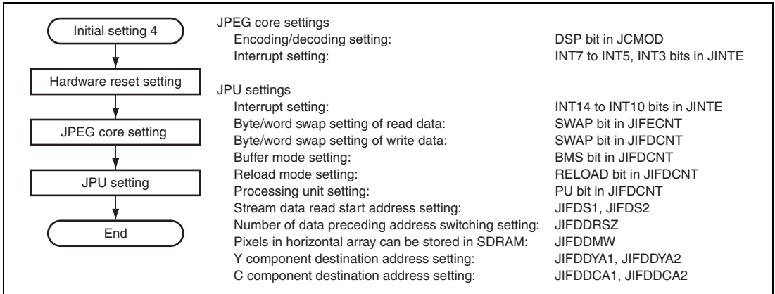
Figure 37.19 Flow of Initial Setting 4
