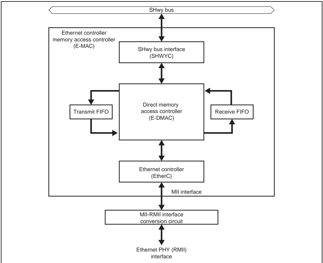
Figure 47.1 Block Diagram of Ethernet MAC Controller
