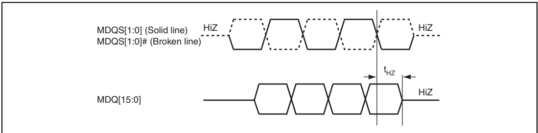
Figure 52.33 Time Required for DQ Output to enter Hi-Z state (Write)
