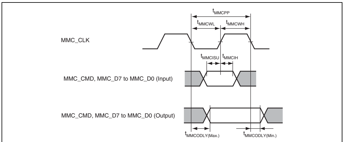
Figure 52.86 MMCIF Module Signal Timing
