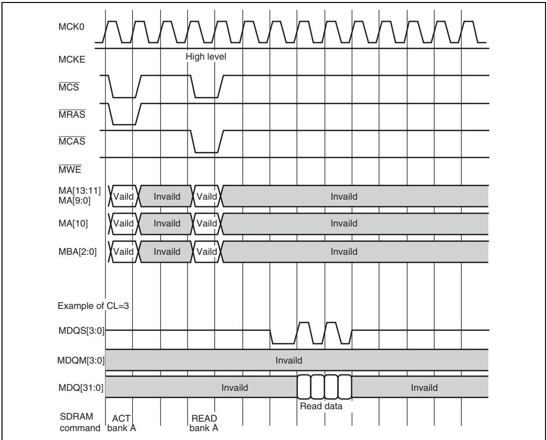
Figure 15.7 Waveforms for 1-/2-/4-/8-/16-Byte Reading (When the Bus Width Is Set to 32 Bits)
