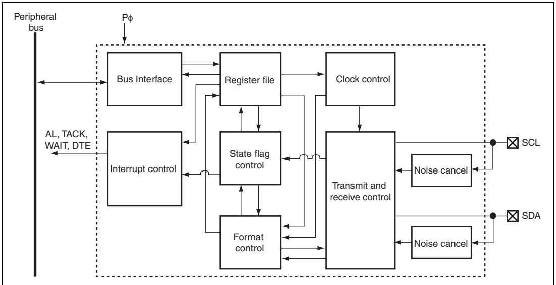
Figure 32.1 Block Diagram of I 2 C Bus Interface
