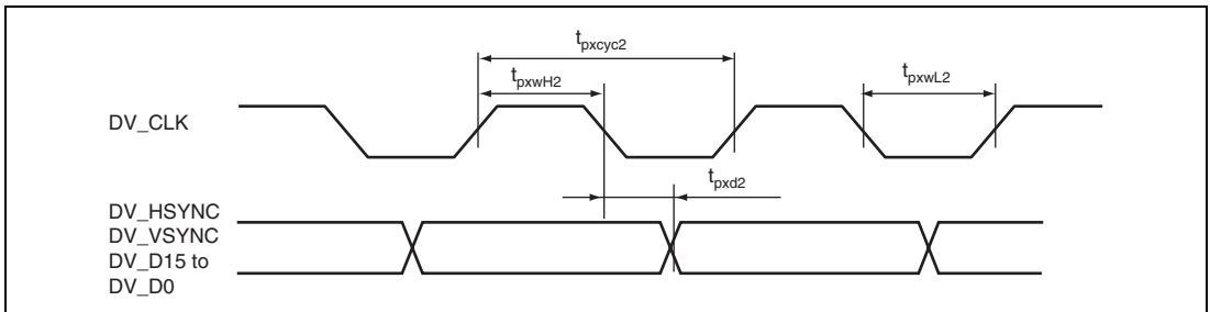
Figure 52.54 VOUModule AC Characteristics (VOUCR.CKPL = 1)
