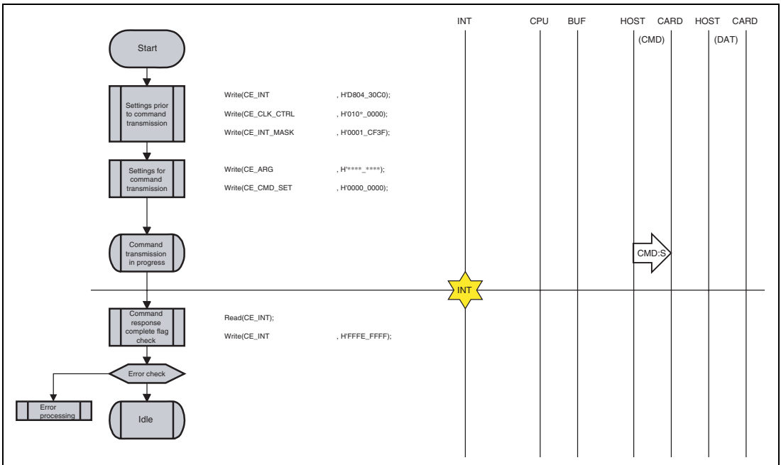
Figure 23.13 Command Transmission (CMD0)
