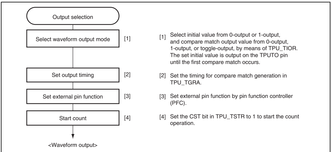
Figure 21.5 Example of Setting Procedure for Waveform Output by Compare Match
