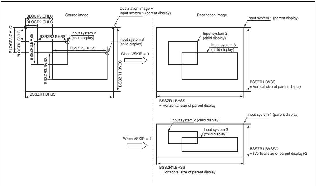
Figure 36.5 Comparison of Destination Displays with Skipping at Reading Enabled and Disabled
