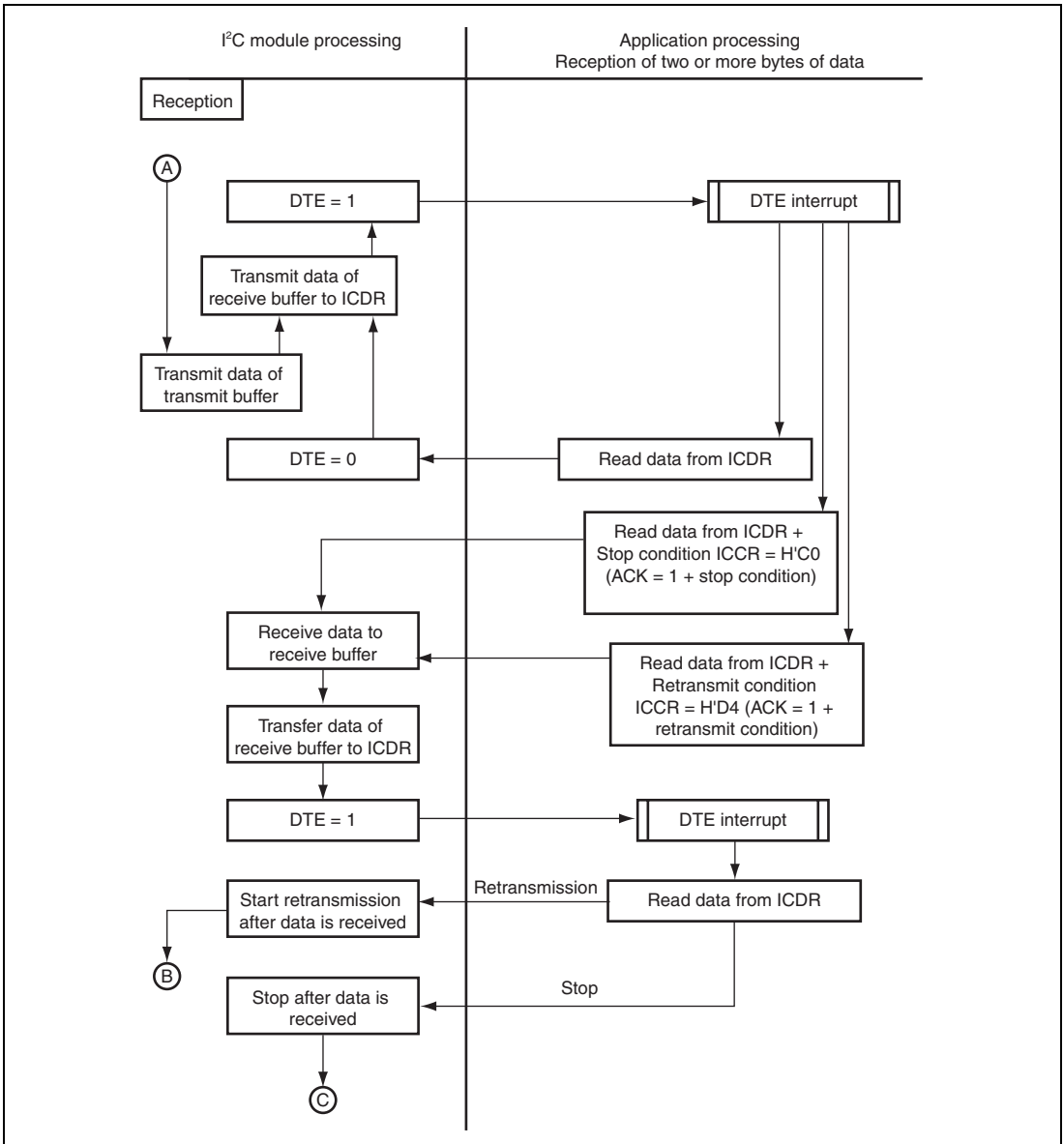
Figure 32.9 I 2 C Transmission Sequence (in Receive Mode of Two or More Bytes of Data)
