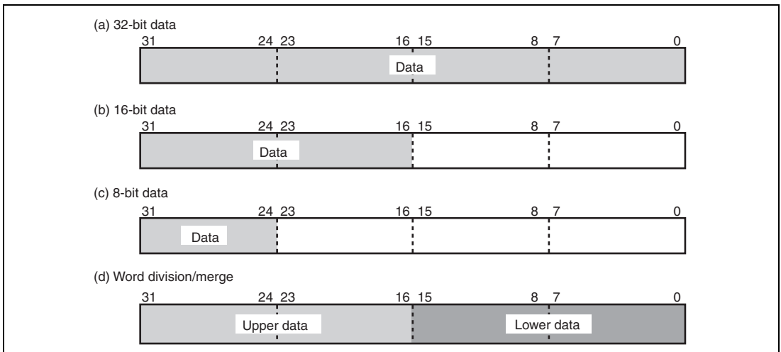
Figure 25.9 Transmit/Receive Data Bit Alignment
