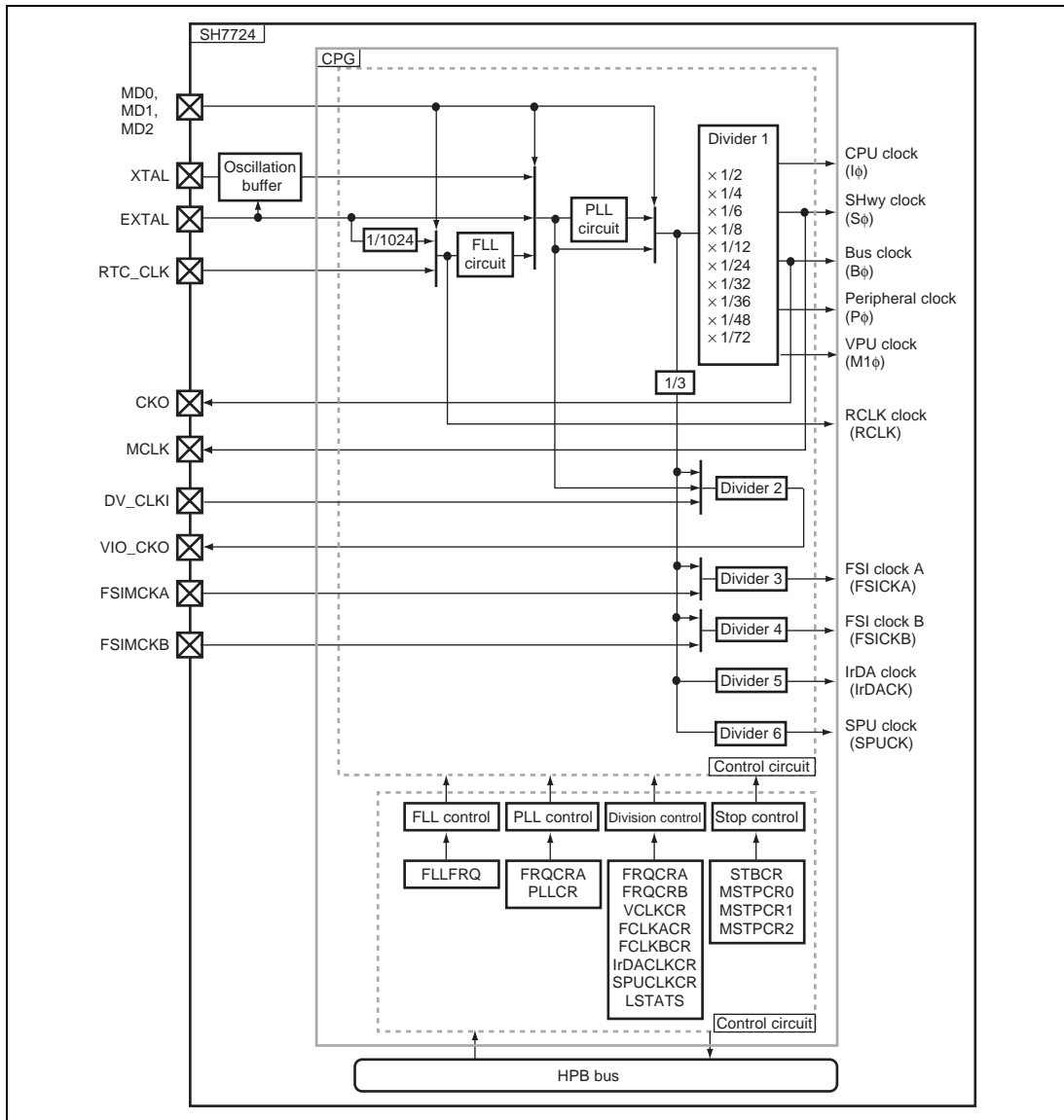
Figure 17.1 Block Diagram of CPG
