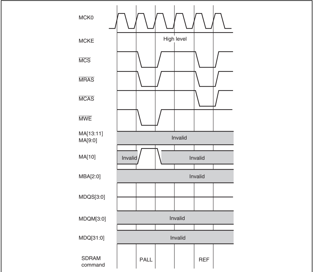
Figure 15.11 Auto-Refresh Operation
