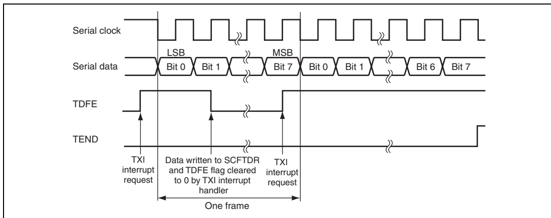
Figure 26.12 Example of SCIF Transmit Operation
