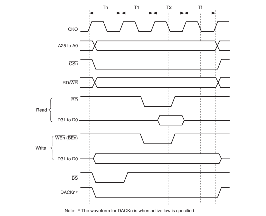
Figure 14.10 \overline{CSn} Assert Period Extension
