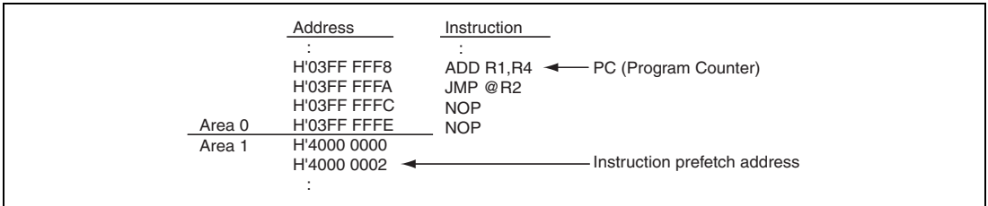
Figure B.1 Instruction Prefetch
