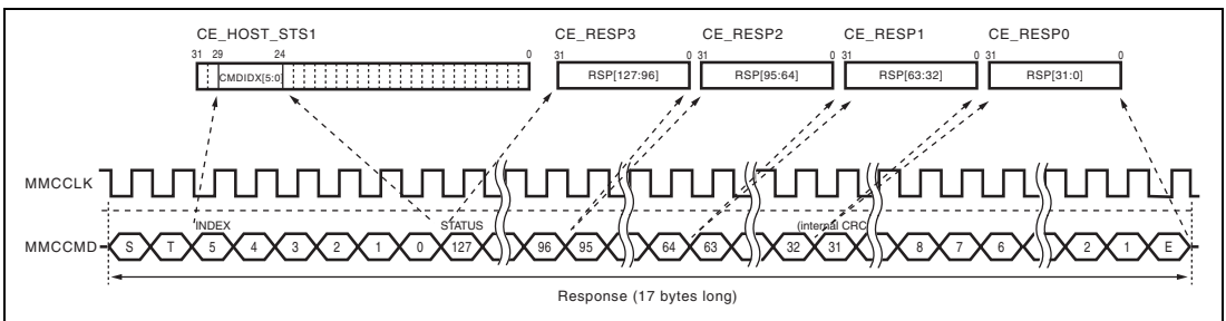
Figure 23.4 Format of 17-Byte Response (R2)
