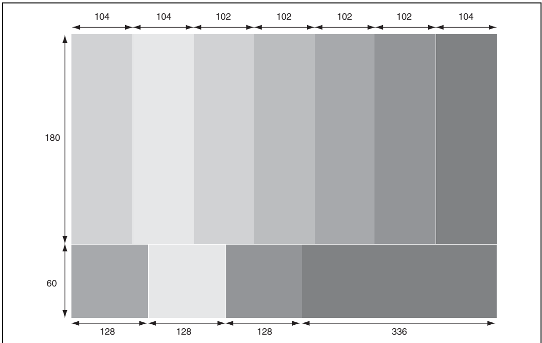
Figure 40.2 Output Color Bar Pattern
