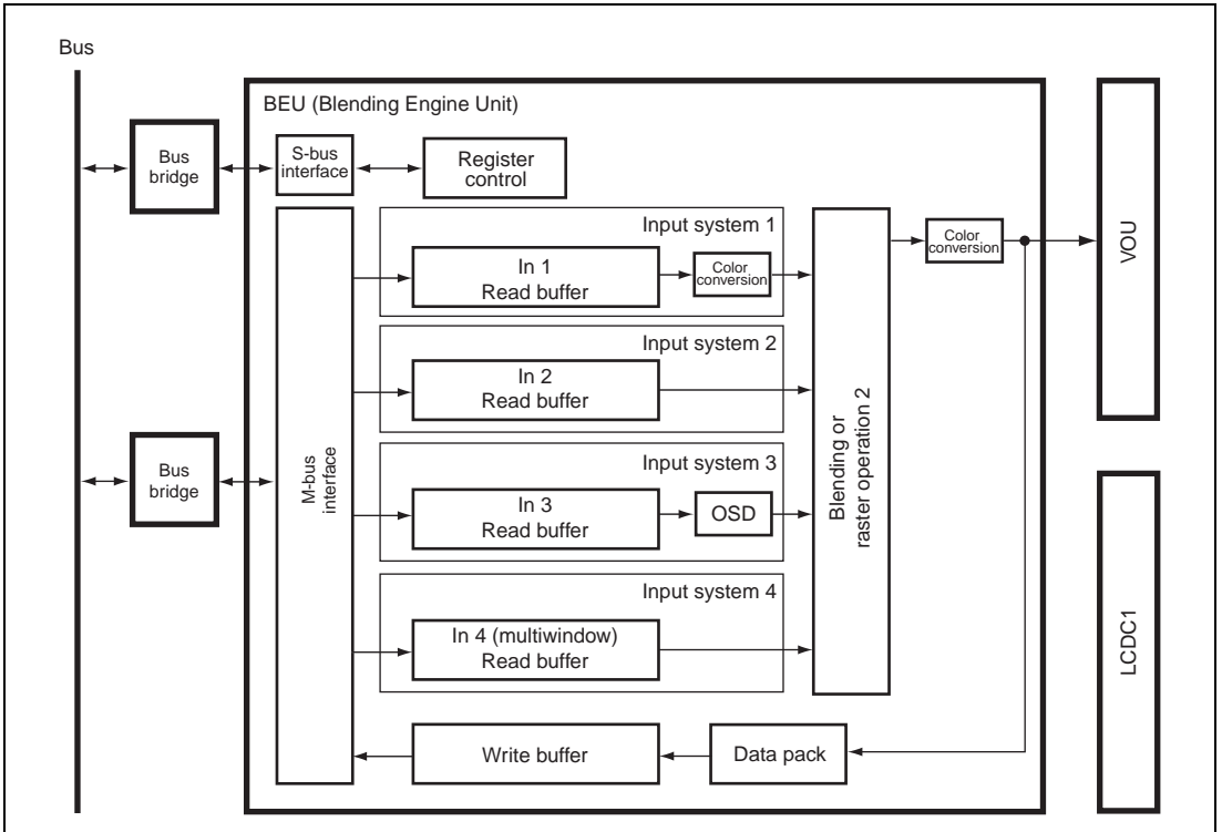
Figure 36.1 Block Diagram of BEU
