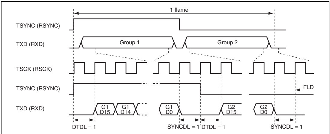
Figure 25.6 Synchronization Timing in L/R Synchronization Mode
