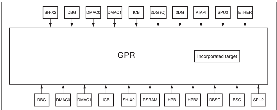
Figure 12.1 Connection of SuperHyway Packet Router (GPR)
