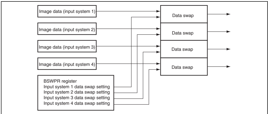
Figure 36.16 Data Swap Configuration when MODSEL = 1
