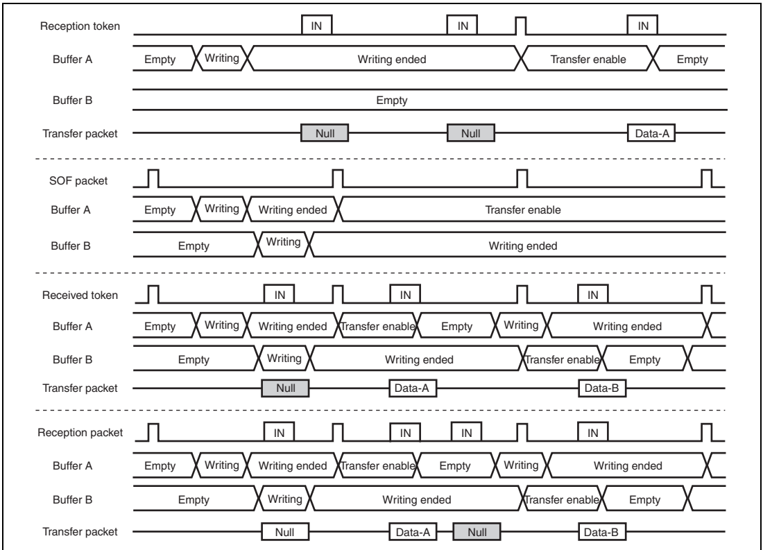
Figure 31.17 Example of Data Setup Function Operation
