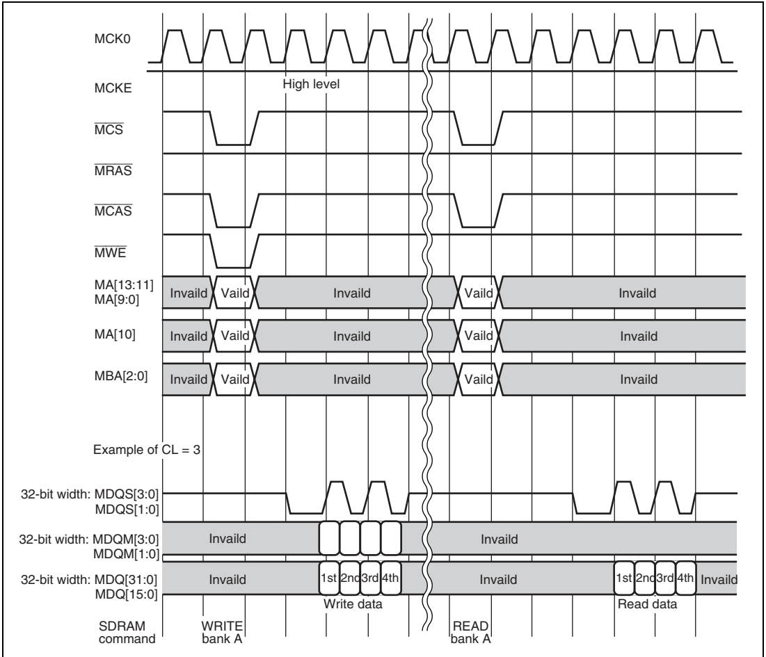
Figure 15.2 Burst Access Operation
