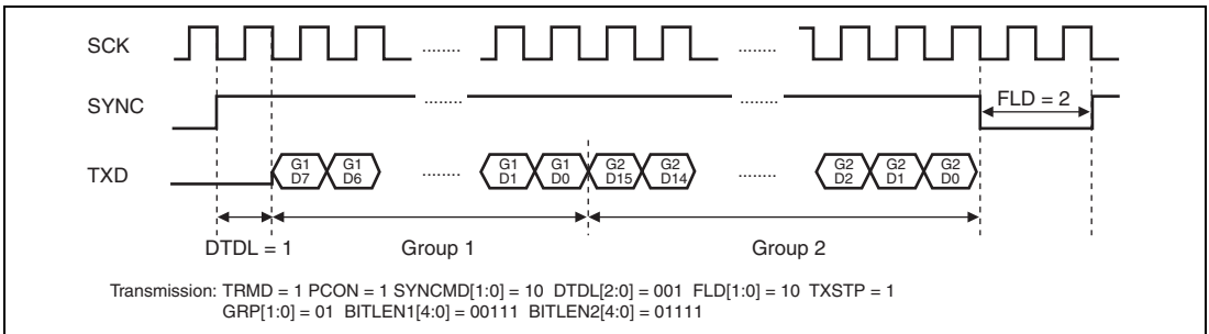
Figure 25.17 Transmit Timing ( \mu -WIRE transmit)
