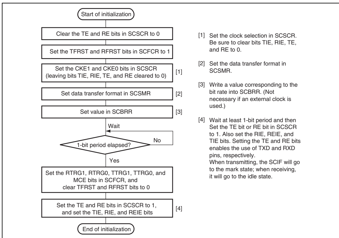
Figure 26.3 Sample Flowchart for SCIF Initialization
