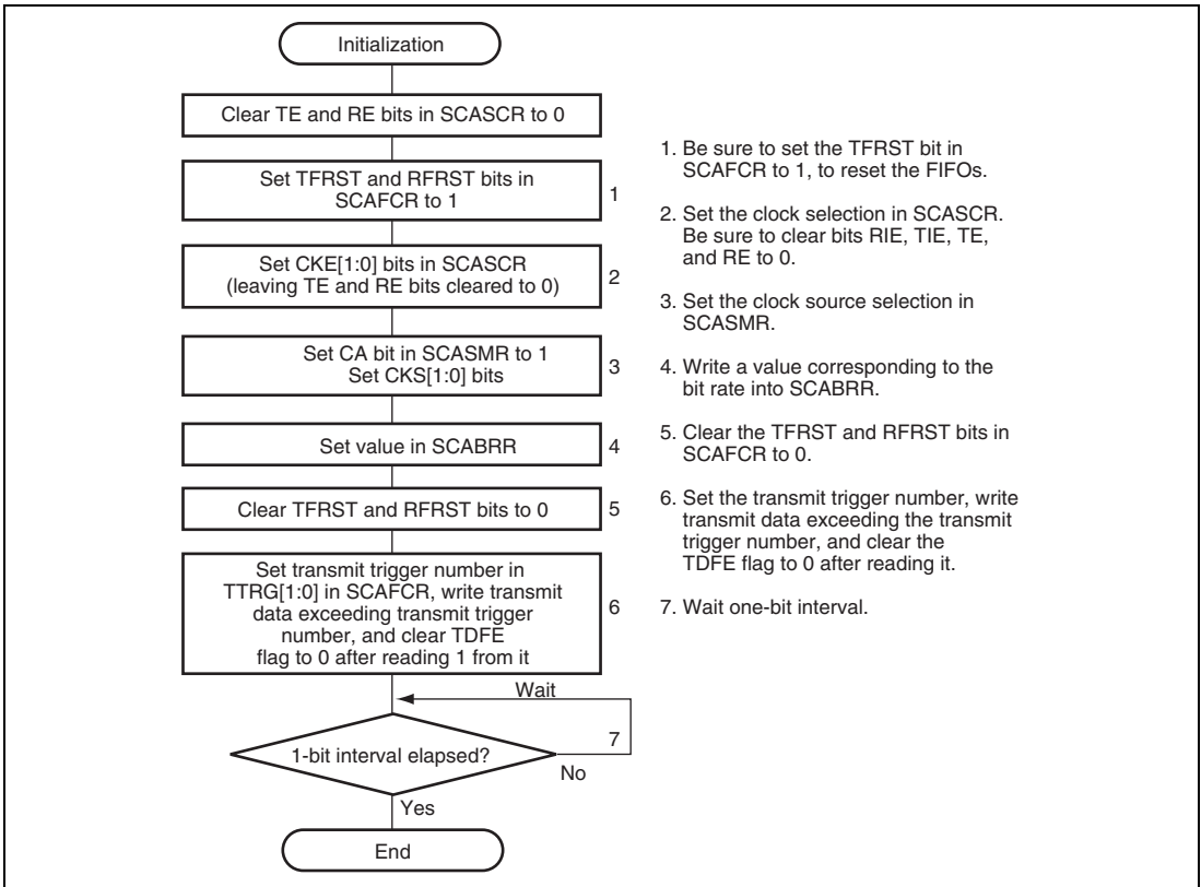
Figure 27.15 Sample SCIFA Initialization Flowchart (3) (Simultaneous Transmission and Reception)
