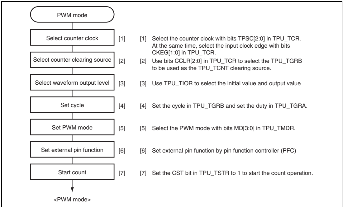
Figure 21.11 Example of PWM Mode Setting Procedure
