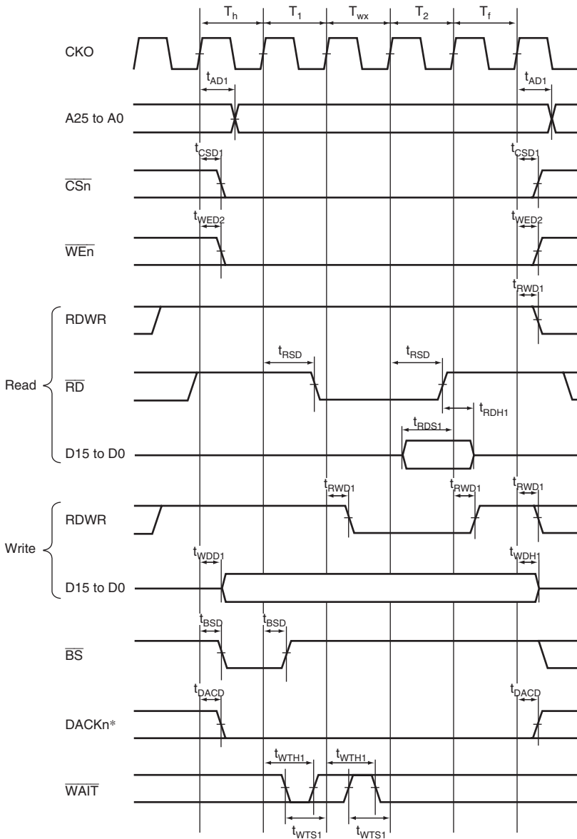
Figure 52.16 SRAM Bus Cycle with Byte Selection (SW = 1 Cycle, HW = 1 Cycle, Asynchronous External Wait 1, BAS = 1 (Write Cycle WE Control))
