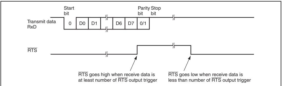
Figure 27.11 Example of \overline{\text{RTS}} Control Operation
