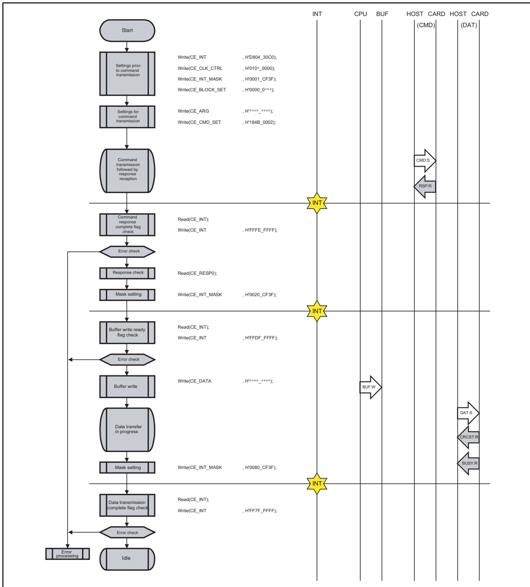
Figure 23.18 Single-Block Write (CMD24)
