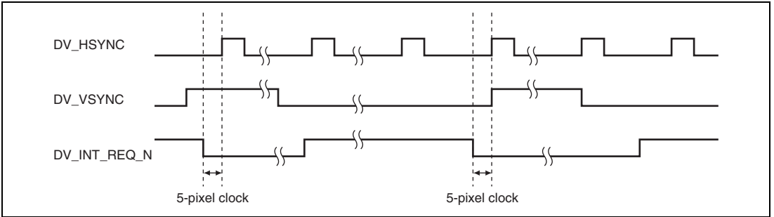
Figure 40.10 Interrupt Occurrence Timing
