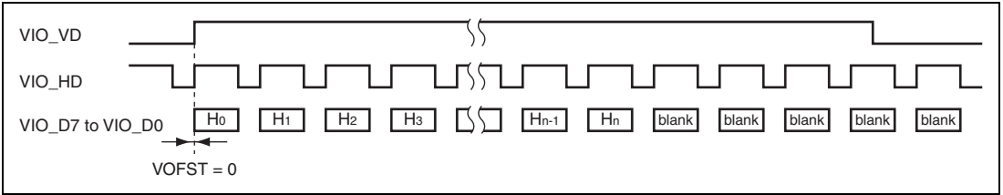
Figure 34.17 Timing when VD is Data Enable Signal
