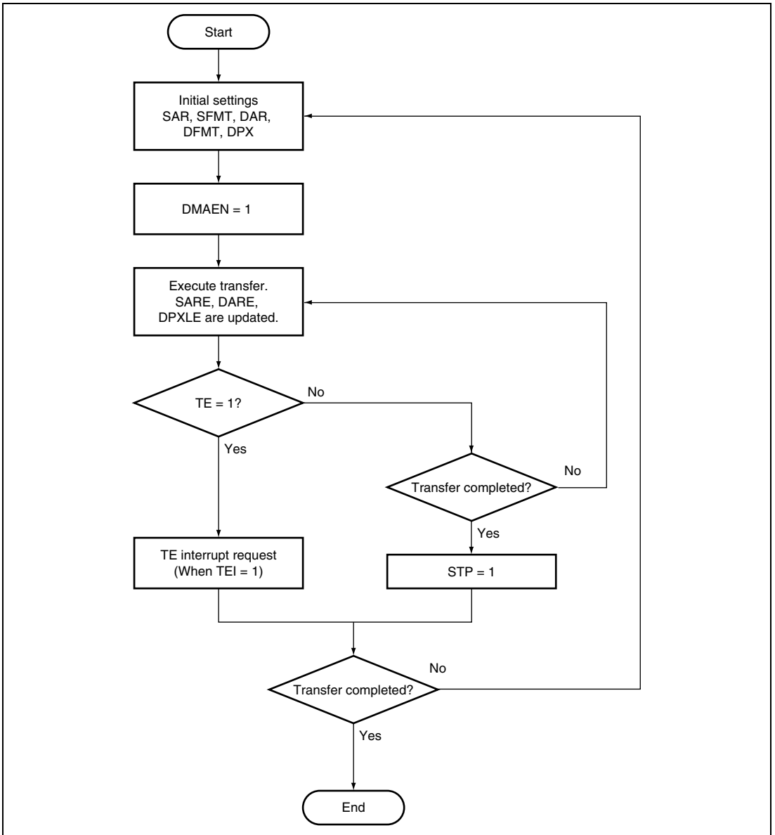
Figure 42.11 Flowchart of Transfer Using 2D-DMAC
