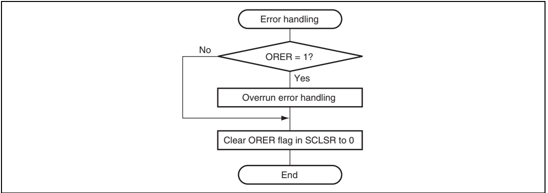
Figure 26.14 Sample Flowchart for Receiving Serial Data (2)
