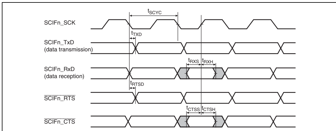
Figure 52.45 SCIF Module Signal Timing
