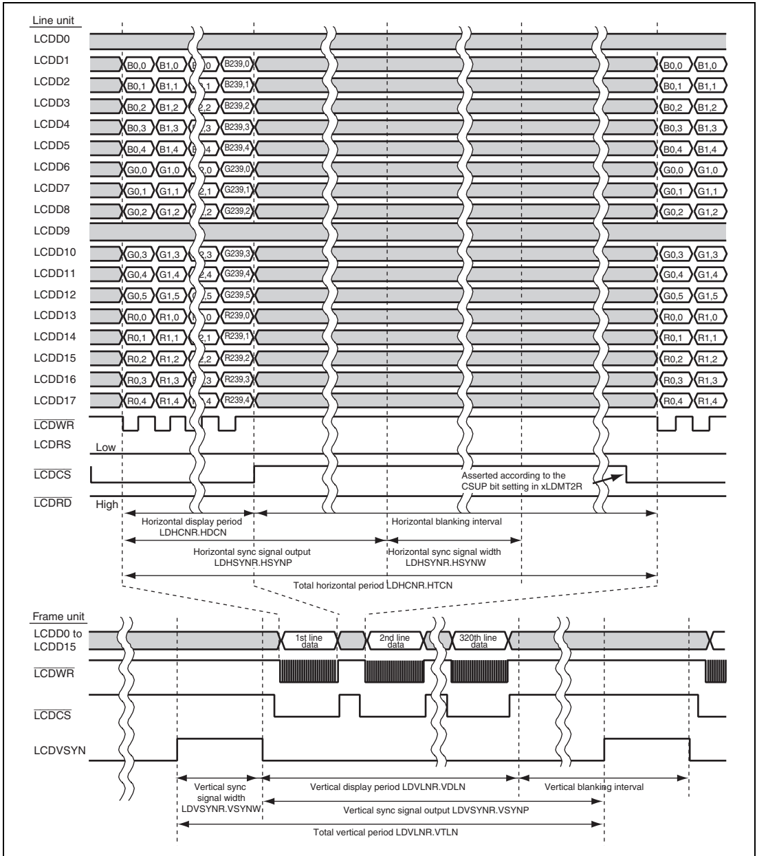
Figure 39.14 Example of Clock and LCD Data Signals (2)
