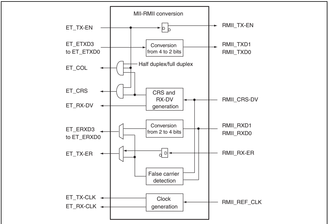
Figure 47.15 Block Diagram of MII-RMII Conversion
