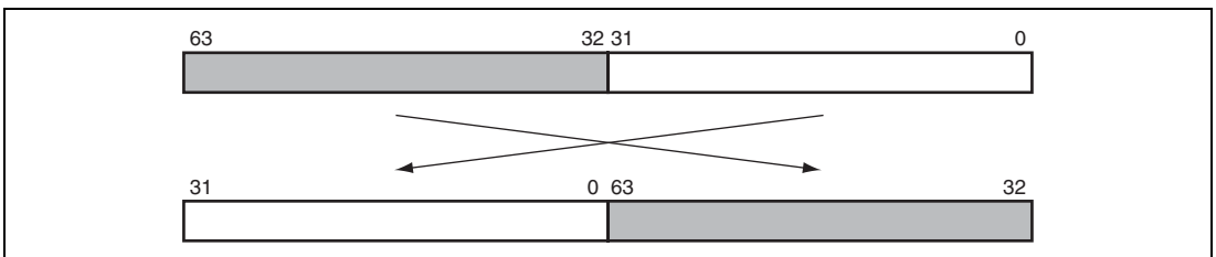
Figure 42.3 Data Before and After Longword Swapping
