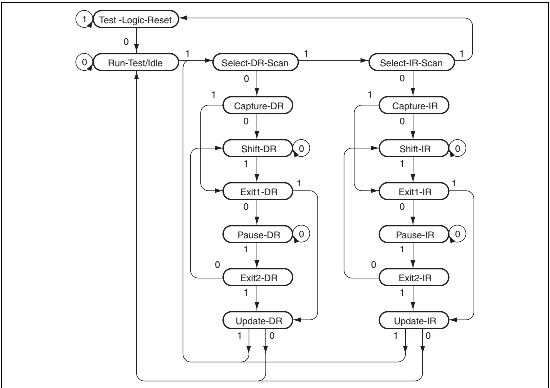
Figure 50.2 TAP Controller State Transitions
