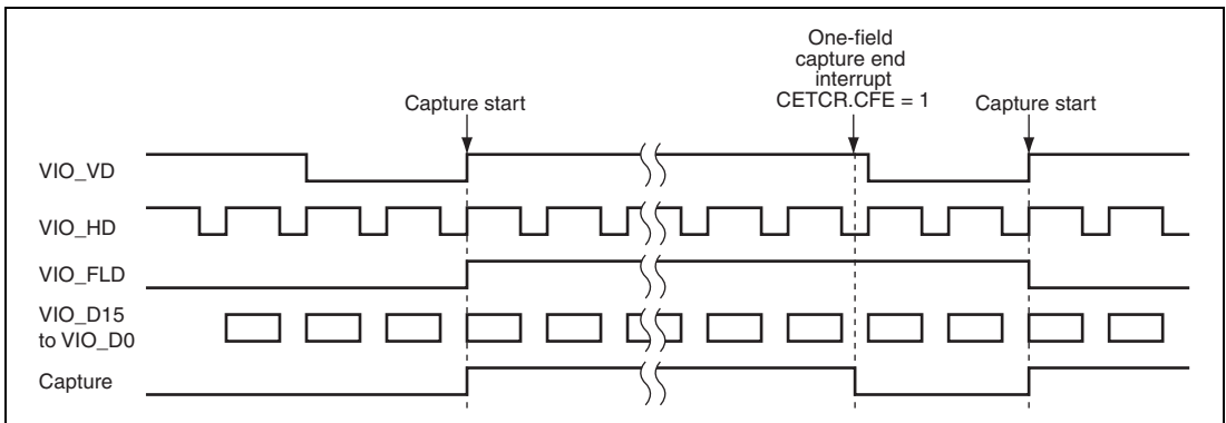
Figure 34.47 CFE Generation Timing
