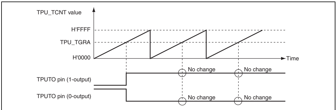
Figure 21.6 Example of 0-Output/1-Output Operation
