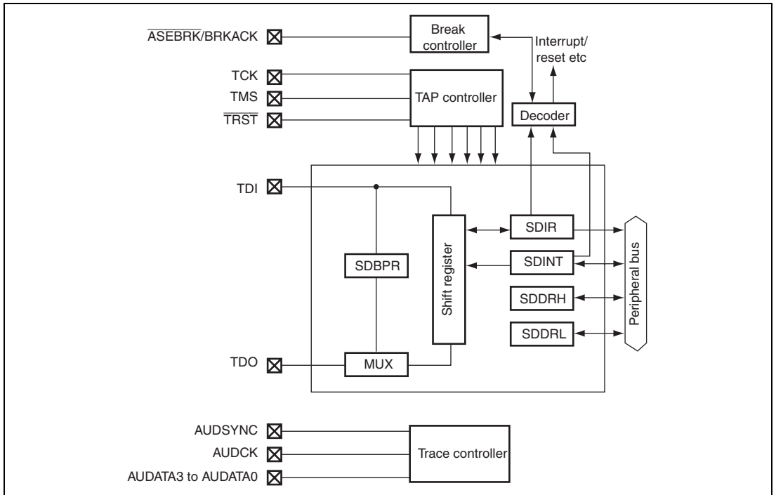
Figure 50.1 H-UDI Block Diagram
