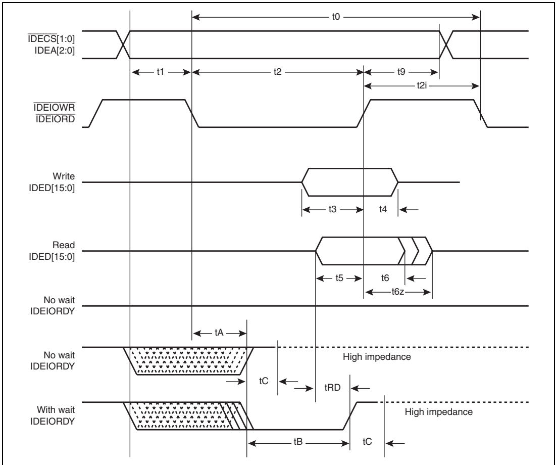
Figure 52.58 PIO Data Transfer and Register Transfer between Devices
