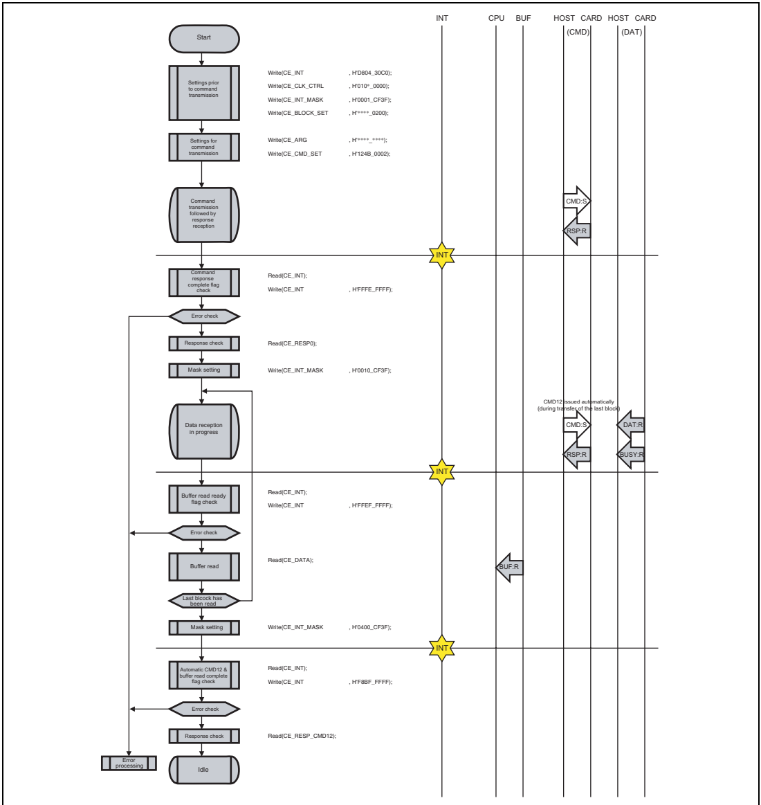
Figure 23.17 Multi-Block Read (with Automatic CMD12 Issuance) (CMD18)
