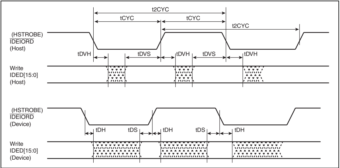
Figure 52.69 Ultra DMA Transfer Data Out Burst
