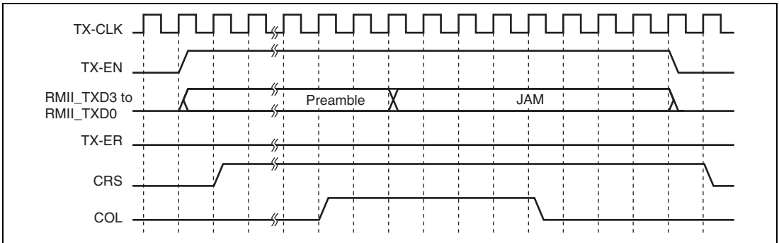
Figure 47.9 (2) MII Frame Transmit Timing (Collision)
