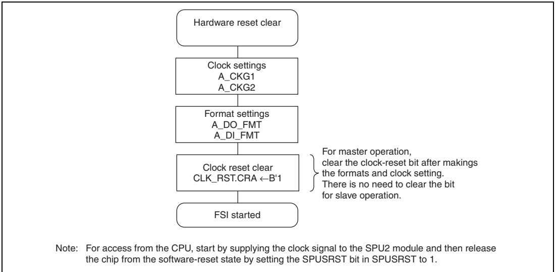
Figure 45.22 Flow for Starting FSI (Port A)
