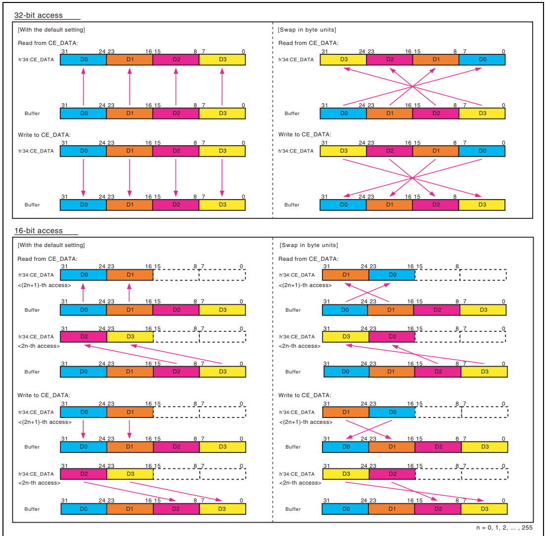
Figure 23.8 Specification of Byte-Swapping in 32/16-Bit Accesses
