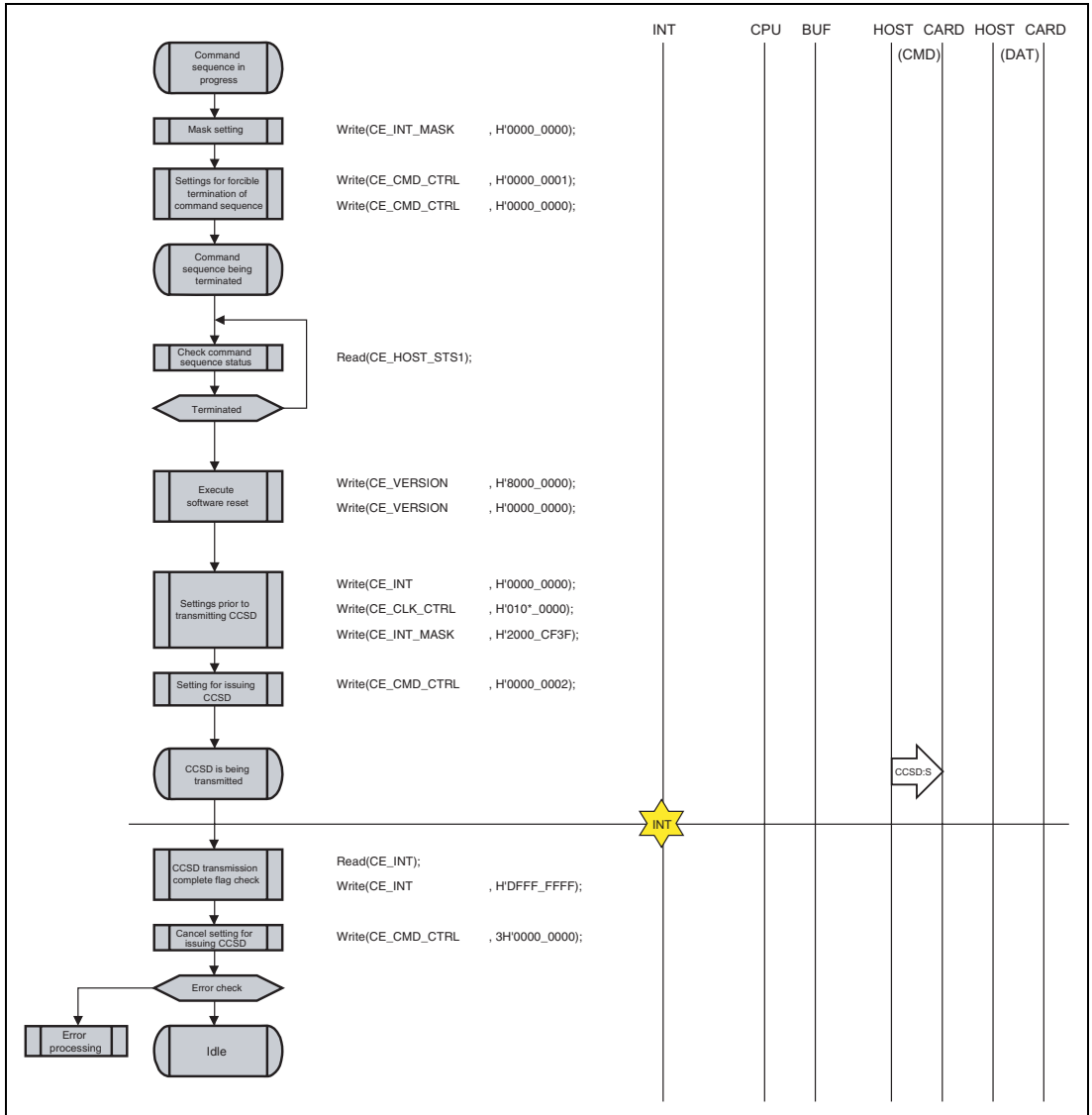
Figure 23.24 Forcible Termination → Transmission of CCSD
