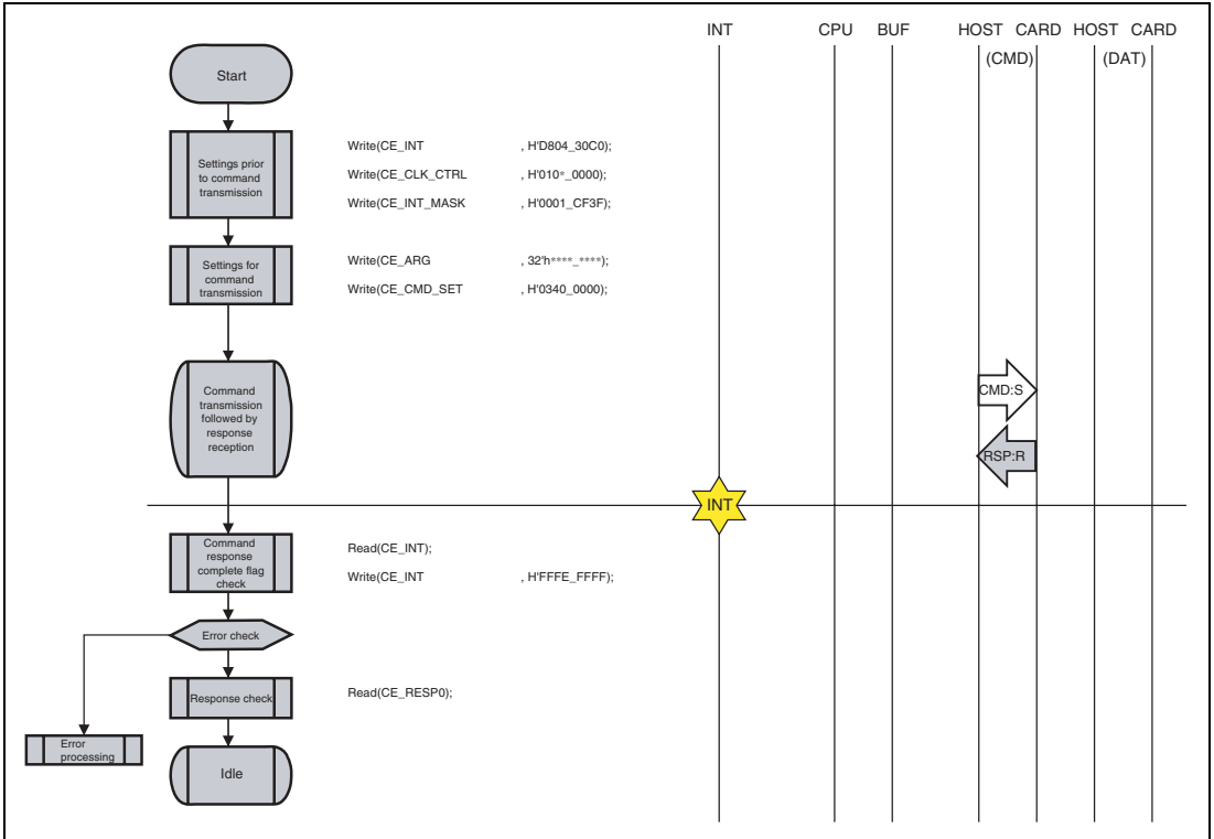
Figure 23.14 Command Transmission → Response Reception (CMD3)
