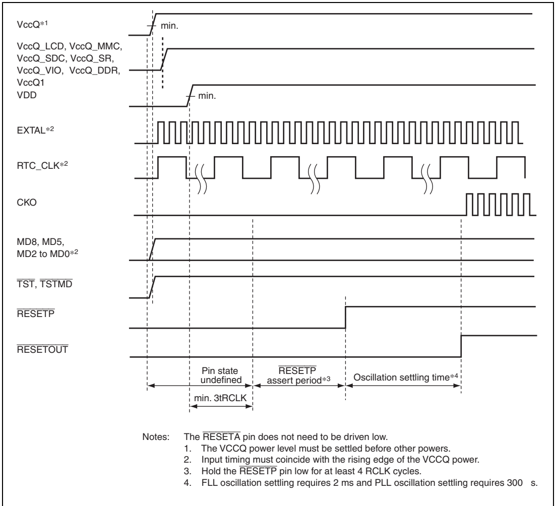
Figure 18.2 Power-On Sequence
