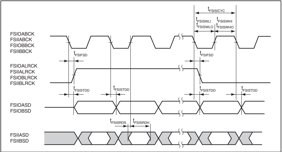
Figure 52.88 FSIMCK Transmission Timing
