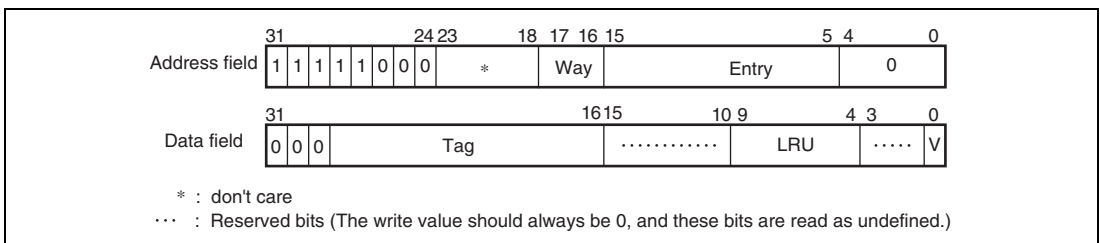
Figure 9.2 Memory-Mapped Secondary Cache Address Array
