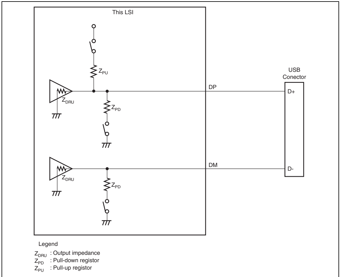
Figure 31.2 UBS Connector Connection
