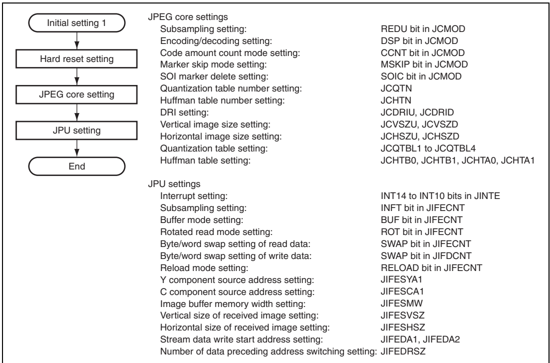
Figure 37.3 Flow of Initial Setting 1
