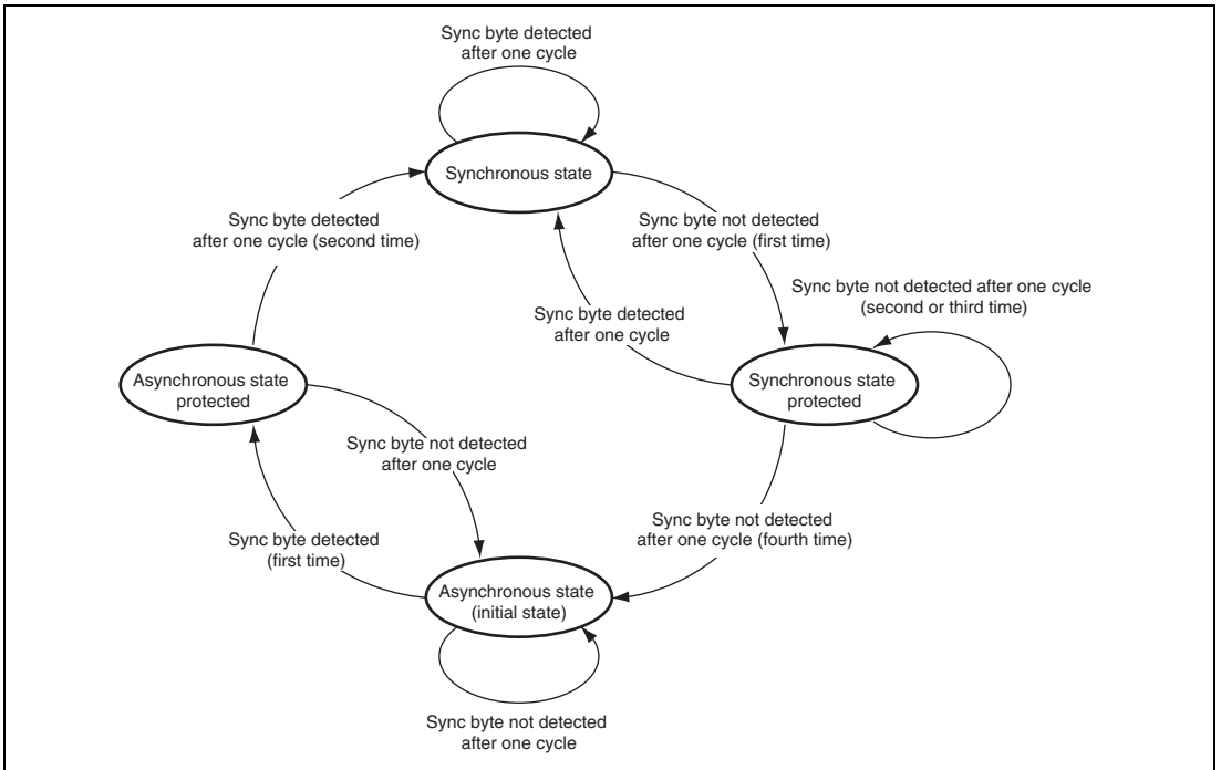
Figure 43.4 Detection State Configuration of Sync Byte
