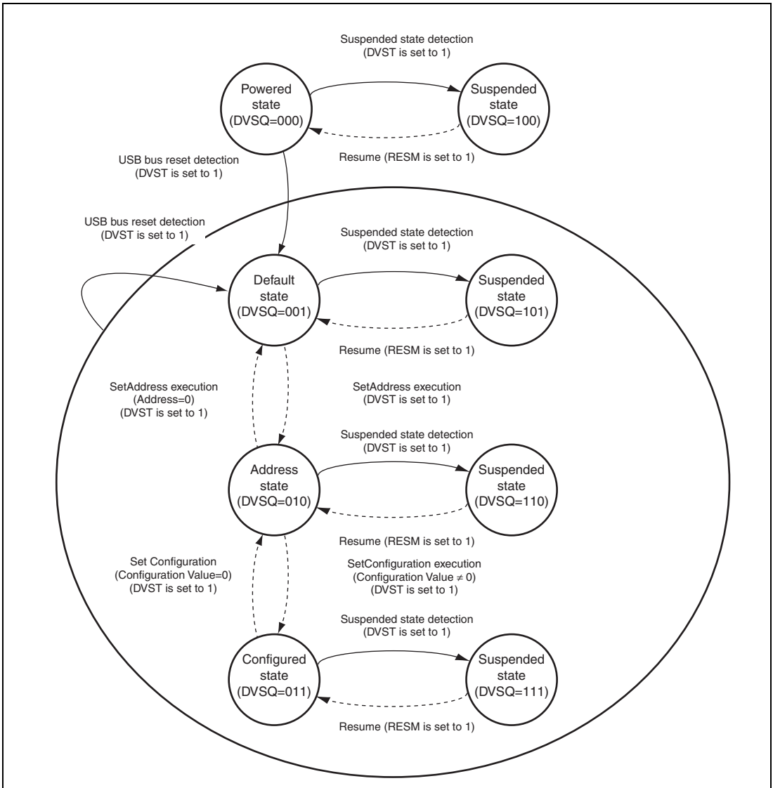
Figure 31.7 Device State Transitions
