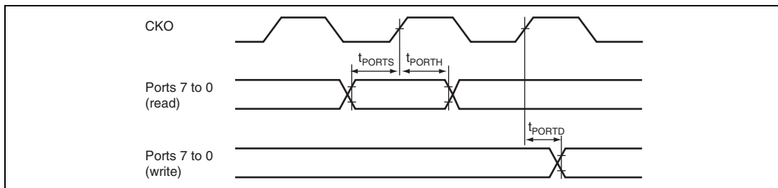
Figure 52.36 I/O Port Timing
