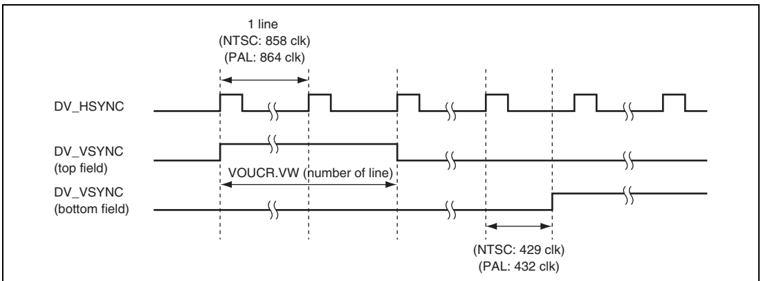
Figure 40.9 Timing of HSYNC and VSYNC Generation
