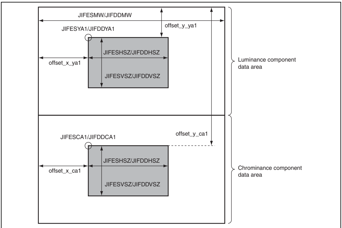
Figure 37.22 Data Allocation Image in Frame Buffer
