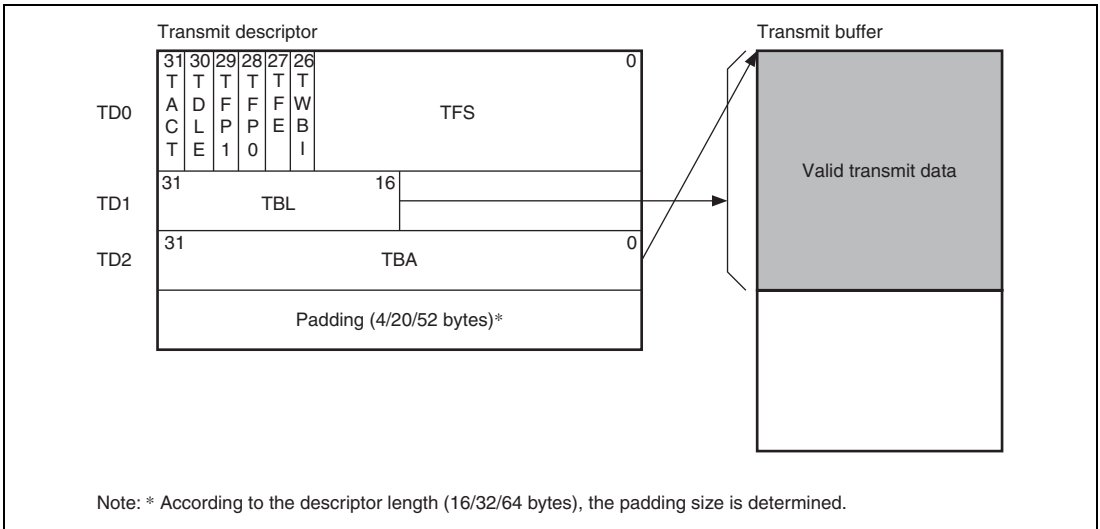
Figure 47.2 Relationship between Transmit Descriptor and Transmit Buffer
