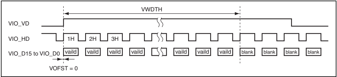
Figure 34.20 Vertical Capture Timing
