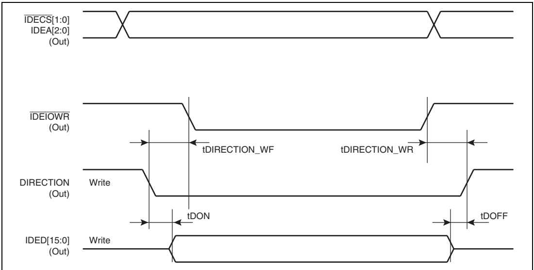
Figure 52.73 PIO Data Transfer to Device (DIRECTION)
