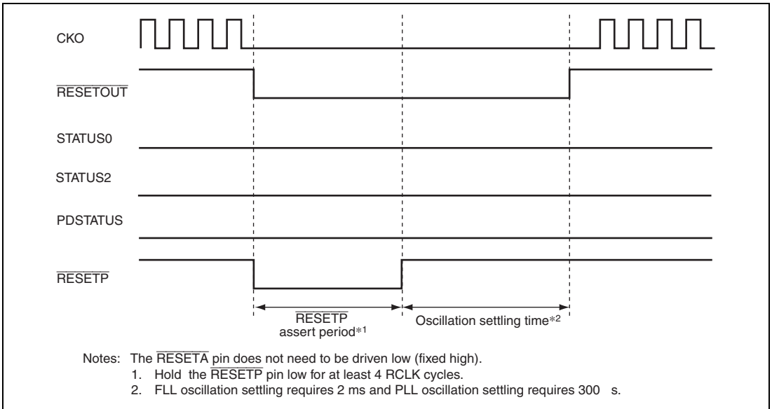
Figure 18.3 State of Output Pins at Power-On Reset
