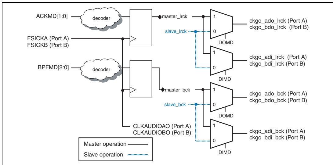
Figure 45.2 Master Clock Generation, I/O Operations, Master/Slave Selection
