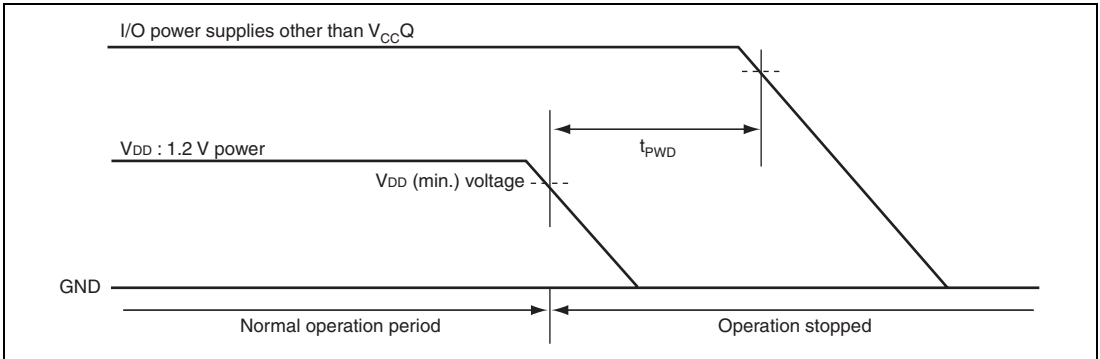
Figure 52.2 Power-off Sequence
