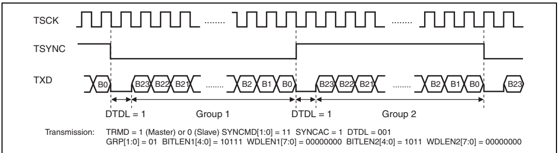
Figure 25.16 Transmit Timing (24 Bits IIS)
