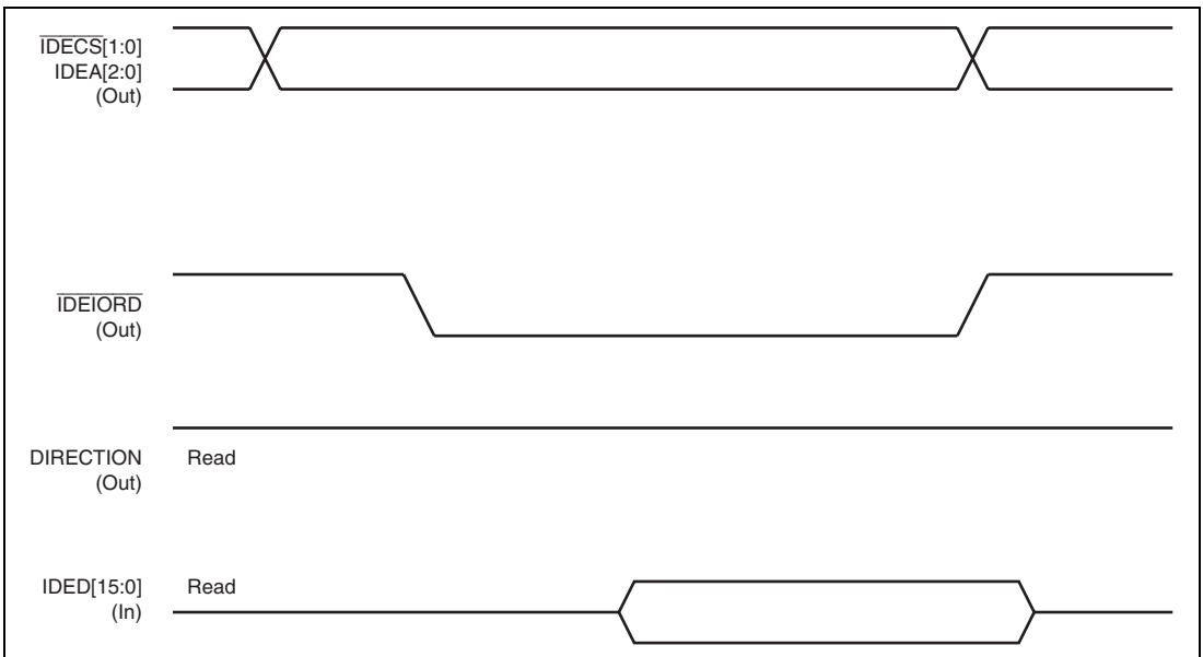
Figure 52.74 PIO Data Transfer from Device (DIRECTION)
