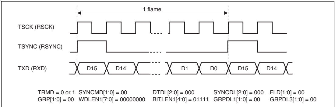
Figure 25.14 Transmit and Receive Timing (16 Bits)
