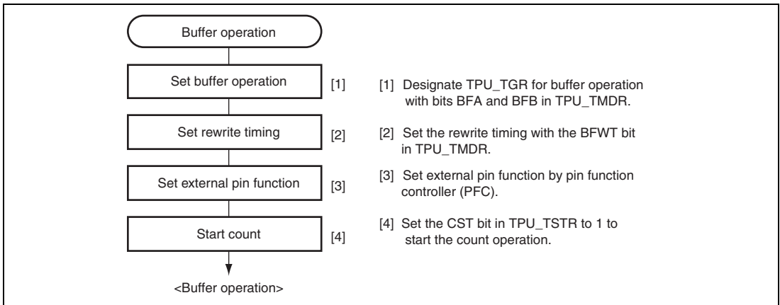
Figure 21.9 Example of Buffer Operation Setting Procedure
