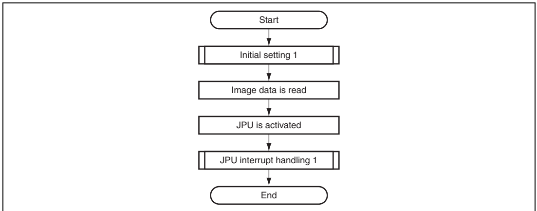
Figure 37.2 Flow of Encoding in Frame Buffer Mode
