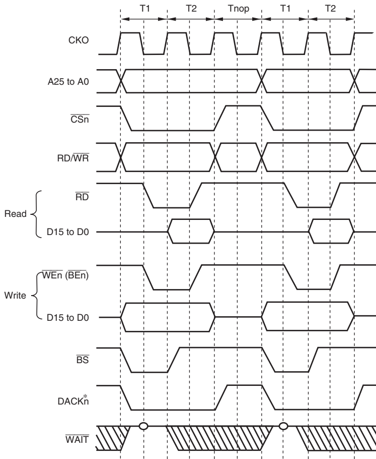
Figure 14.3 Continuous Access for Normal Space 1 Bus Width = 16 Bits, Longword Access, WM Bit in \overline{CS}_n\overline{WCR} = 0 (Access Wait = 0, Cycle Wait = 0)
