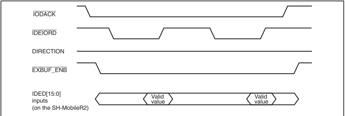
Figure 46.8 Multiword DMA Data-in Burst
