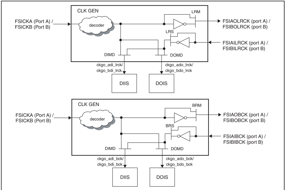
Figure 45.3 Master/Slave Clock Inversion Selector
