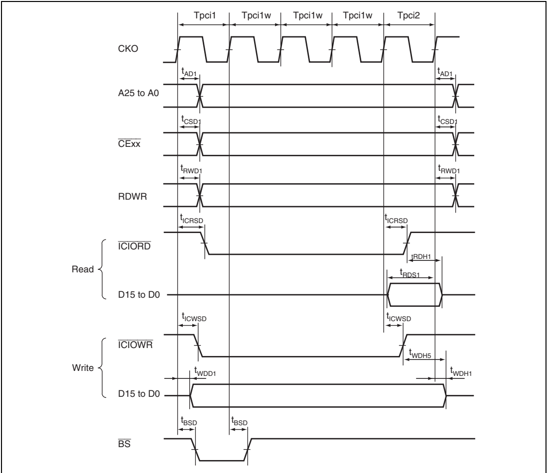
Figure 52.23 PCMCIA I/O Card Interface Bus Timing
