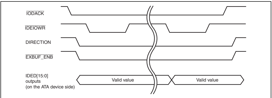
Figure 46.9 Multiword DMA Data-out Burst
