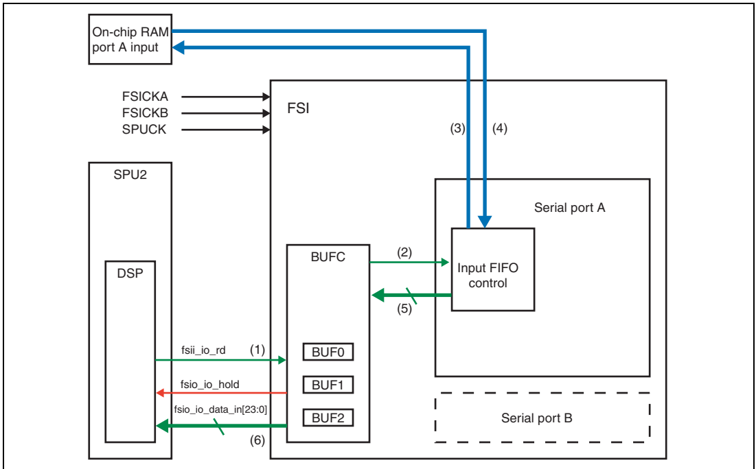
Figure 45.5 Block Diagram of Input FIFO Read Request
