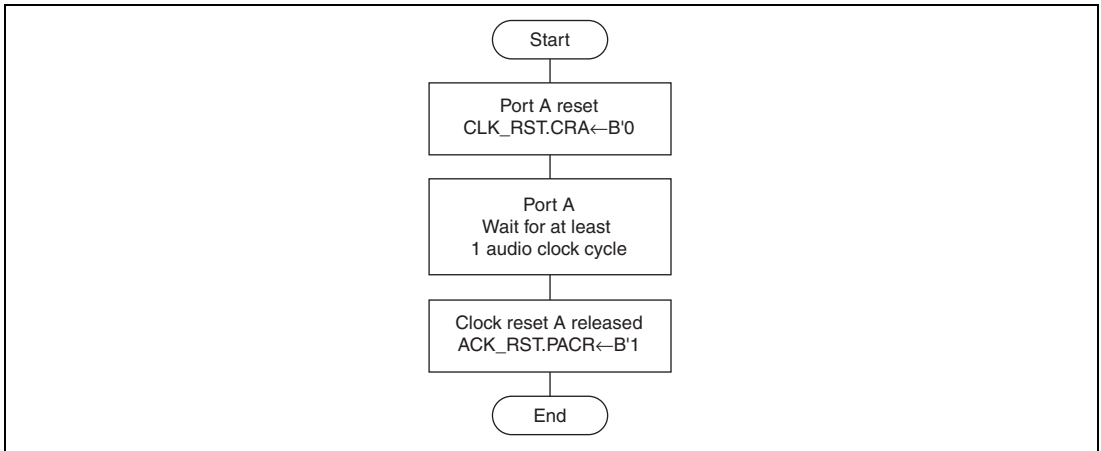
Figure 45.8 Flow of Clock Reset A
