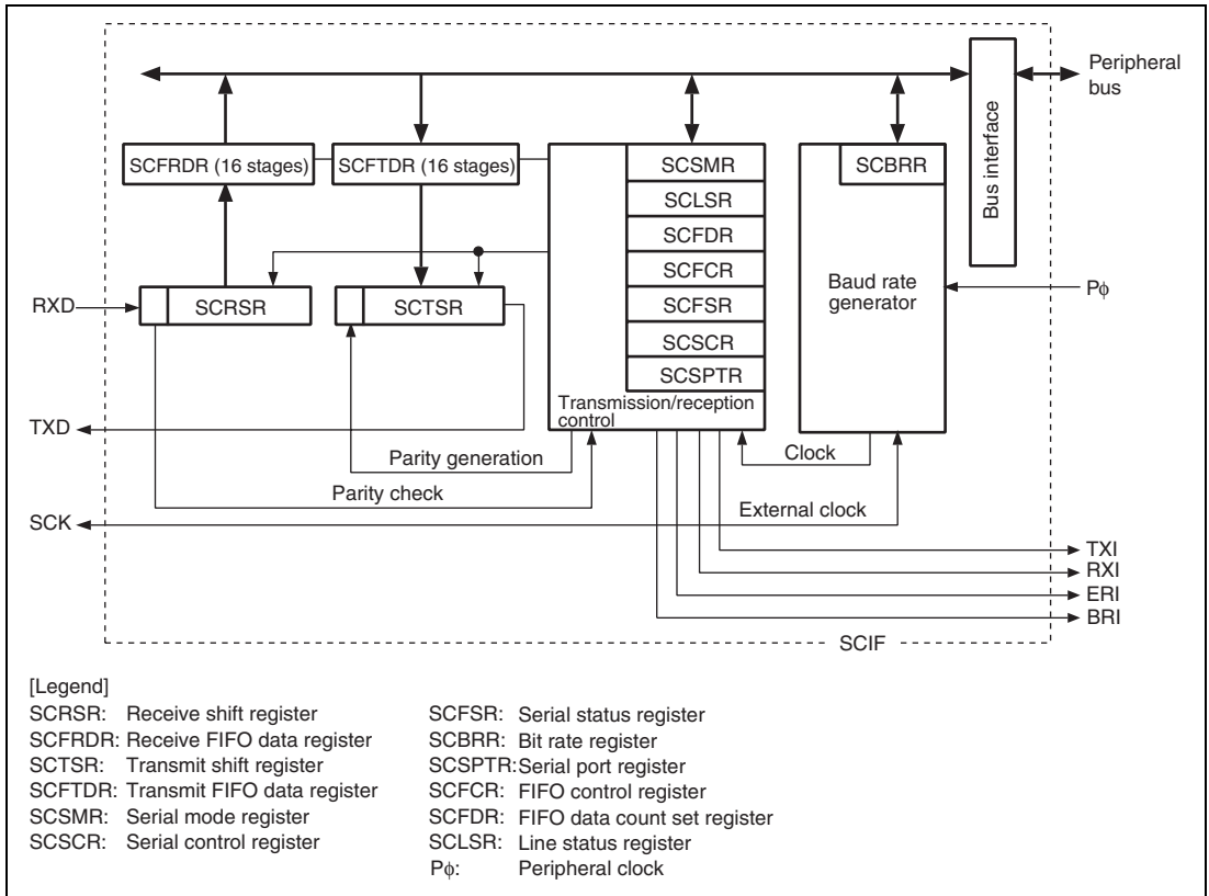
Figure 26.1 Block Diagram of SCIF
