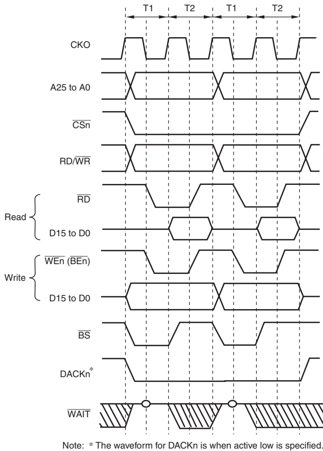
Figure 14.4 Continuous Access for Normal Space 2 Bus Width = 16 Bits, Longword Access, WM Bit in CSnWCR = 1 (Access Wait = 0, Cycle Wait = 0)
