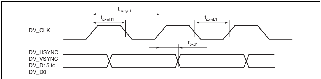
Figure 52.53 VOUModule AC Characteristics (VOUCR.CKPL = 0)
