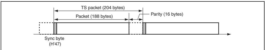
Figure 43.2 MPEG2-TS Packet Configuration
