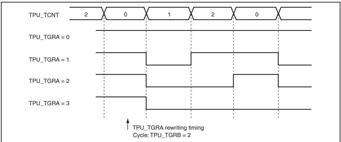
Figure 21.13 Example of PWM Mode Operation (2)
