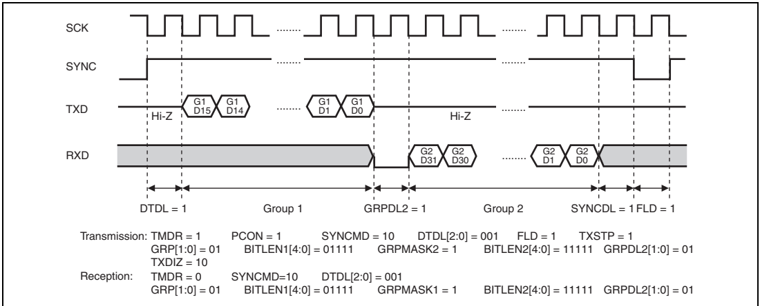
Figure 25.18 Transmit and Receive Timing ( \mu -WIRE)
