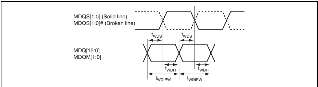
Figure 52.32 Relation between DQS and DQ/DQM Output Waveforms (Write)
