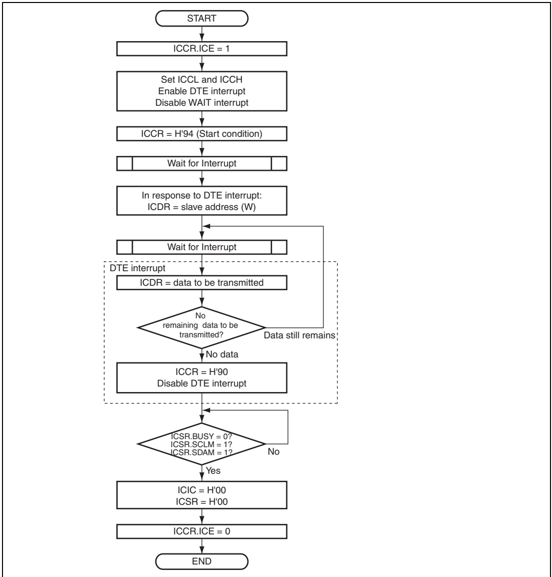
Figure 32.19 Example Flow of Software for Transmission (WAIT = 0)
