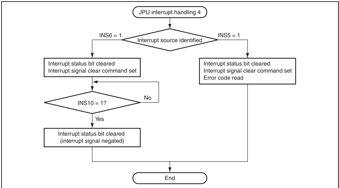
Figure 37.17 Flow of JPU Interrupt Handling 4
