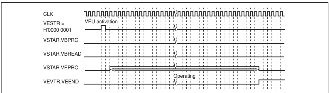
Figure 35.27 VSTAR State Transitions in Normal Operating Mode
