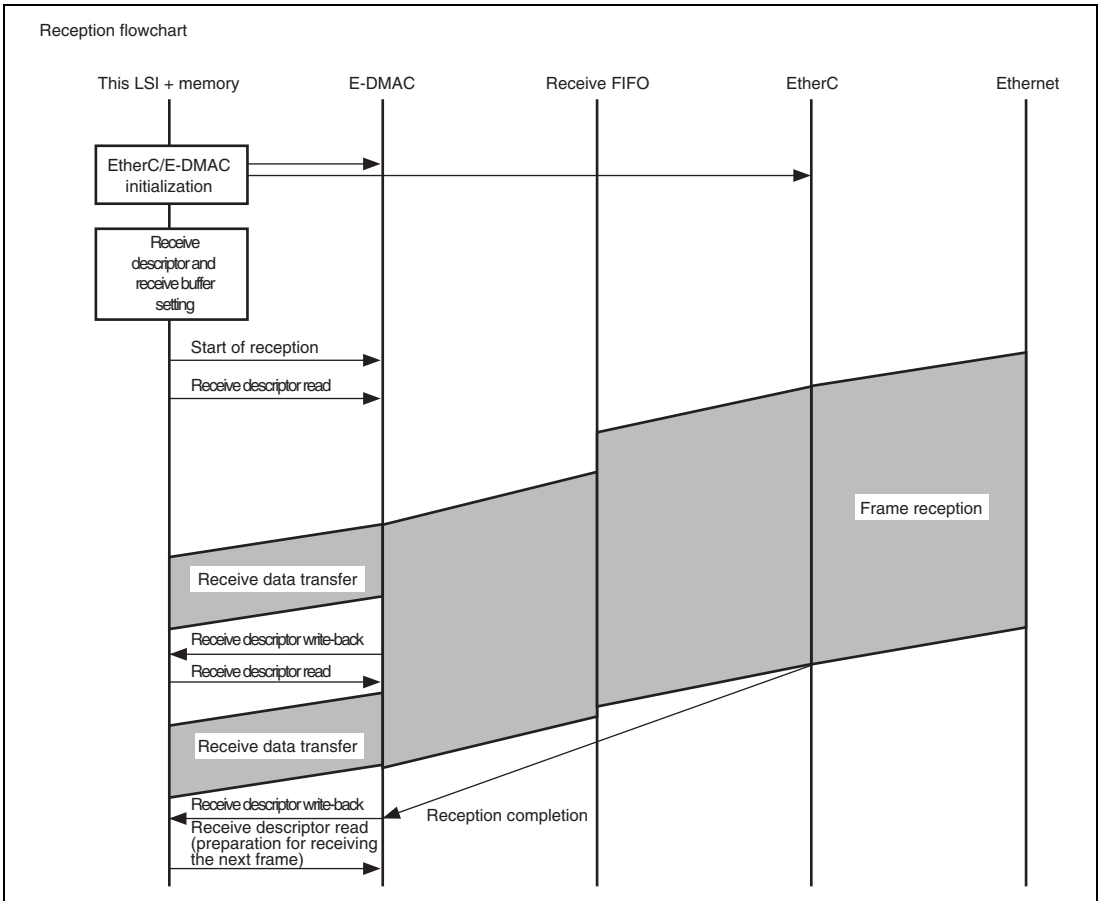
Figure 47.5 Sample Reception Flowchart (Single-Frame/Two-Descriptor)
