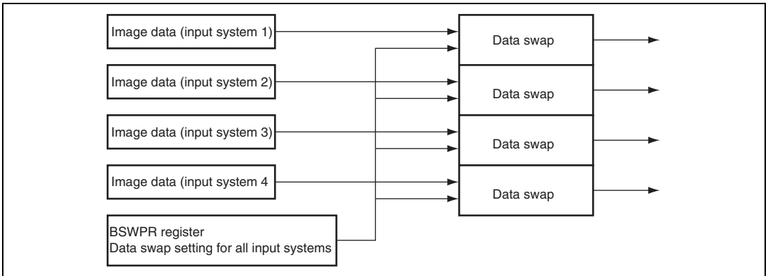
Figure 36.15 Data Swap Configuration when MODESEL = 0
