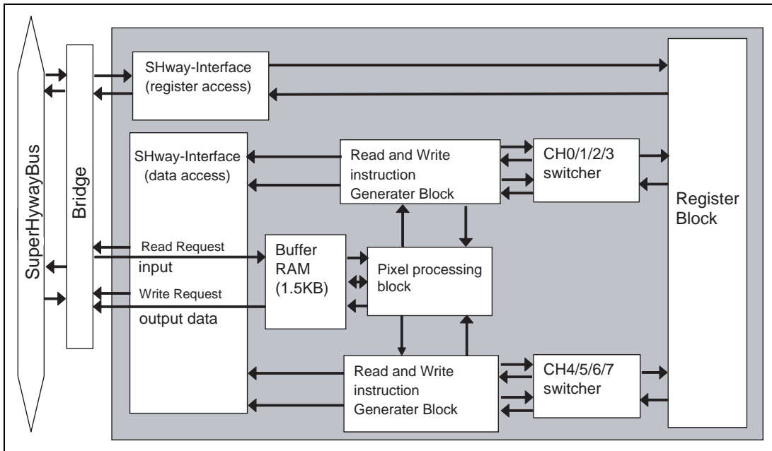
Figure 42.1 Block Diagram of 2D-DMAC
