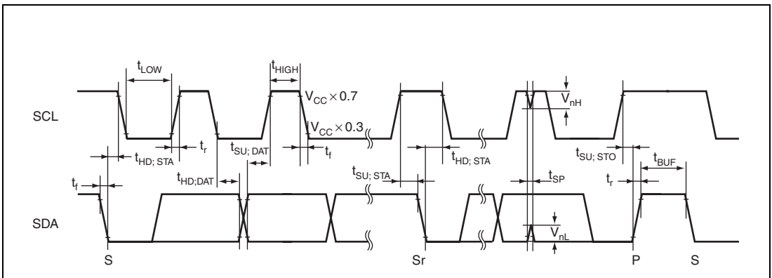
Figure 52.46 Device Timing Definition on I 2 C Bus
