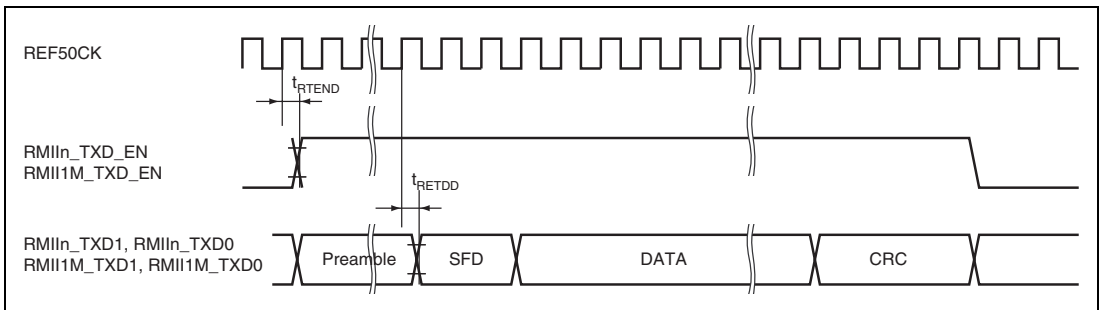
Figure 52.82 RMII Transmission Timing
