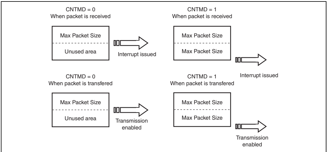
Figure 31.12 Example of Buffer Memory Operation
