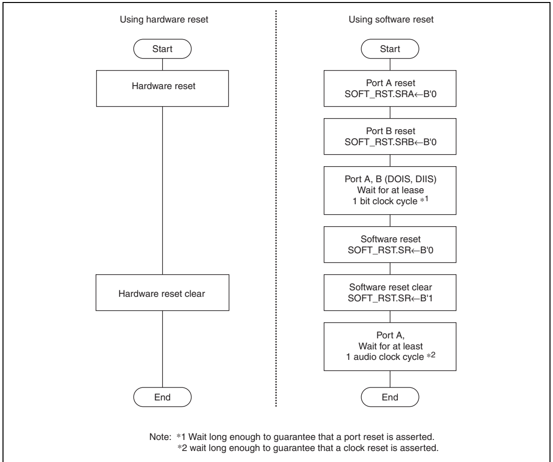
Figure 45.9 Operation Flow of FSI Initial States
