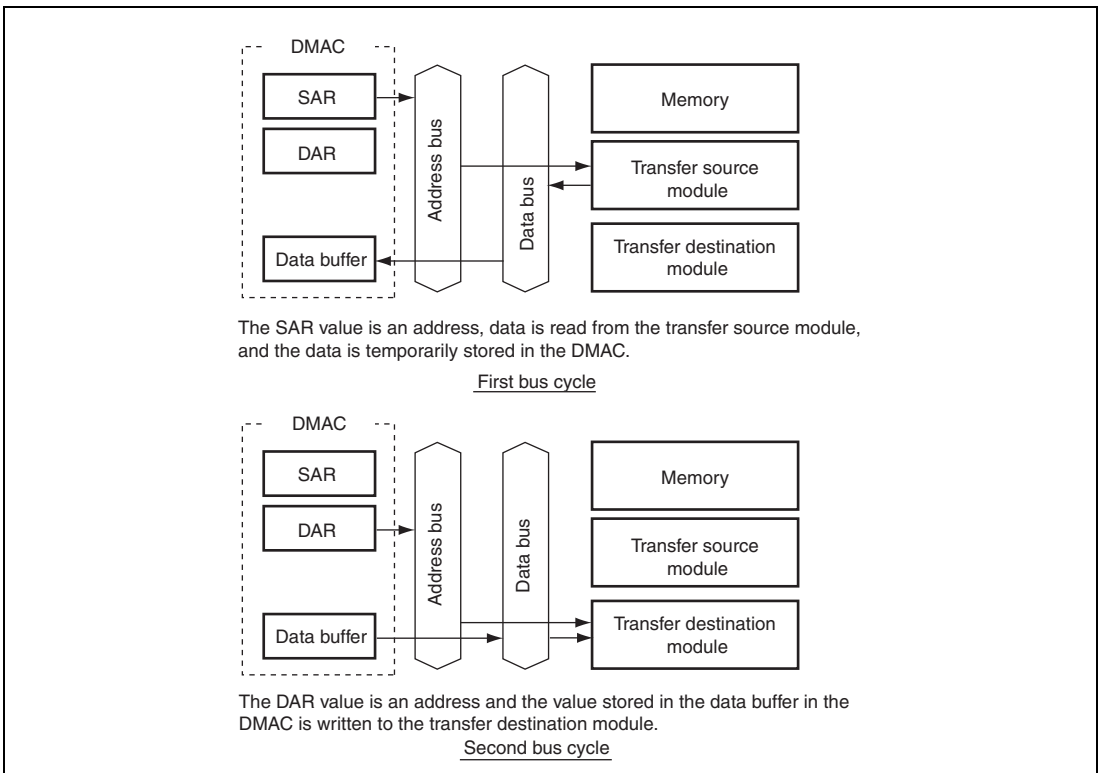
Figure 16.4 Data Flow of Dual Address Mode
