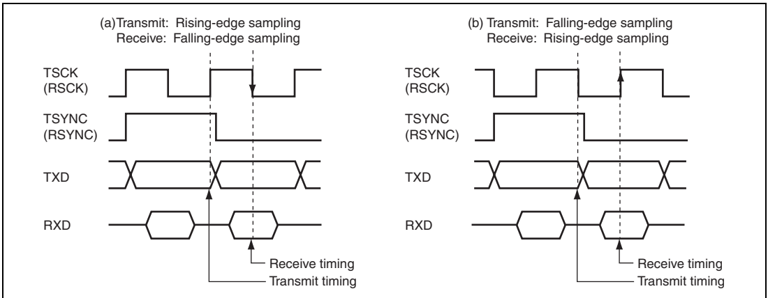
Figure 25.7 Transmit/Receive Timing.
