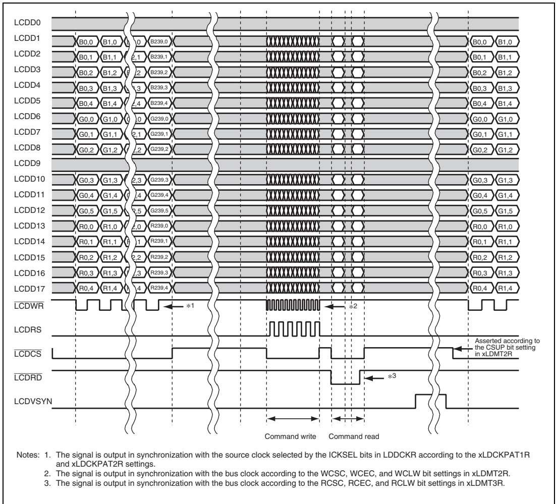
Figure 39.15 Example of Clock and LCD Data Signals (3)
