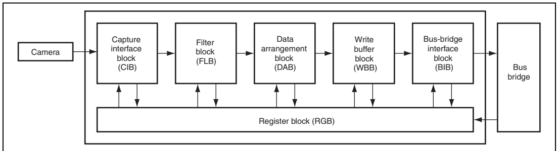
Figure 34.1 Block Diagram of CEU
