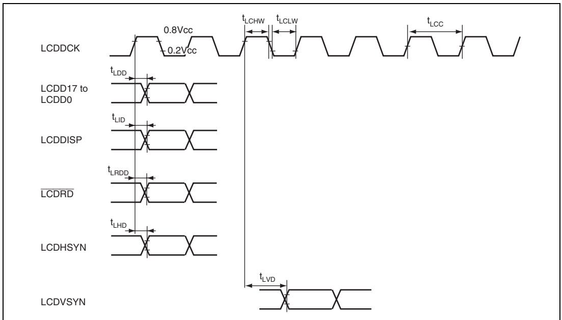
Figure 52.48 LCDC AC Characteristics
