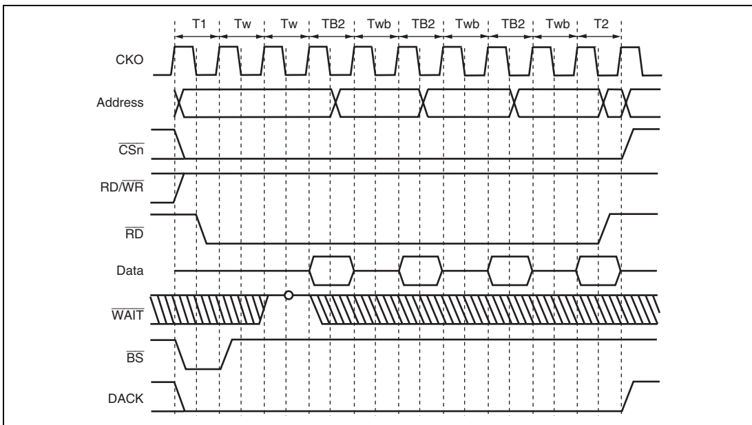
Figure 14.11 Burst ROM (Clock Asynchronous) Access (Bus Width = 32 Bits, 16-byte Transfer (Number of Bursts = 4), Access Wait for 1st Time = 2, Access Wait for 2nd Time and After = 1)
