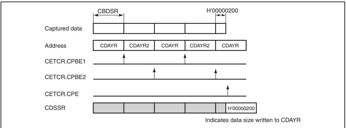
Figure 34.51 Overall Timing of CDSSR Operation in Bundle Write (When Bundle Write End and Capture End Does Not Coincide)
