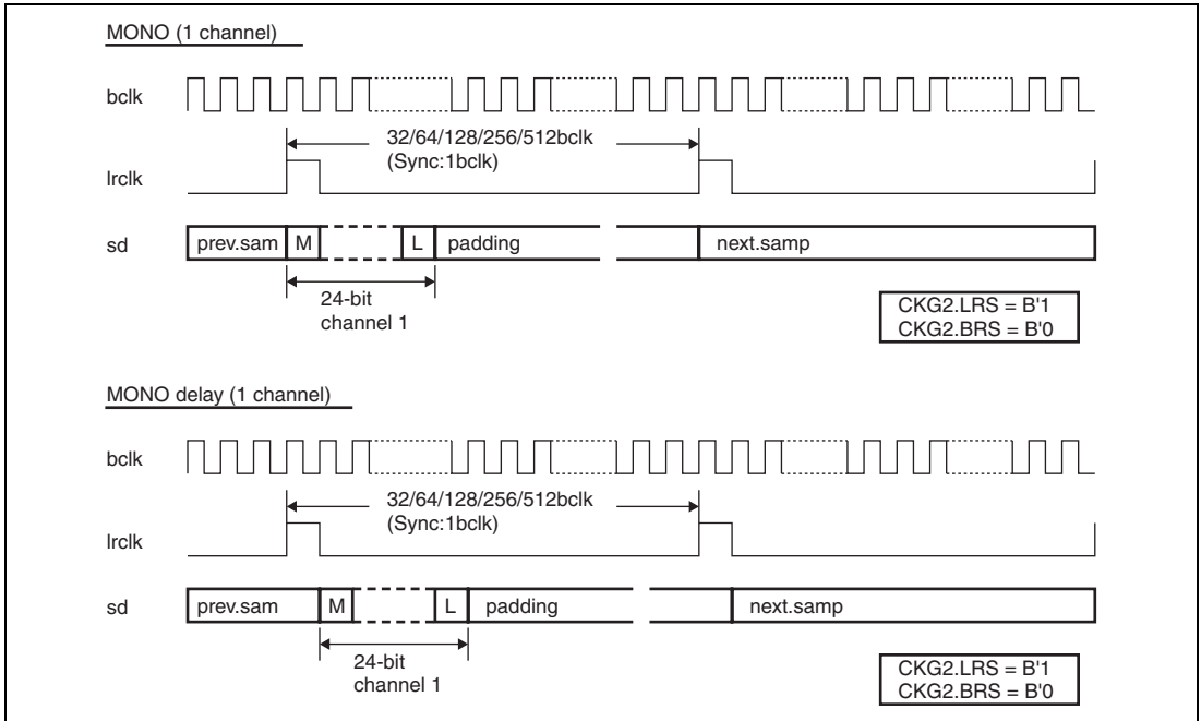
Figure 45.16 MONO and Mono delay Formats
