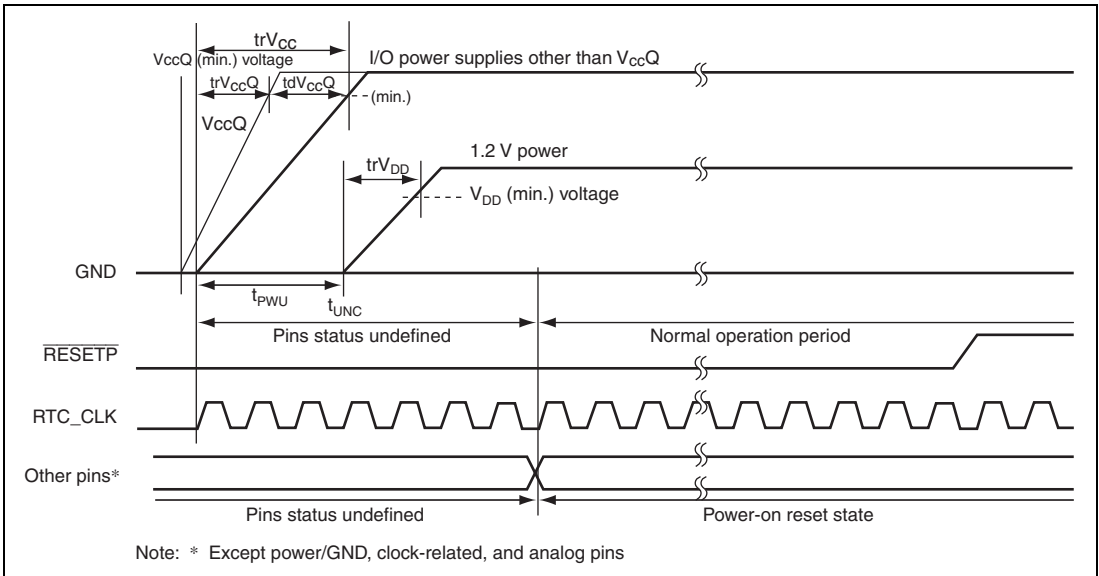
Figure 52.1 Power-on Sequence
