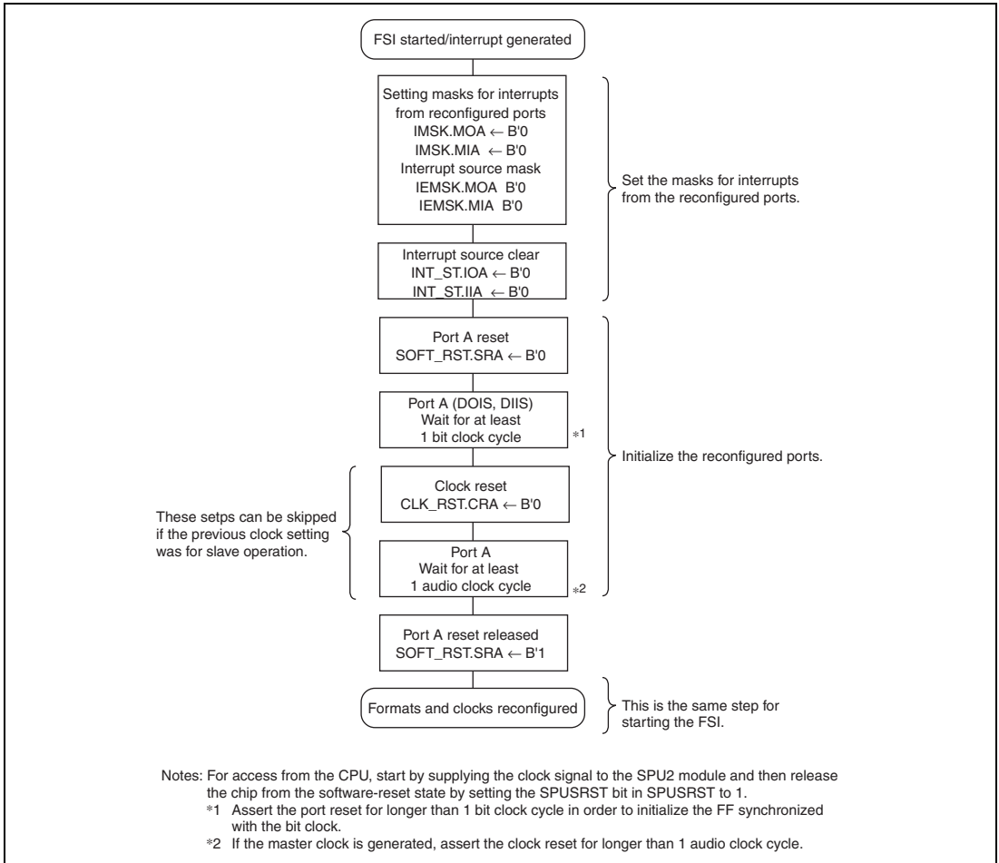
Figure 45.23 Flow for Restarting FSI (Port A)
