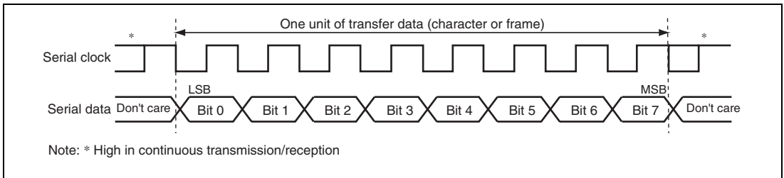
Figure 27.12 Data Format in Synchronous Communication
