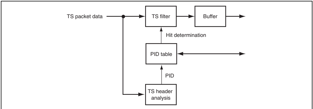
Figure 43.5 Block Diagram of PID Filtering
