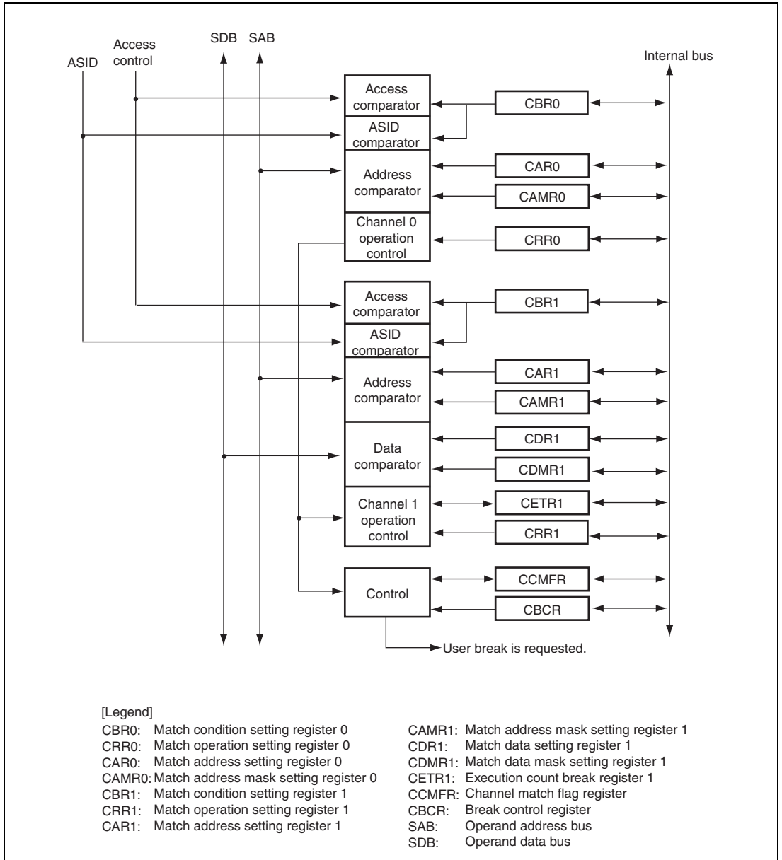
Figure 49.1 Block Diagram of UBC
