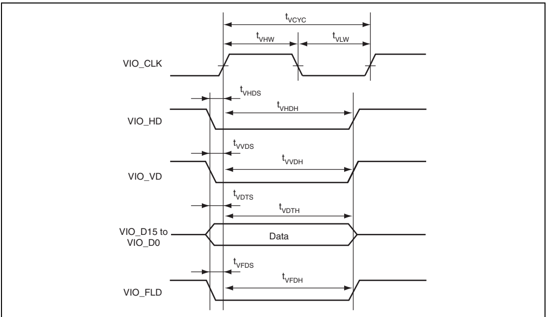
Figure 52.47 VIO Module Signal Timing
