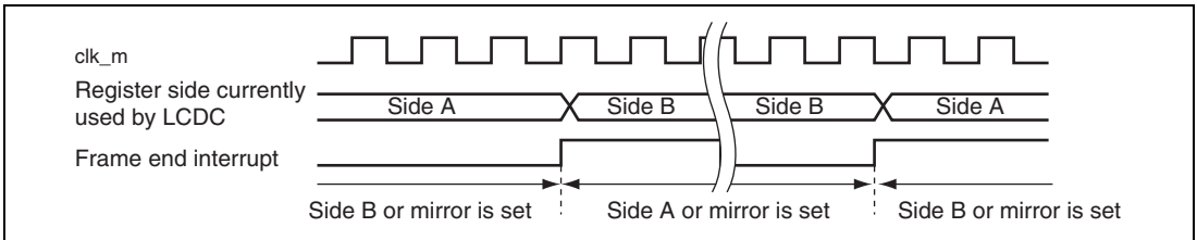
Figure 39.12 Timing of Interrupts and Register Setting
