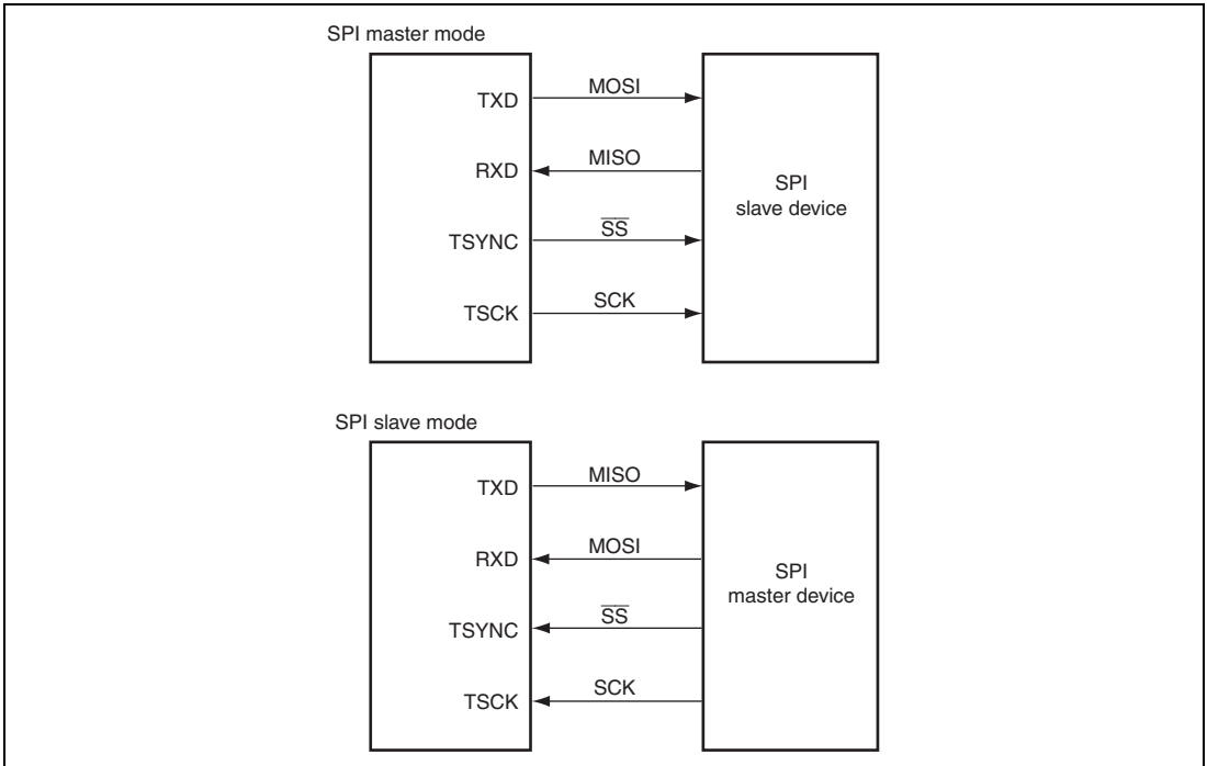
Figure 25.19 Example of SPI Device Connection
