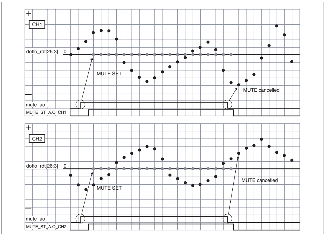
Figure 45.10 Normal MUTE Specification (Output Operation)
