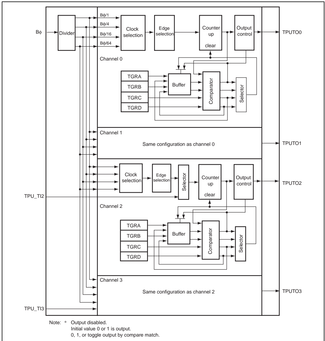
Figure 21.1 TPU Block Diagram
