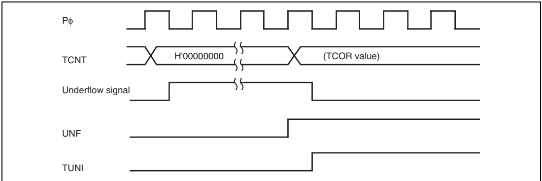
Figure 20.5 UNF Set Timing
