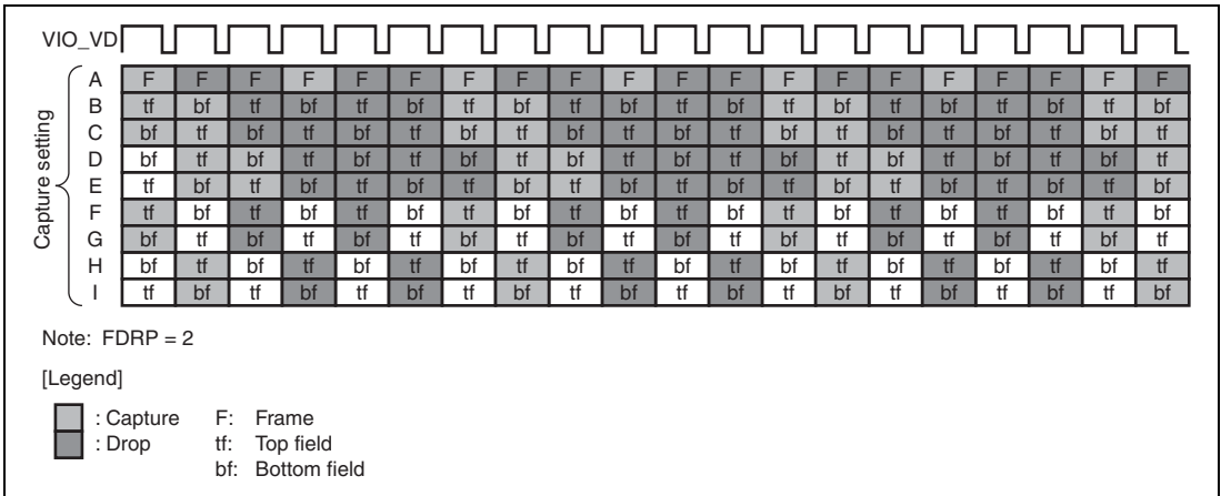
Figure 34.10 Image of Frame Drop Timing for Capture Settings (FDRP Bits = 2)
