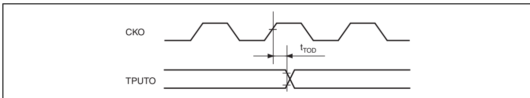
Figure 52.39 TPU Output Timing
