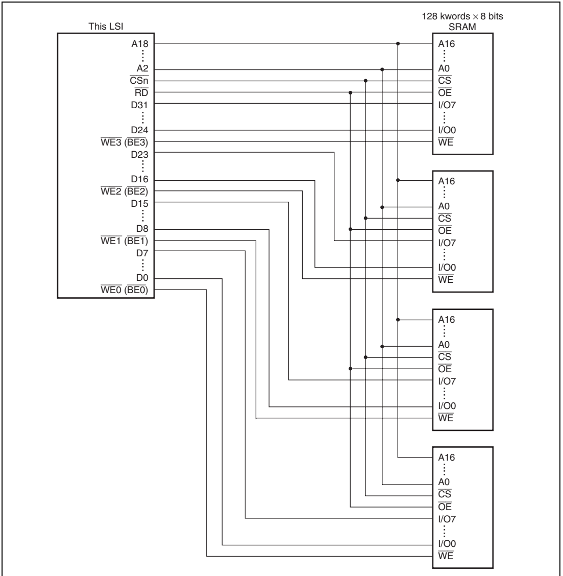
Figure 14.5 Example of 32-Bit Data-Width SRAM Connection
