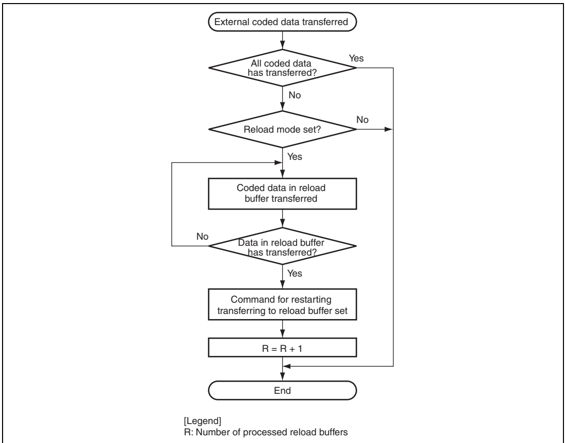
Figure 37.15 Flow of Transferring External Coded Data
