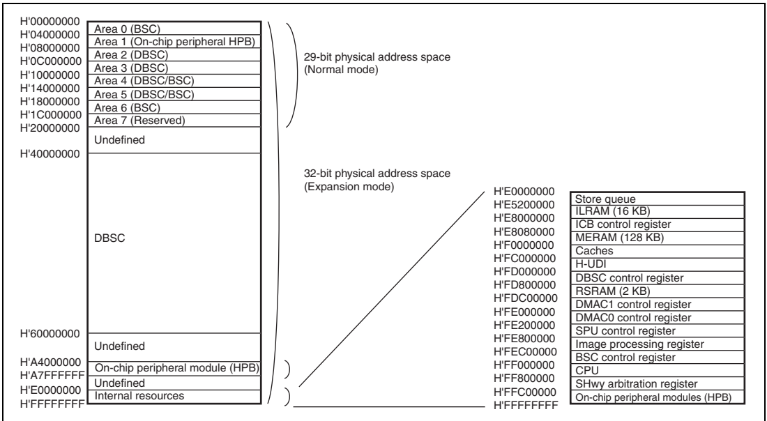
Figure 1.4 Physical Address Space
