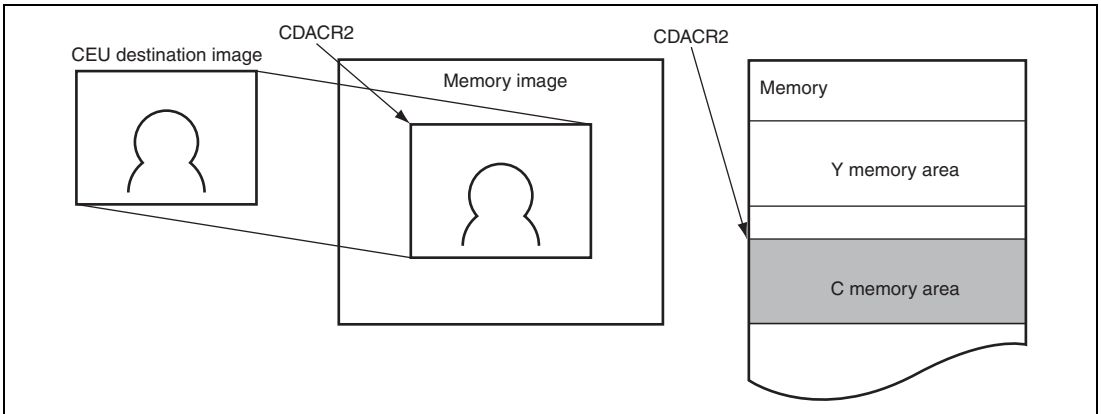
Figure 34.53 Relationship between Captured Image and C Component Memory Area
