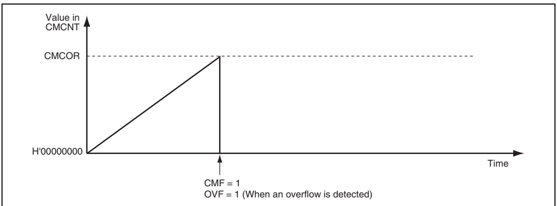
Figure 22.2 Counter Operation (One-Shot Operation)
