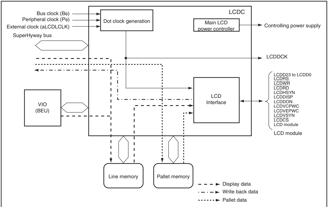
Figure 39.1 Block Diagram of LCDC
