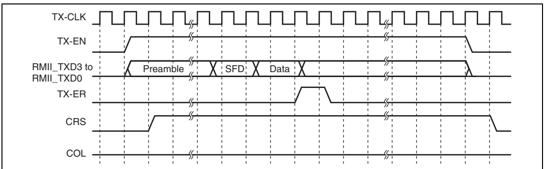
Figure 47.9 (3) MII Frame Transmit Timing (Transmit Error)
