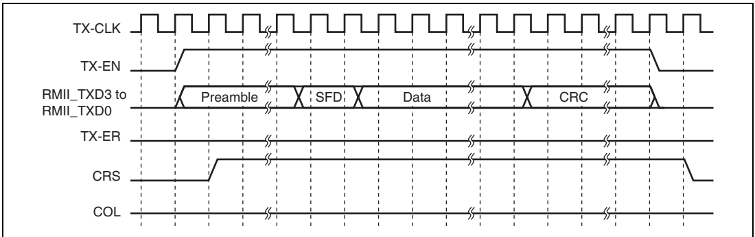
Figure 47.9 (1) MII Frame Transmit Timing (Normal Transmission)
