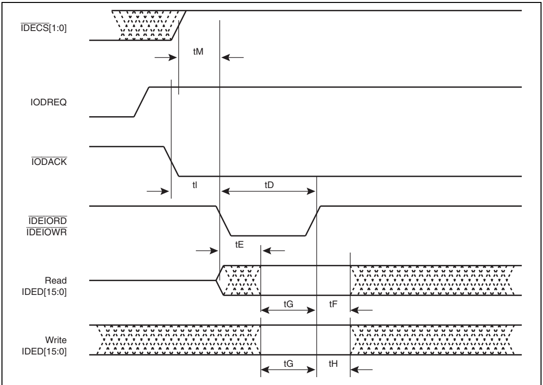
Figure 52.59 Start of Multiword DMA Data Transfer
