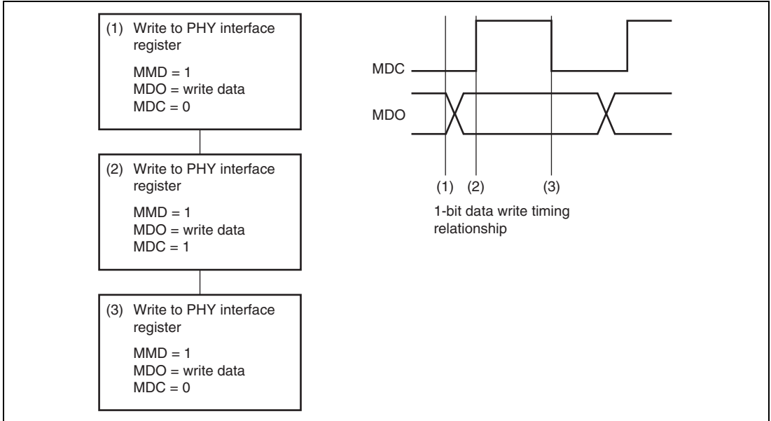
Figure 47.11 (1) 1-Bit Data Write Flowchart
