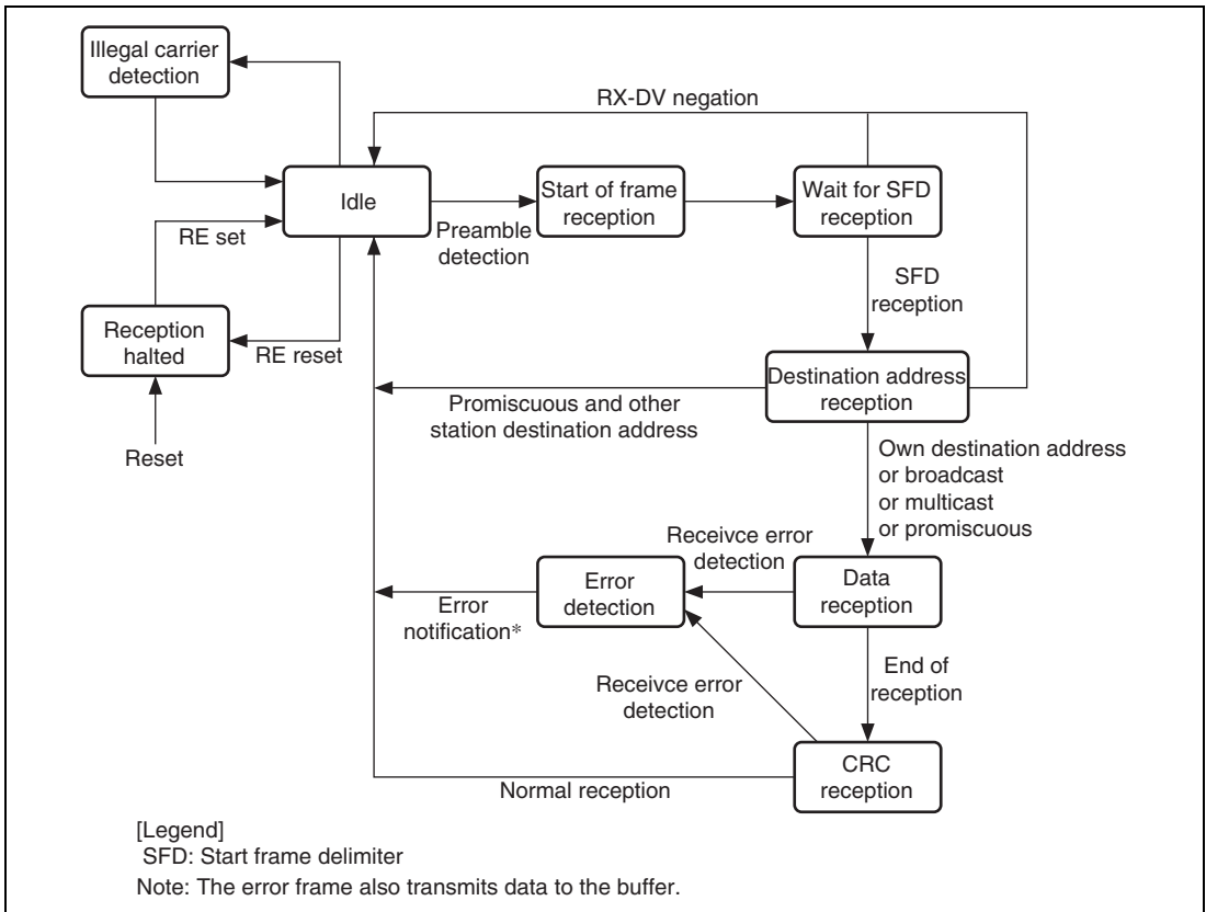
Figure 47.8 EtherC Receiver State Transmissions
