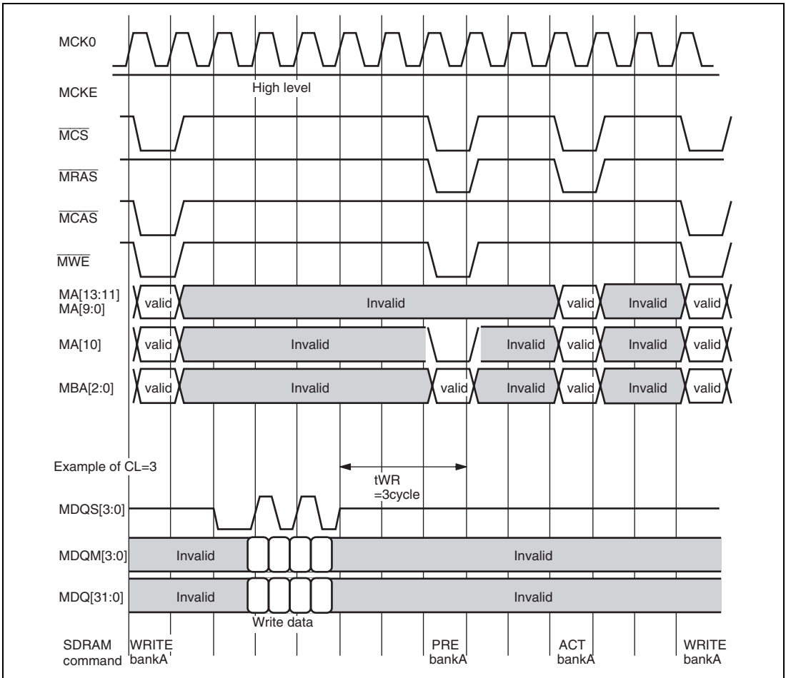
Figure 15.15 t_{WR}
