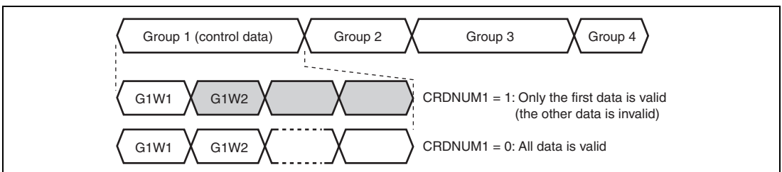
Figure 25.8 Control Data Allocation
