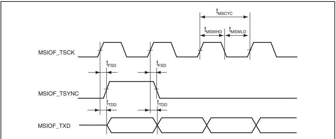
Figure 52.42 MSIOF Transmission/Reception Timing (Master Mode 1)
