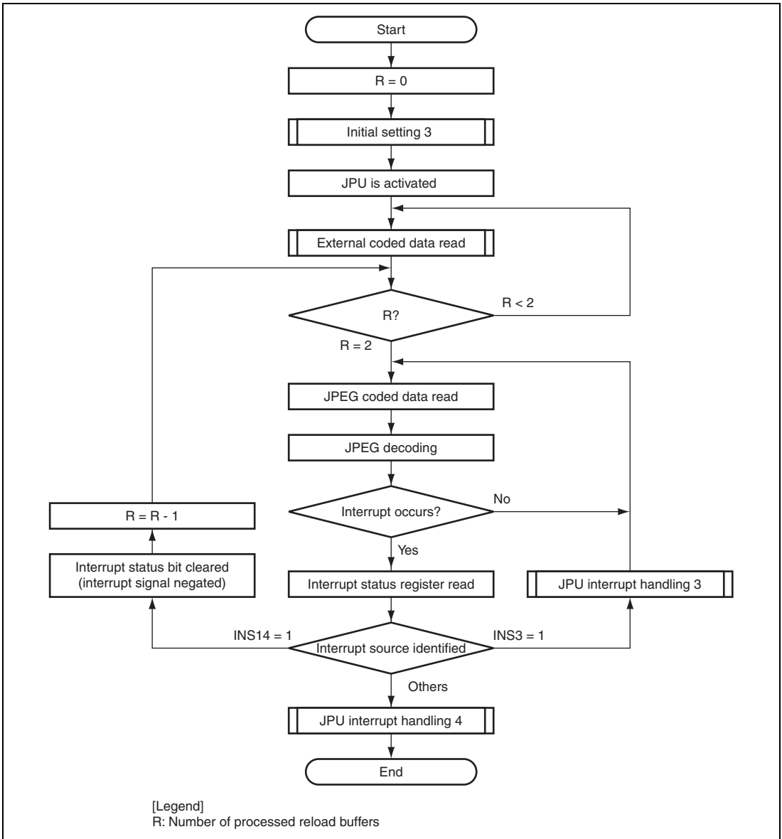
Figure 37.13 Flow of Decoding in Frame Buffer Mode
