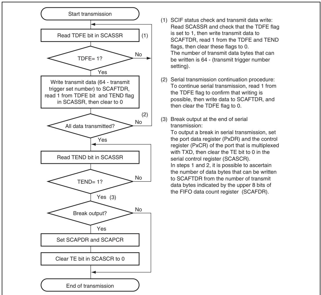
Figure 27.3 Sample Serial Transmission Flowchart
