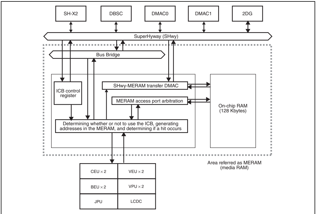
Figure 41.1 Relationship between MERAM and Other Modules
