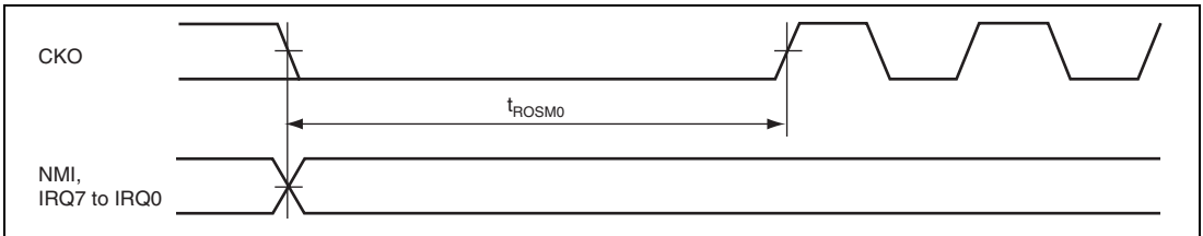
Figure 52.8 Oscillation Settling Time on Return to R-standby due to NMI and IRQ (Clock Mode 3)
