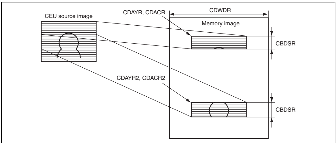
Figure 34.41 Image of Bundle Write to Memory
