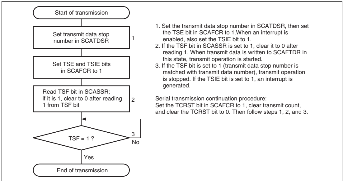
Figure 27.6 Transmit Data Stop Function Flowchart
