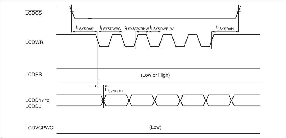
Figure 52.51 LCDC AC Characteristics (SYS Interface, Data Write Bus Cycle)
