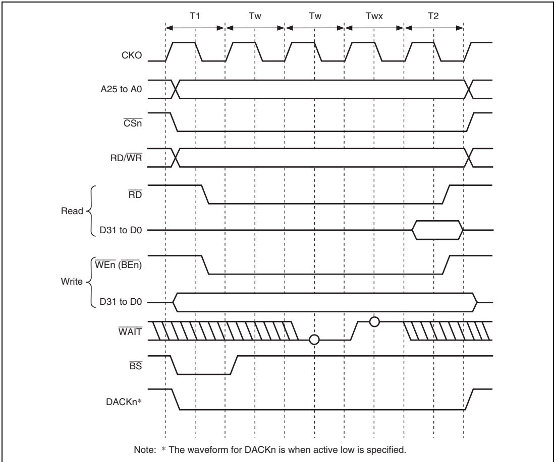
Figure 14.9 Wait Cycle Timing for Normal Space Access (Wait Cycle Insertion Using \overline{\text{WAIT}} Signal)
