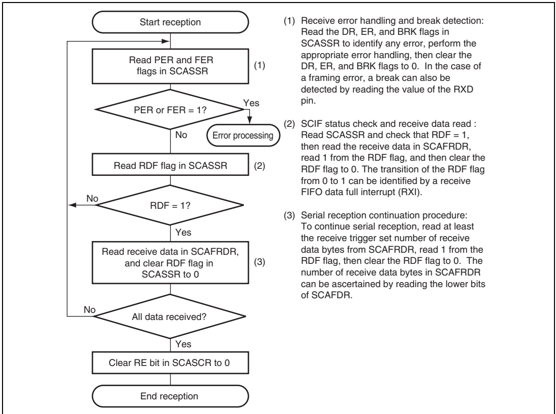
Figure 27.7 Sample Serial Reception Flowchart (1)
