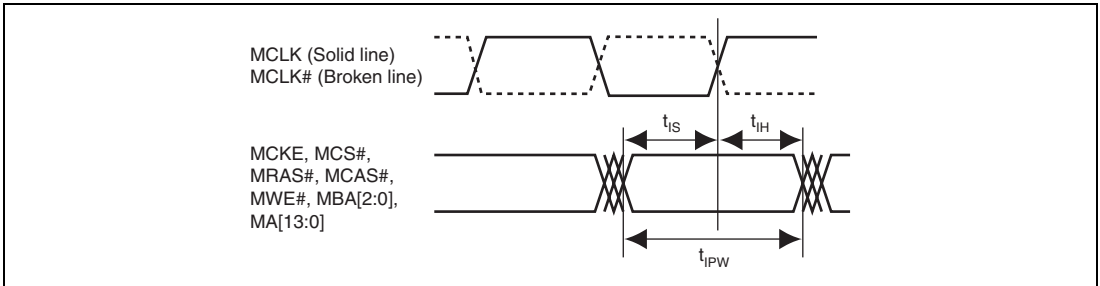
Figure 52.26 Relation between Command Pins and Output Clock
