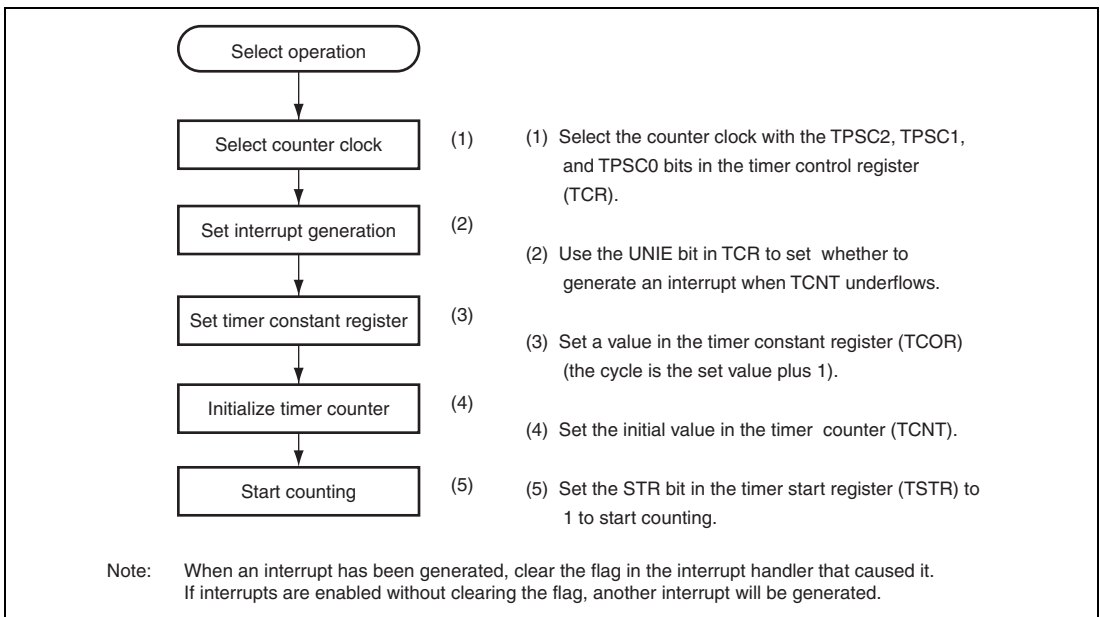
Figure 20.2 Setting Count Operation
