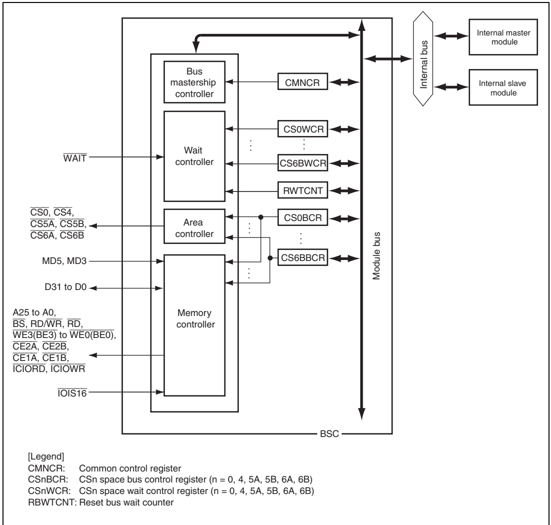
Figure 14.1 Block Diagram of BSC
