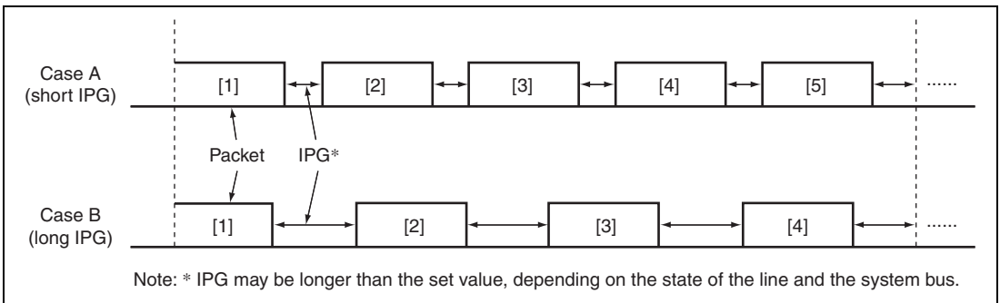
Figure 47.12 Changing IPG and Transmission Efficiency
