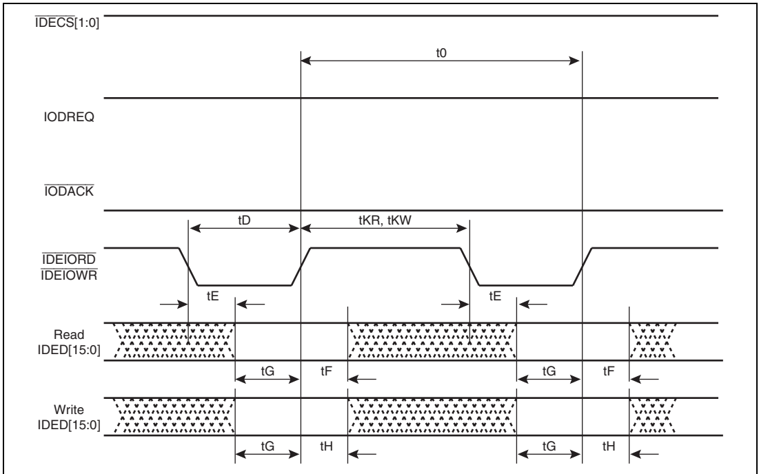
Figure 52.60 Multiword DMA Data Transfer
