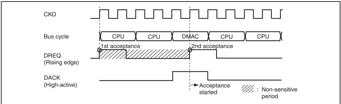
Figure 16.12 Example of DREQ Input Detection in Cycle Steal Mode Edge Detection
