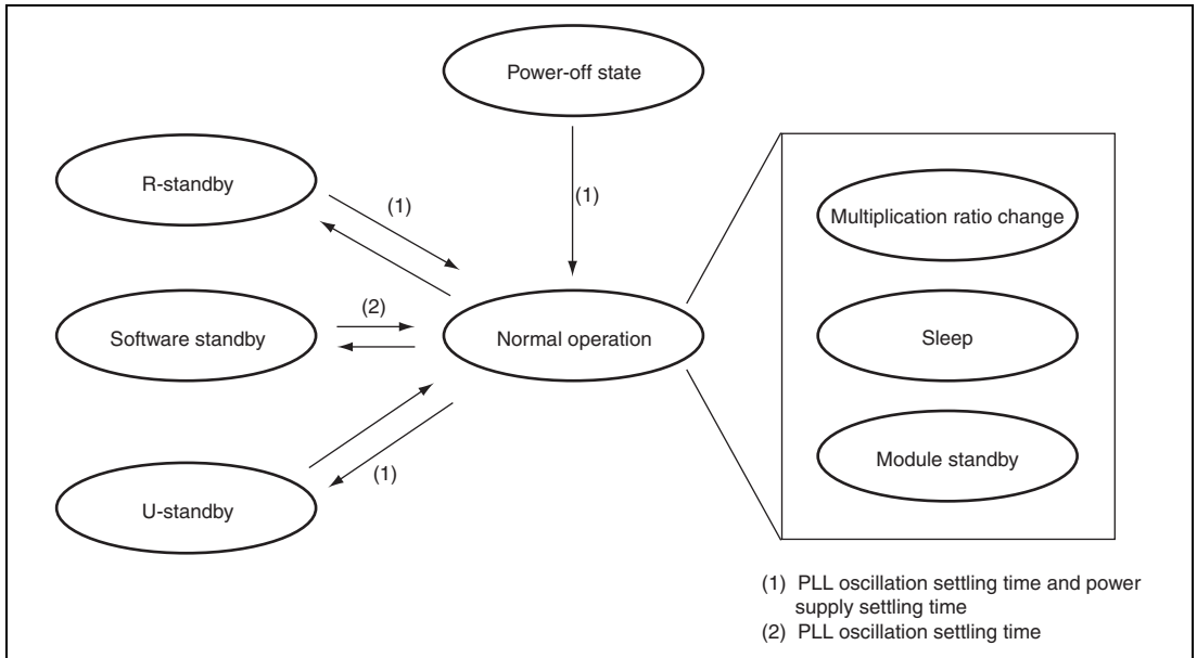
Figure 18.1 Mode Transition Diagram
