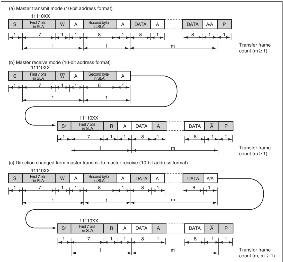
Figure 32.5 I 2 C Bus Data Formats (10-Bit Address Format)
