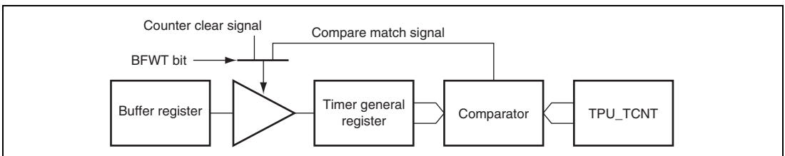
Figure 21.8 Compare Match Buffer Operation
