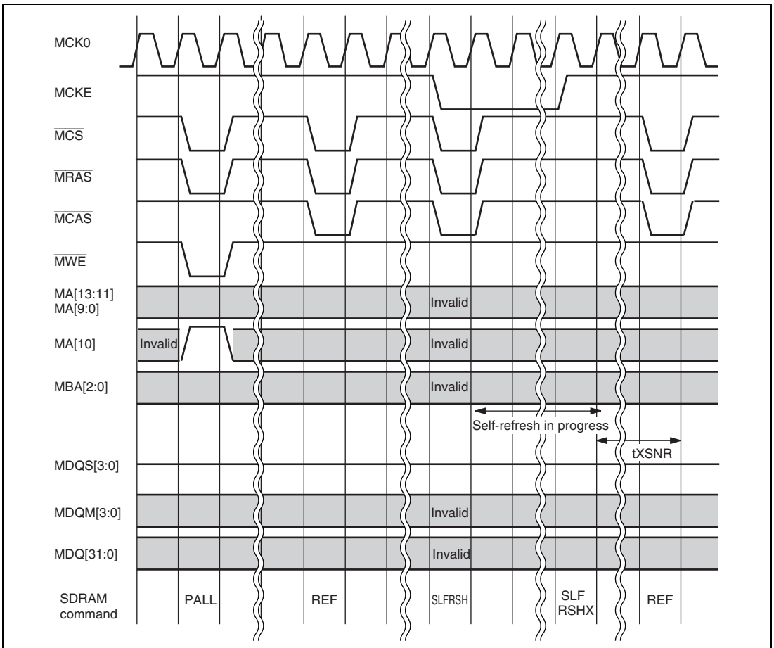
Figure 15.12 Self-Refresh Operation
