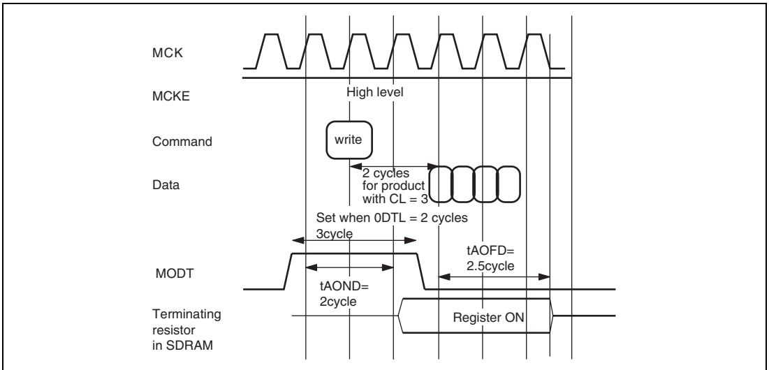
Figure 15.21 ODT Control Signal when CL = 3
