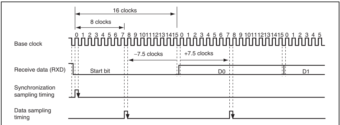
Figure 27.22 Received data Sampling Timing in Asynchronous Mode
