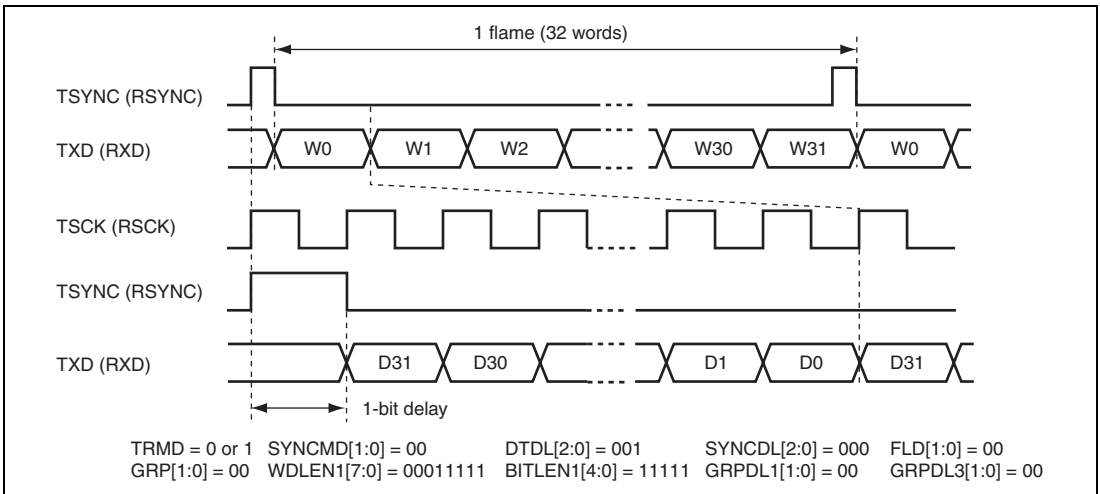
Figure 25.15 Transmit and Receive Timing (32 Bits)
