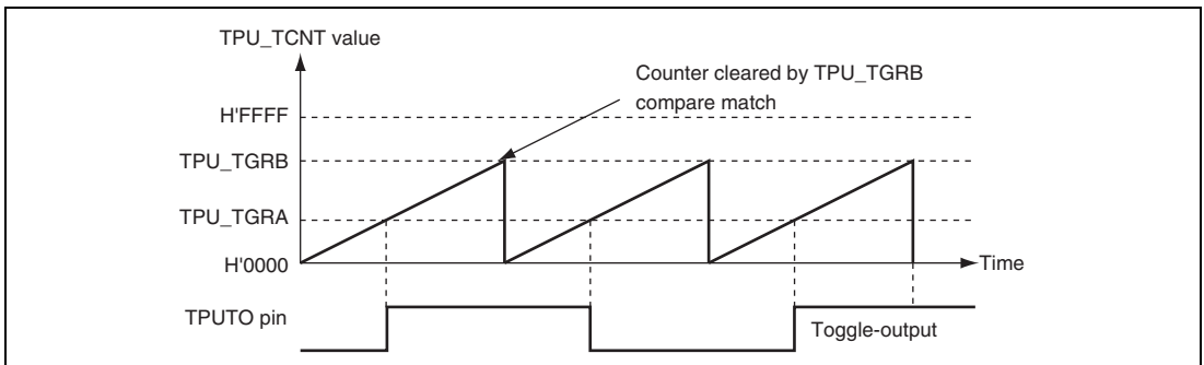
Figure 21.7 Example of Toggle Output Operation
