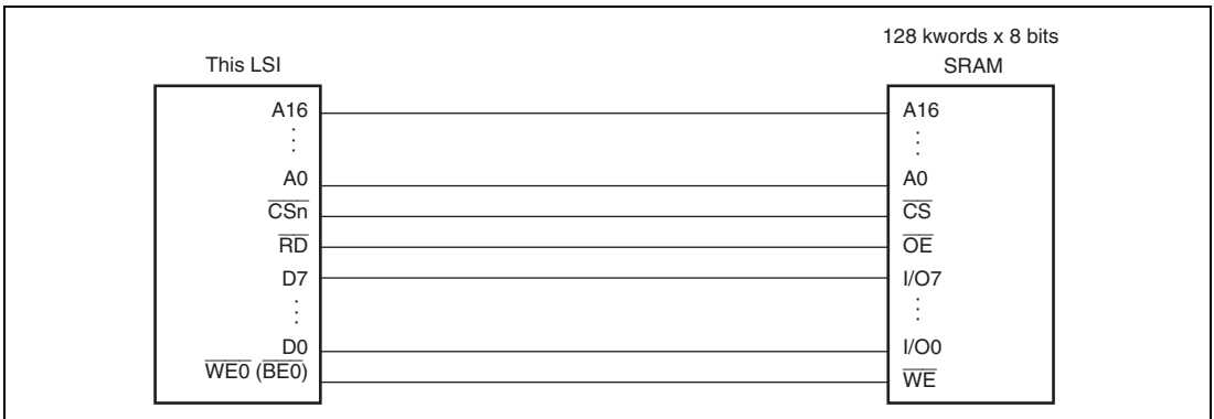
Figure 14.7 Example of 8-Bit Data-Width SRAM Connection
