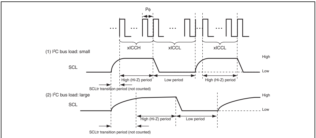
Figure 32.3 SCL Waveforms
