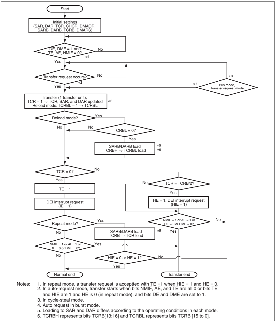
Figure 16.10 DMA Transfer Flowchart
