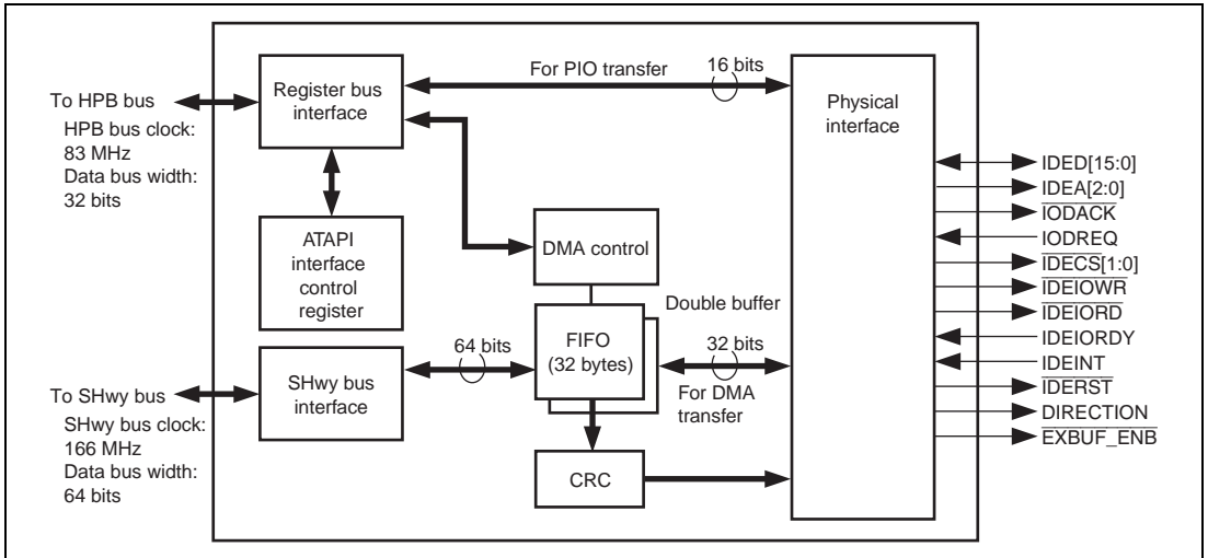
Figure 46.1 ATAPI Block Diagram
