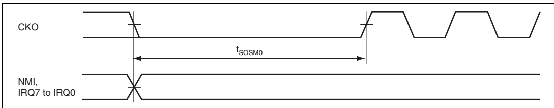
Figure 52.6 Oscillation Settling Time on Return from Software Standby by NMI or IRQ
