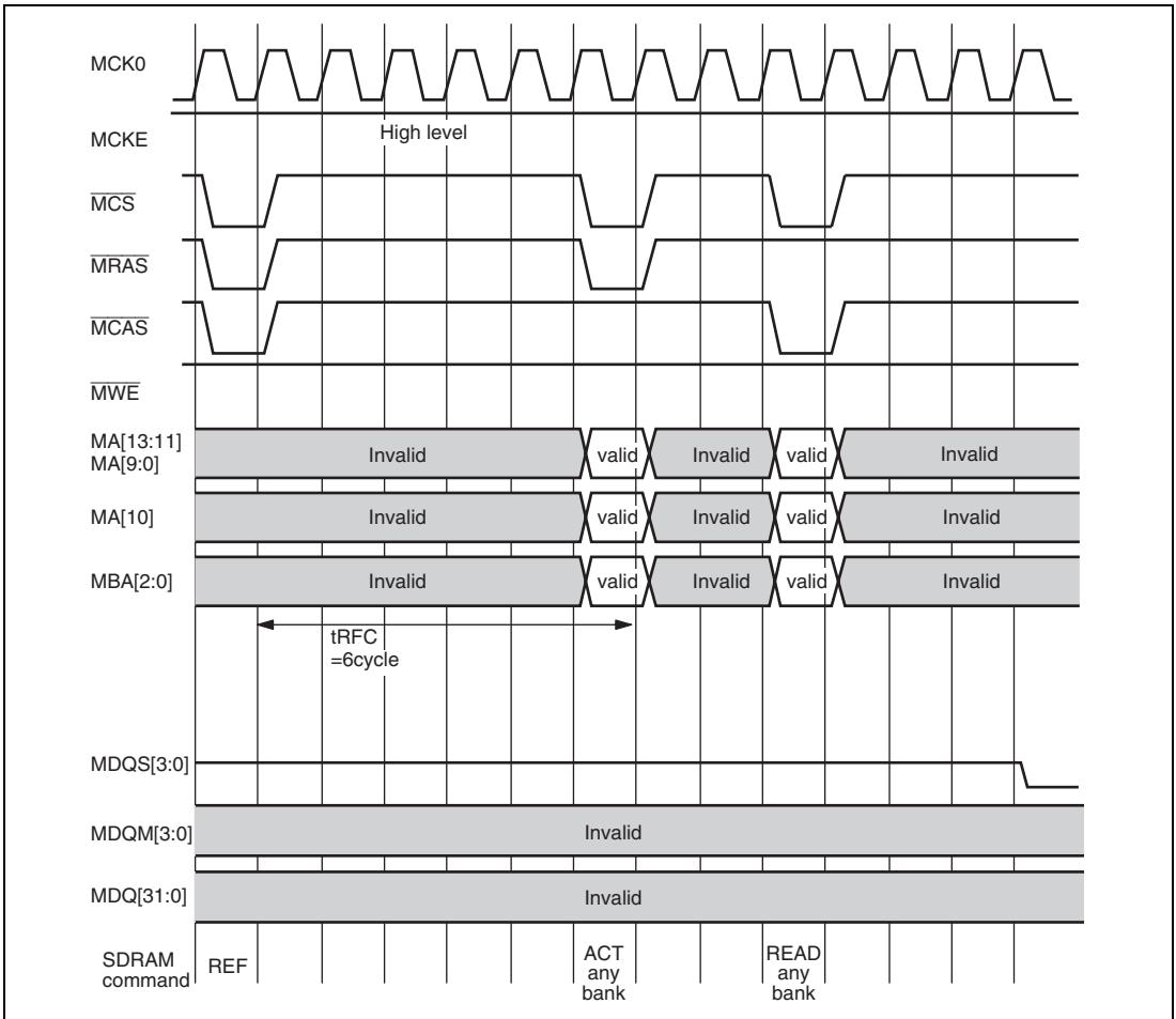
Figure 15.19 tRFC
