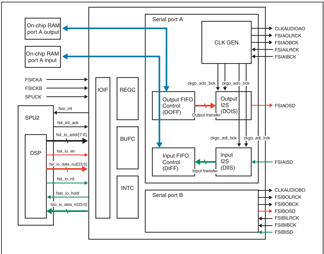
Figure 45.1 Block Diagram
