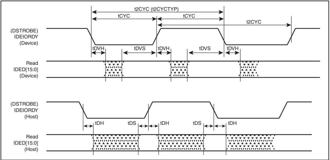
Figure 52.64 Ultra DMA Transfer Data In Burst
