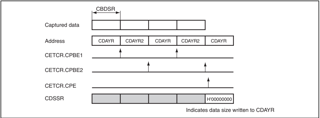
Figure 34.50 Overall Timing of CDSSR Operation in Bundle Write (When Bundle Write End and Capture End Coincide)
