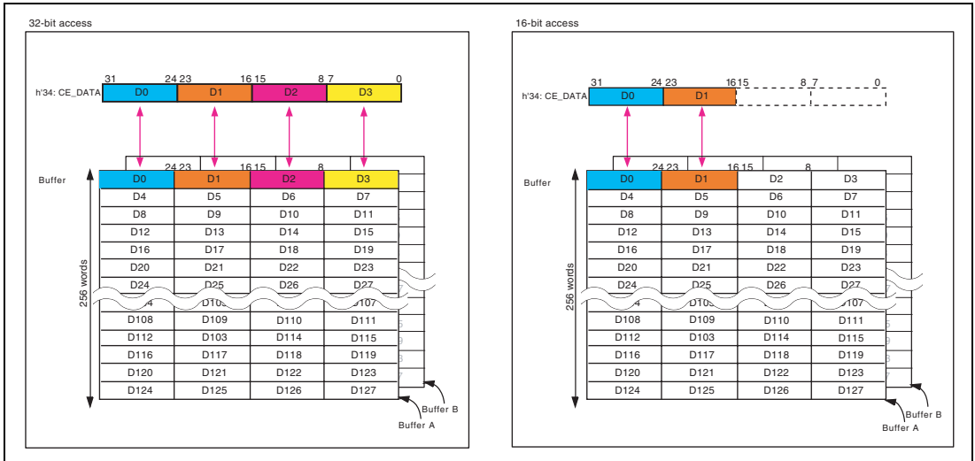
Figure 23.7 Double Buffer Structure
