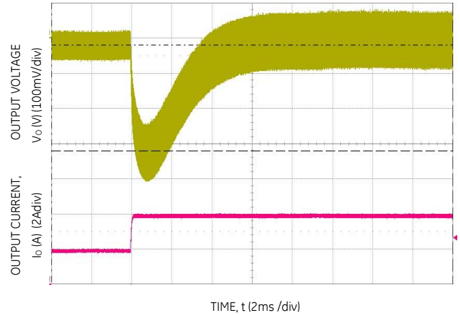
Figure 4. Transient Response to Dynamic Load Change from 50% to 100% at 12Vin, C out =3x10uF+220uF, C Tune =6800pF, R Tune =30.1kΩ
