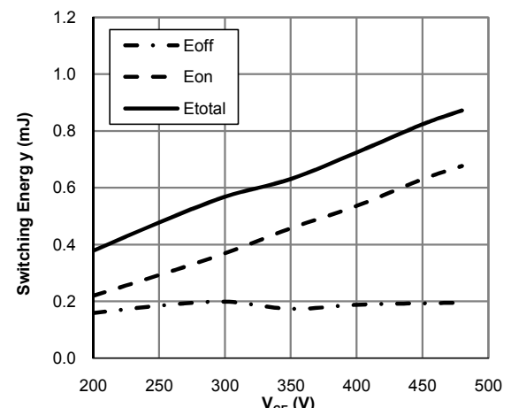
Figure 20: Switching Loss vs. V_{CE} ( T_j=150^\circ\text{C}, V_{GE}=15\text{V}, I_c=15\text{A}, R_g=20\Omega )
