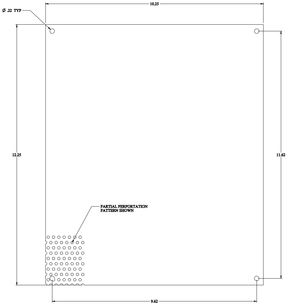
FRONT VIEW
