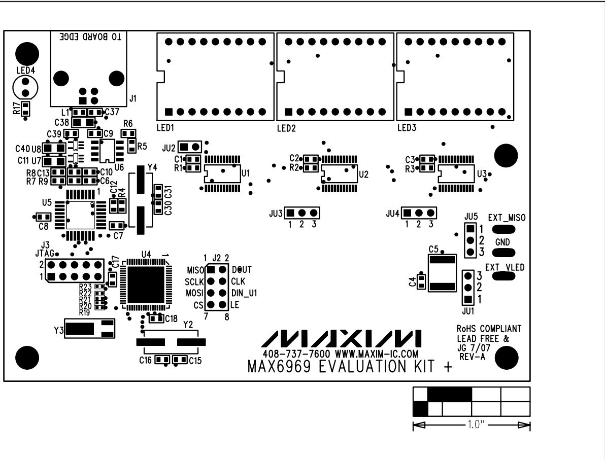
Figure 4. MAX6969 EV Kit Component Placement Guide—Component Side
