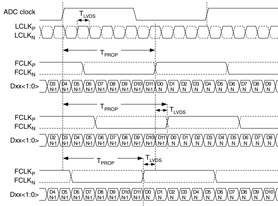
Figure 10. LVDS output timing adjustment
