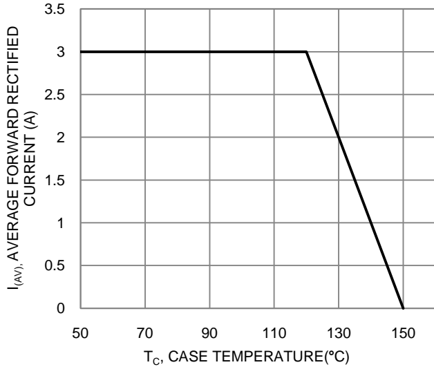
Figure 1. Output Current Derating Curve
