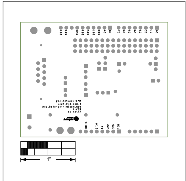
MAX13053A Shield—Bottom Silkscreen
