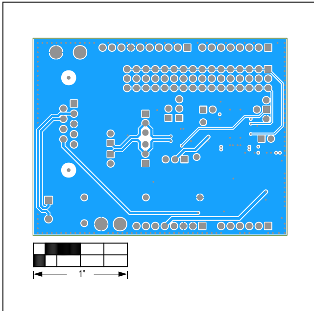
MAX13053A Shield—Bottom
