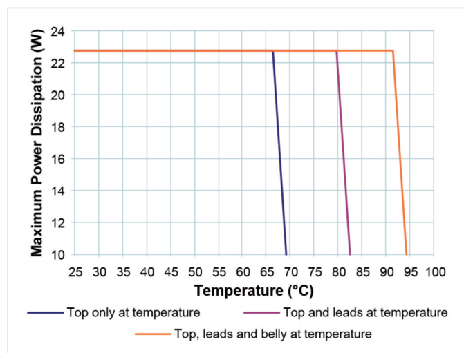
Figure 20 — Thermal Specified Operating Area: Max Power Dissipation vs. Case Temp for current limited operation
