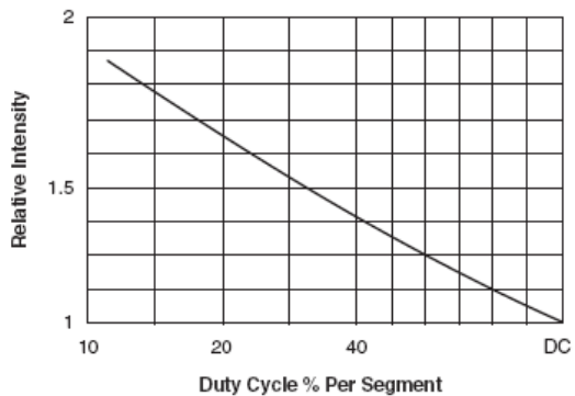
Fig. 5 Luminous Intensity vs. Duty Cycle
