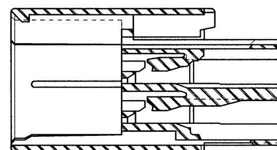
SECT. A-A
