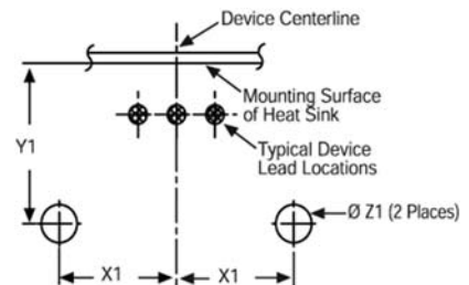
Mounting Details:
