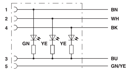
Contact assignment of M12 sockets with 3 LEDs
