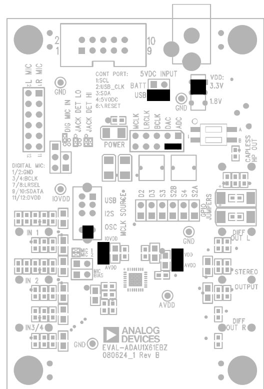
Figure 2. Evaluation Board Setup and Configuration
