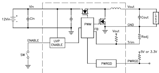
Figure 23: Block Diagram
