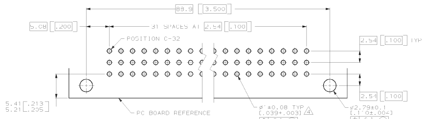
PC BOARD LAYOUT RECOMMENDED PC BOARD THICKNESS 1.57 [0.062]
