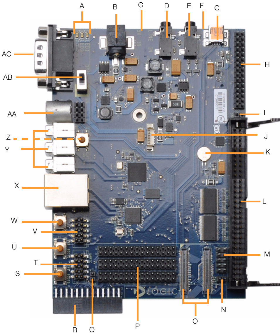
Figure 1.2 – Connection Diagram for the Baseboard
