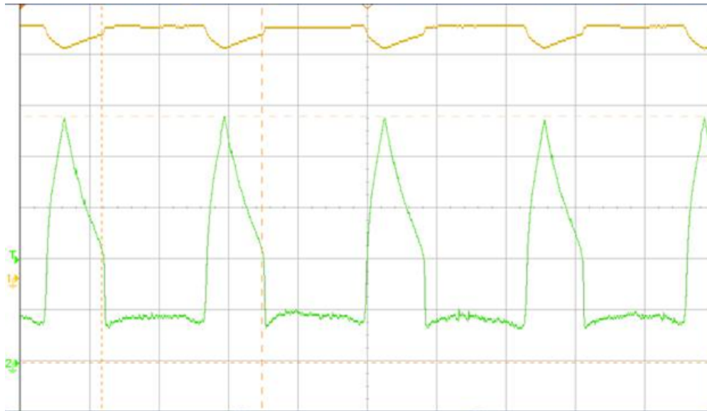
USB only GSM850 Burst Current of .965 Amps
