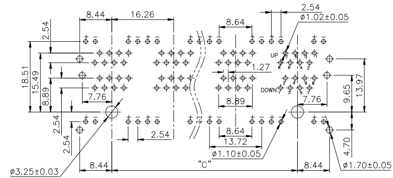
PC Board Layout example Component Side Shown
