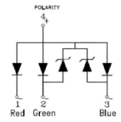
LED SCHEMATIC
