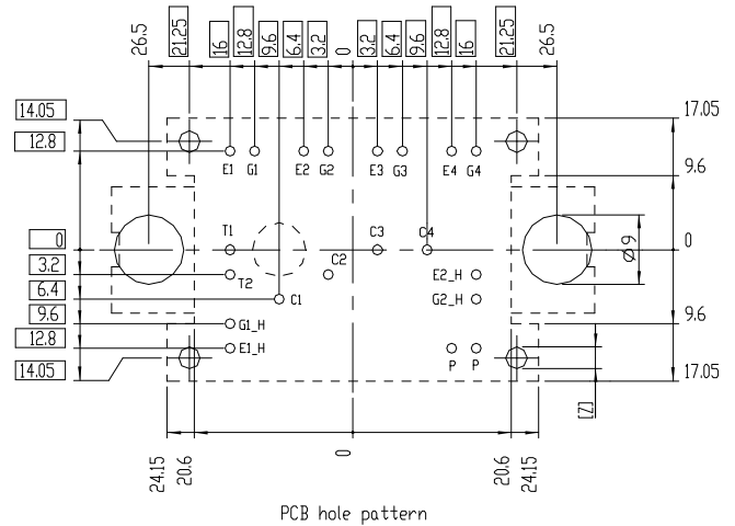
PCB hole pattern
