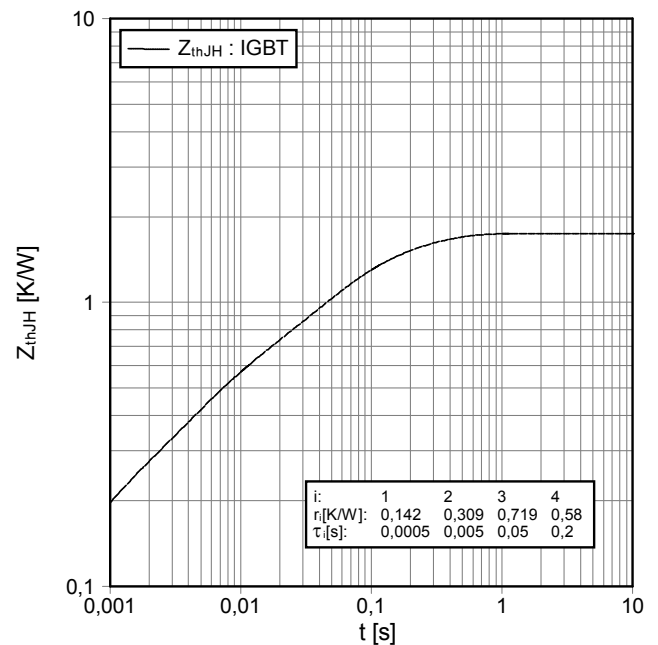
Transienter Wärmewiderstand IGBT-Wechselr. transient thermal impedance IGBT-inverter Z_{thJH} = f(t)
