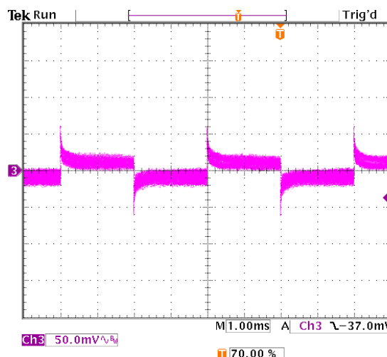
Figure 51. Transient Response with Regulation set to 3.72 mV/A.
