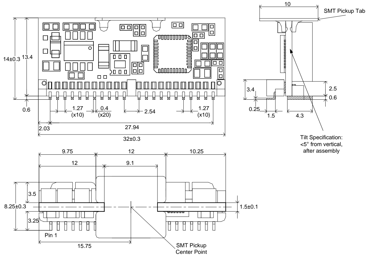
Figure 58 Mechanical Drawing
