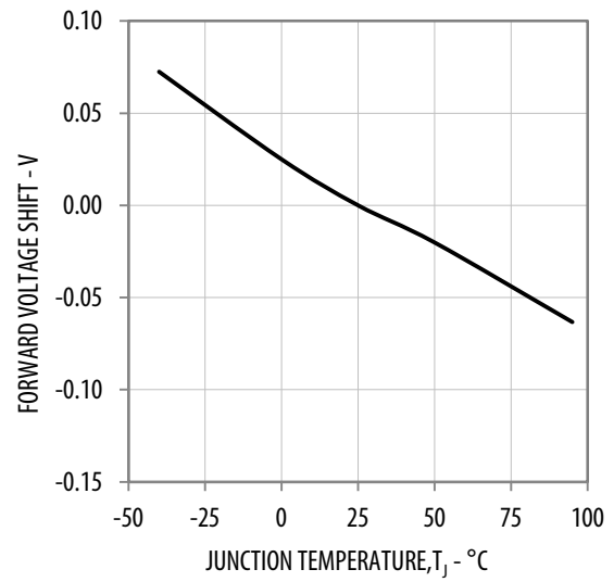
Figure 9: Forward Voltage vs. Temperature
