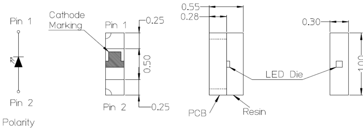
Figure 1: Package Dimensions
