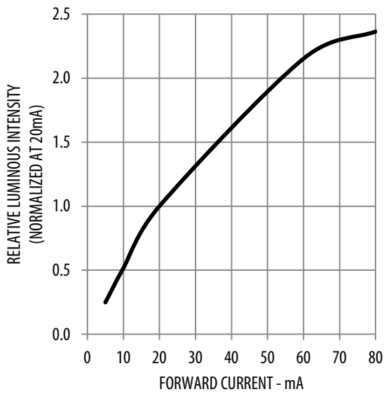
Figure 4: Intensity vs. Forward Current
