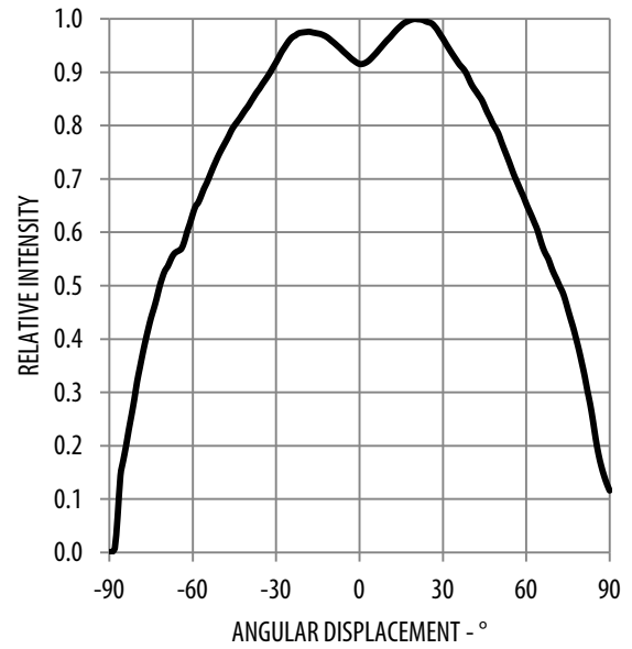
Figure 5: Intensity vs. Angle
