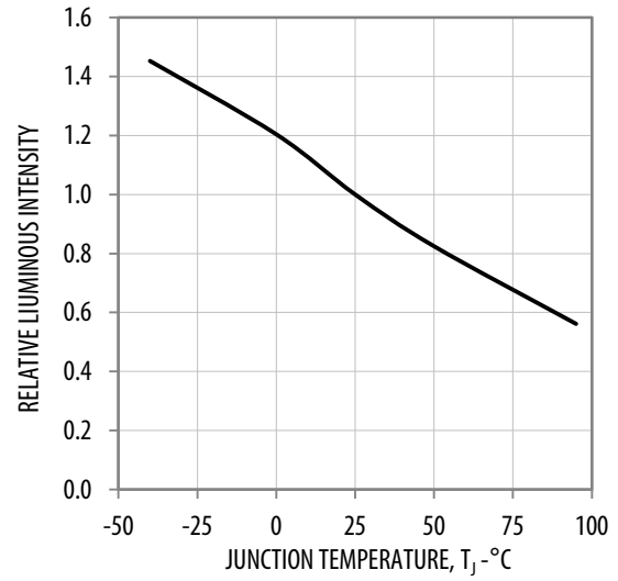
Figure 7: Intensity vs. Temperature
