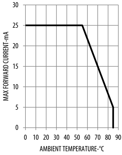
Figure 10: Forward Current vs. Temperature
