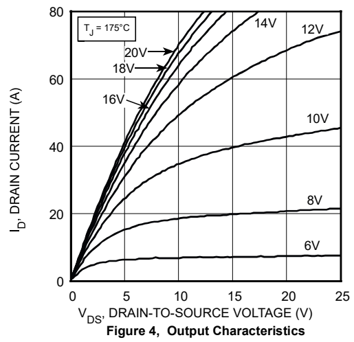
Figure 4, Output Characteristics
