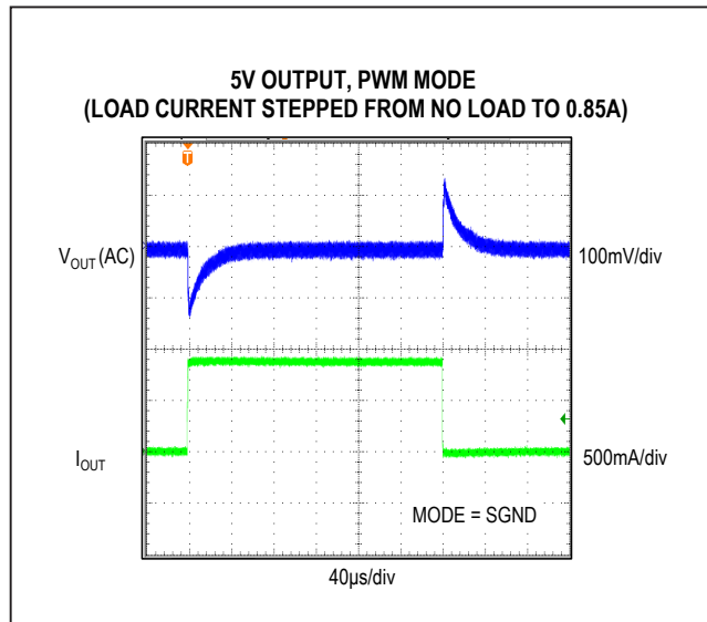
Figure 7. MAX17505 5V Output, No Load to 0.85A Load Transient (PWM Mode)
