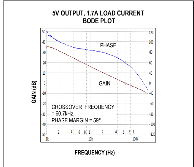
Figure 6. MAX17505 5V Output Full Load Bode Plot ( V_{IN} = 24V )
