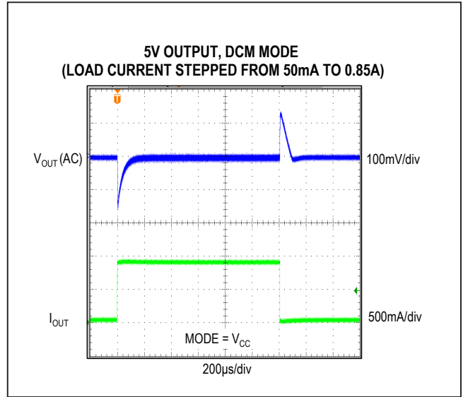
Figure 9. MAX17505 5V Output, 50mA to 0.85A Load Transient (DCM Mode)
