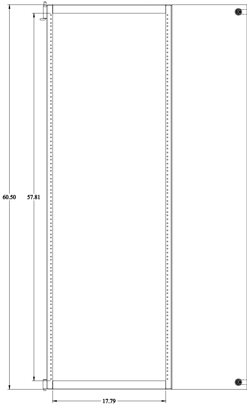
FRONT VIEW
